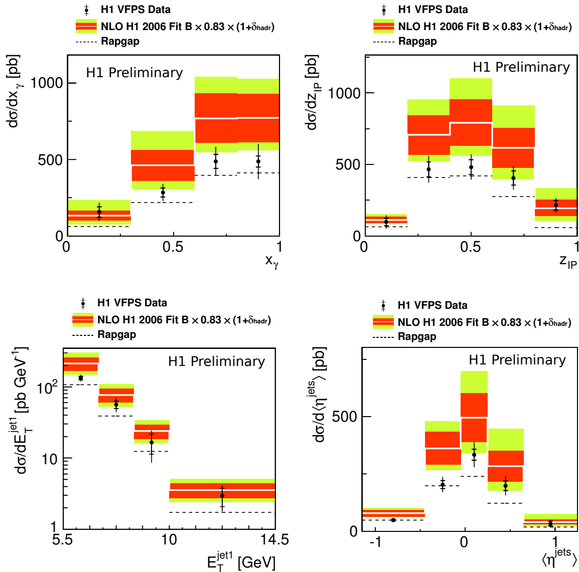
Figure 1: Differential diffractive dijet photoproduction cross sections as a function of x_\gamma , z_{IP} , E_T^{\text{jet1}} and \langle\eta^{\text{jets}}\rangle . The inner error bars represent the statistical errors. The outer error bars indicate the statistical and systematic errors added in quadrature. NLO QCD predictions based on the DPDF set H1 2006 Fit B, corrected to the level of stable hadrons, are shown as a white line. The red band indicates the DPDFs uncertainties and light green band indicates the DPDFs and scale uncertainties added in quadrature. The LO QCD predictions from RAPGAP using the same DPDF set are shown by the dashed black line.
