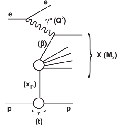
Figure 1: Diagram of the reaction ep \rightarrow eXp .
