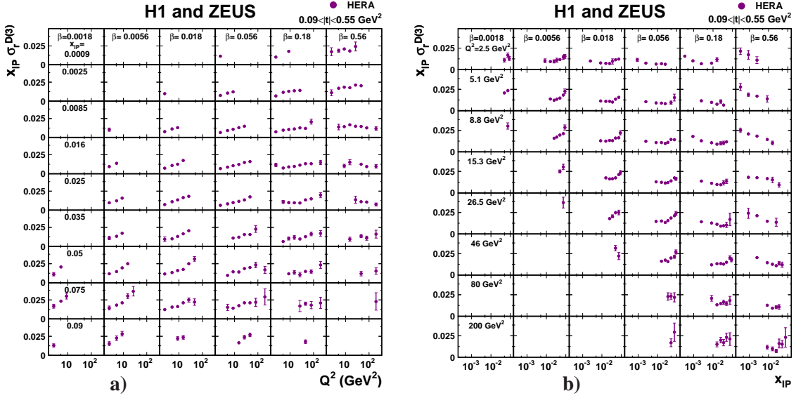
Figure 3: HERA combined reduced diffractive cross section x_P \sigma_r^{D(3)}(\beta, Q^2, x_P) for 0.09 < |t| < 0.55 \text{ GeV}^2 . as a) a function of Q^2 for different values of \beta and x_P and b) as a function of x_P for different values of \beta and Q^2 . The error bars indicate the statistical, systematic and procedural uncertainties added in quadrature. The normalisation uncertainty is included.
