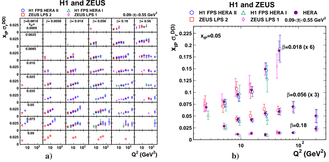
Figure 2: Reduced diffractive cross section x_{IP} \sigma_r^{D(3)}(\beta, Q^2, x_{IP}) for 0.09 < |t| < 0.55 GeV 2 as a function of Q^2 for different values of \beta and x_{IP} . In a) the H1 ‘FPS HERA II’ [6], H1 ‘FPS HERA I’ [5], ZEUS ‘LPS 2’ [2] and ZEUS ‘LPS 1’ [7] data are presented. The inner error bars indicate the statistical uncertainties, the outer error bars show the statistical and systematic uncertainties added in quadrature. Normalisation uncertainties are not included in the error bars of the individual measurements. In b) the combined data are compared to the H1 and ZEUS input data in 3 bins of \beta , at x_{IP} = 0.05 . Here the normalisation uncertainties are included in the error bars of the combined data points.
