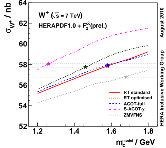
Figure 13: W^+ production cross section \sigma_{W^+} at the LHC for \sqrt{s} = 7 TeV as a function of m_c^{mod} . The lines show predictions for different VFN schemes as indicated by the legend. The stars show the predictions obtained with the optimal value of m_c^{mod} used in a given scheme. The thick dashed horizontal lines indicate the range of \sigma_{W^+} , determined for m_c^{mod} = m_c^{mod}(opt) .
