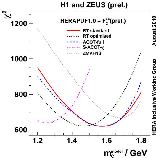
Figure 12: Comparison of the \chi^2 of HERA I + F_2^{cc} fits using different heavy flavour schemes represented as lines of different styles.
