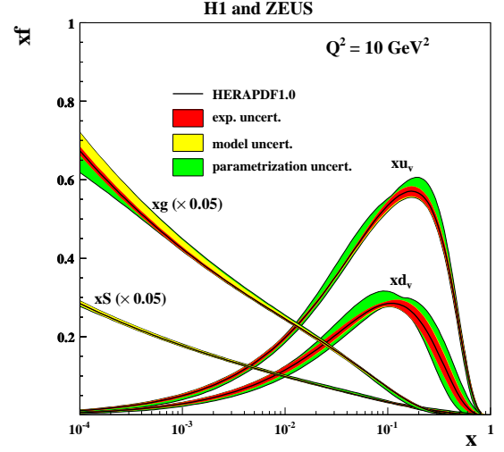
Figure 3: The parton distribution functions from HERAPDF1.0 at Q^2 = 10 GeV 2 . The gluon and sea distributions are scaled down by a factor 20. The experimental, model and parametrisation uncertainties are shown separately.
