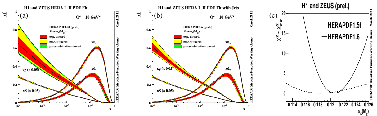
FIGURE 1. (a) HERAPDF1.5f without and (b) HERAPDF1.6 with jet data included in the fit, as a function of x for Q^2 = 10 GeV 2 with \alpha_s(M_Z) as an additional free parameter in the fit, and (c) \Delta\chi^2 for both fits.
