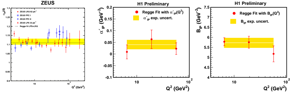
Figure 3: Measurement of the \alpha_P(0) (left), \alpha'_P(0) (middle) and B_P as a function of Q^2
