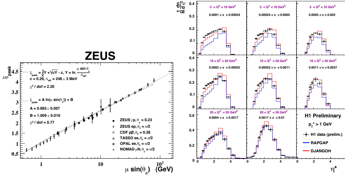
Figure 1: Left: The \xi peak as a function of \mu \sin(\theta_c) , \mu is the characteristic energy scale. The ZEUS \gamma p data (solid circles) and ep data (diamonds) and results from OPAL (crosses), TASSO (triangles), NOMAD (stars) and CDF (open circles) collaborations are shown. Right: Measured \eta^* for charged particles for the hadronic centre of mass system for p_t^* > 1 GeV. Data are compared to RAPGAP and DJANGO Monte Carlo predictions.
