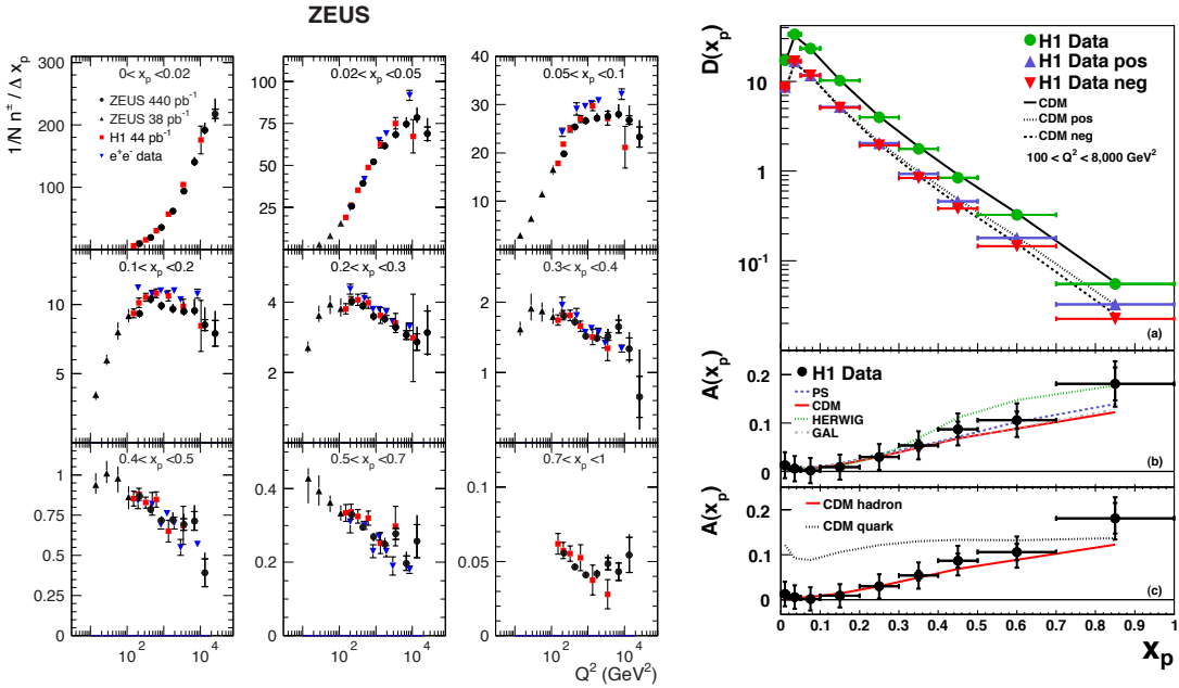
Figure 2: Left: The measured normalised distributions of the scaled momentum, 1/Nn_{\pm}/\Delta x_p , as a function of Q and x_p . The dots (triangles) represent the new (previous) ZEUS measurement, the squares the H1 data and the inverted triangles the e^+e^- data. Right: (a) The measured normalised distributions of the scaled momentum, D(x_p) , for all charged particles and for positively (pos) and negatively (neg) charged particles separately, and (b), (c) the charge asymmetry, as a function of x_p , compared to Monte Carlo predictions.
