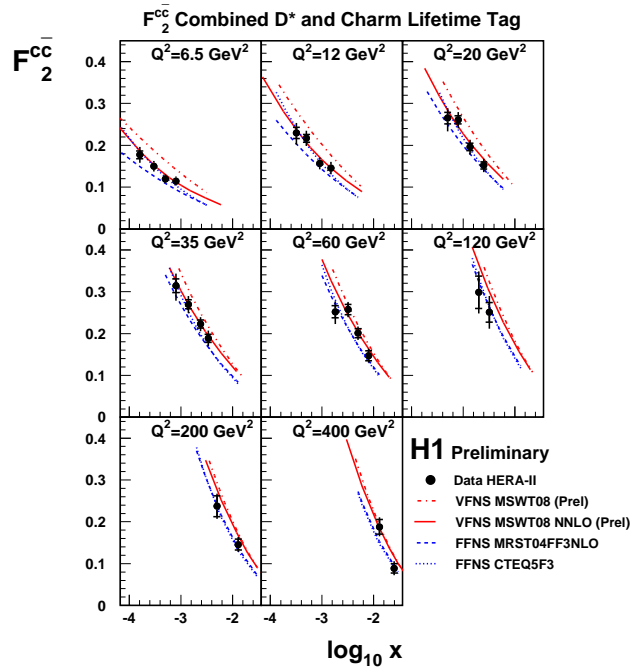
Figure 5: The H1 combined F_2^{c\bar{c}} is compared to different NLO QCD calculations.
