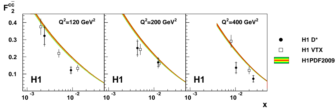
Figure 4: Charm contribution to the proton structure from D^* cross sections together with the H1 results using lifetime information. Data are compared to the H1 PDF fit H1PDF2009.
