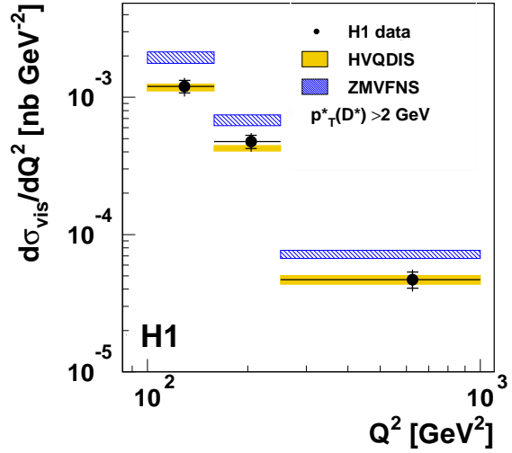
Figure 3: D^* cross section at high Q^2 compared to the massive (HVQDIS) and massless (ZM-VFNS) NLO QCD calculation.
