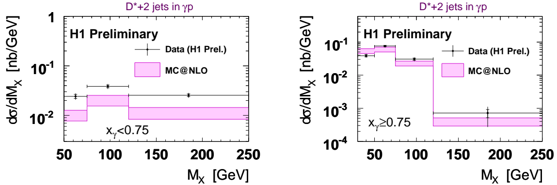
Figure 1: D^* + 2 jet cross section as a function of the invariant mass of the proton and photon side M_X for low x_\gamma < 0.75 (a) and high x_\gamma > 0.75 (b). The data are compared to the prediction by MC@NLO [3] using the CTEQ66 proton PDF [4].
