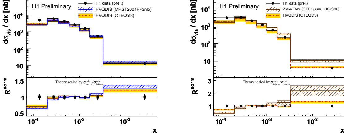
Figure 2: D^* cross section as a function of x (a) compared to the NLO QCD calculation (HVQDIS) using two different proton PDFs: MRST2004FF3nlo [7] or CTEQ5f3 [8]. (b) shows the D^* data for p_T^* > 2 \text{ GeV} compared to the massless (ZM-VFNS) and massive NLO QCD calculation.
