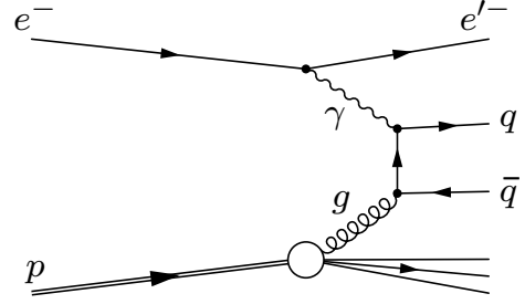
Figure 1: A Feynman diagram of the boson gluon fusion process.
