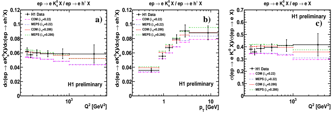
Figure 4: The measured ratios of the K_S^0 over charged particles ( h^\pm ) as function of a) four-momentum of the transfer photon Q^2 and b) the transverse momentum p_T of the K_S^0 . c) The density distribution K_S^0/\text{DIS} as function of Q^2 .
