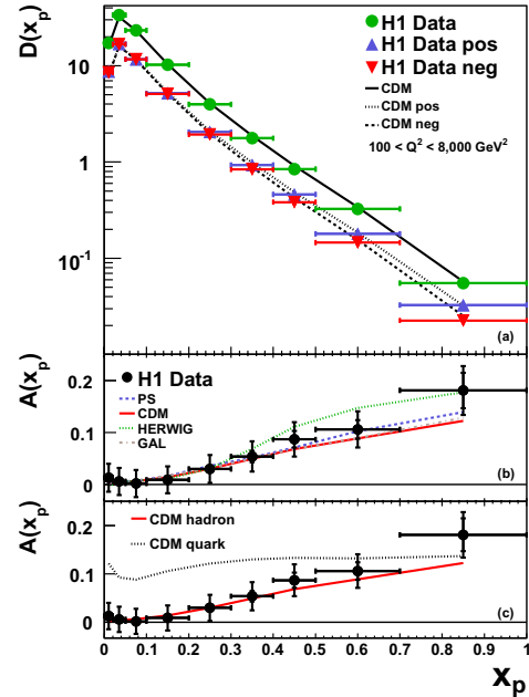
Figure 3. The measured normalized distributions of the scaled momenta for all charged particles and for positively (pos) and negatively (neg) charged particles (a), and the charge asymmetry as a function of x_p (b,c). The data are compared to predictions from different Monte Carlo models.
