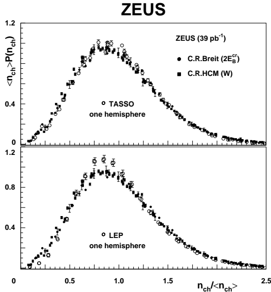
Figure 1: Comparison of multiplicity distributions in KNO form in bins of 2 \cdot E_B^{cr} and W (solid markers) with e^+e^- data for one hemisphere (open circles).
