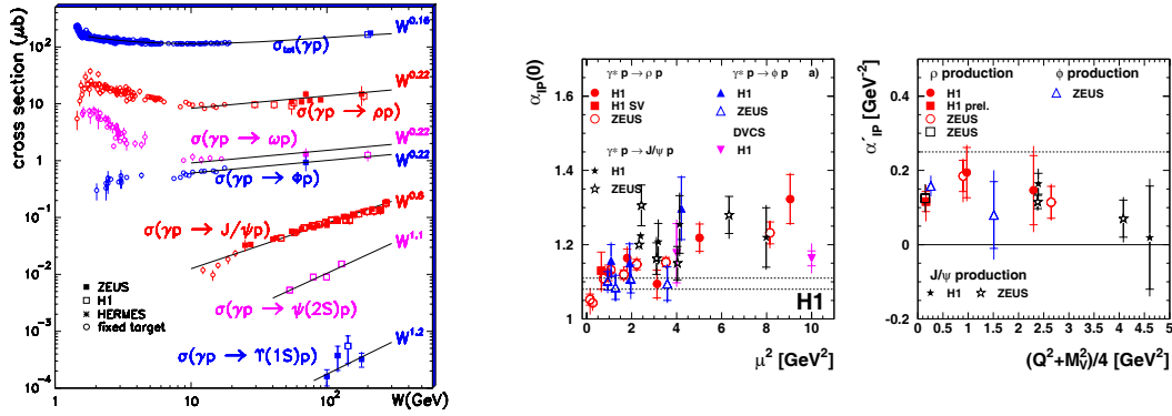
Figure 4: (left) W dependence of VM photoproduction [22]; measurement of the intercept \alpha_{\mathbb{P}}(0) (centre) and of the slope \alpha' (right) of the effective Regge trajectory, as a function of the scale \mu^2 = (Q^2 + M_V^2)/4 for VM production and \mu^2 = Q^2 for DVCS [7].
