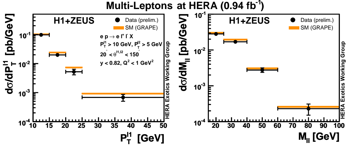
FIGURE 2. The measured cross section of lepton pair production in a phase space dominated by photon-photon processes as a function of the leading lepton transverse momentum P_T^{\ell 1} (left) and the invariant mass of the lepton pair M_{\ell\ell} (right).
