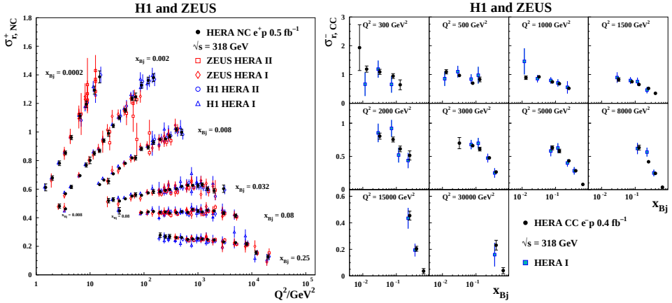
Fig. 1. Left: some of the selected H1 and ZEUS individual NC e^+p cross section measurements in HERA I and II in comparison with the corresponding combined data. Right: the combined CC e^-p cross sections from HERA I in comparison with the full combination.
