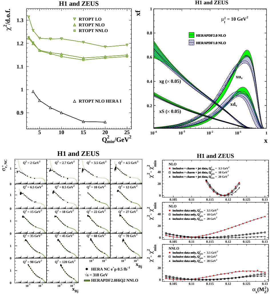
Fig. 2. Top left: the dependence of \chi^2 per degree of freedom (d.o.f.) on Q_{\min}^2 of LO, NLO and NNLO fits to the combined data. Top right: comparison of NLO PDFs xu_v , xd_v , xS = 2x(\bar{U} + \bar{D}) and xg between HERAPDF 2.0 and 1.0. Bottom left: the combined low- Q^2 NC e^+p cross section data in comparison with predictions from high Q^2 version of NNLO HERAPDF 2.0. Dotted lines indicate extrapolation into kinematic regions not included in the fit. Bottom right: \chi^2 - \chi_{\min}^2 versus \alpha_s(M_Z^2) for fits with different Q_{\min}^2 using (upper part) inclusive charm and jet production at NLO, (middle part) inclusive ep scattering data only at NLO and (lower part) inclusive ep scattering data only at NNLO.
