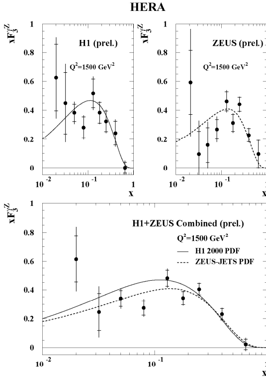
Figure 1: Measurements of the structure function x F_3^{\gamma Z} by the H1 collaboration (top left), the ZEUS collaboration (top right) and combined (bottom). The curves describe the Standard Model predictions as obtained in NLO QCD fits to the H1 inclusive data and to the inclusive and jet ZEUS data, respectively.
