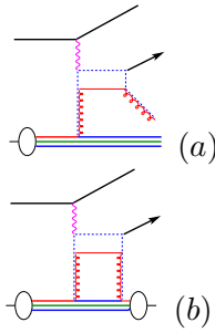
Fig. 1. Schematic picture of inelastic (a) and elastic (b) vector meson lepto-production
