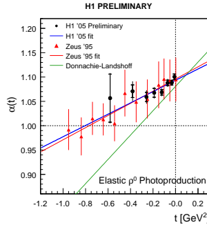
Fig. 7. \alpha_P(t) measured in elastic \rho^0 photoproduction.
