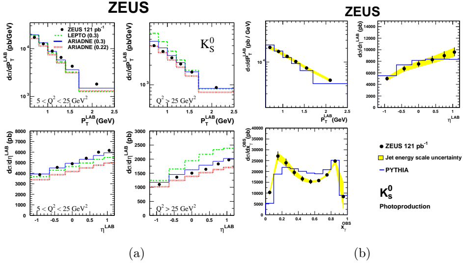
Fig. 1. Differential K_S^0 cross-sections for (a) low and high Q^2 DIS and (b) \gamma p .
