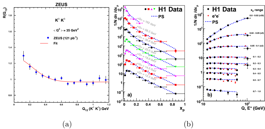
Fig. 2. (a) Bose–Einstein correlation function of K^\pm K^\pm pairs. (b) The measured normalised distribution of the scaled momentum compared with the PS Monte Carlo.
