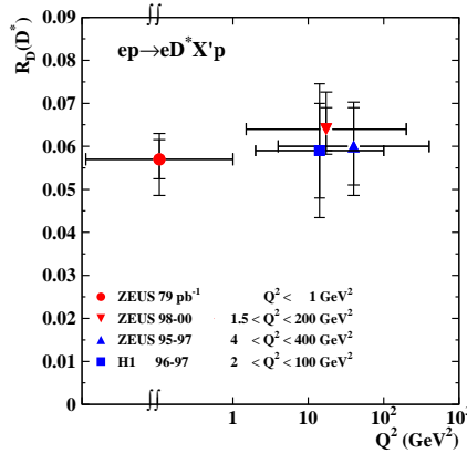
Figure 2: Fractions \mathcal{R}_D of D^* meson diffractive production cross sections measured at HERA in DIS [3, 13, 12] and photoproduction [2]. The inner bars show the statistical errors, the outer bars correspond to the statistical and systematic uncertainties added in quadrature.
