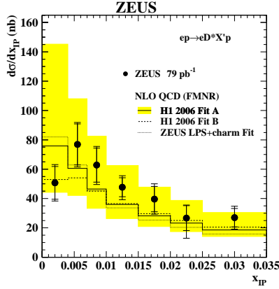
Figure 1: Differential cross section (dots) for diffractive photoproduction of D^* , measured as function of x_P . The inner bars show the statistical errors; the outer bars correspond to the statistical and systematic uncertainties added in quadrature. The data are compared to the NLO QCD calculations (histograms). The shaded bands show the uncertainties coming from variations of the charm-quark mass and the factorisation and renormalisation scales.
