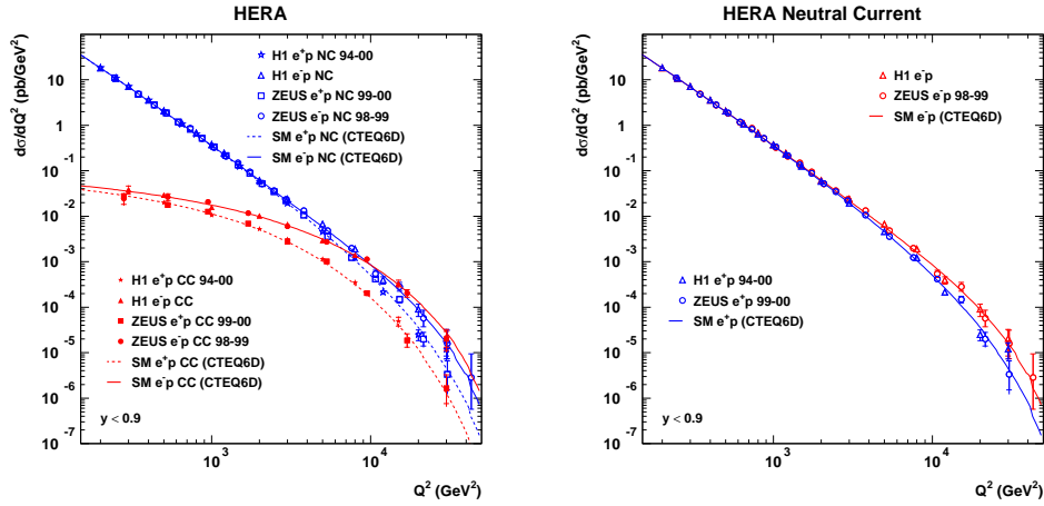
FIGURE 1. Differential cross sections of unpolarized NC and CC scattering as a function of Q^2 for NC and CC (left) and for e^\pm p NC (right).
