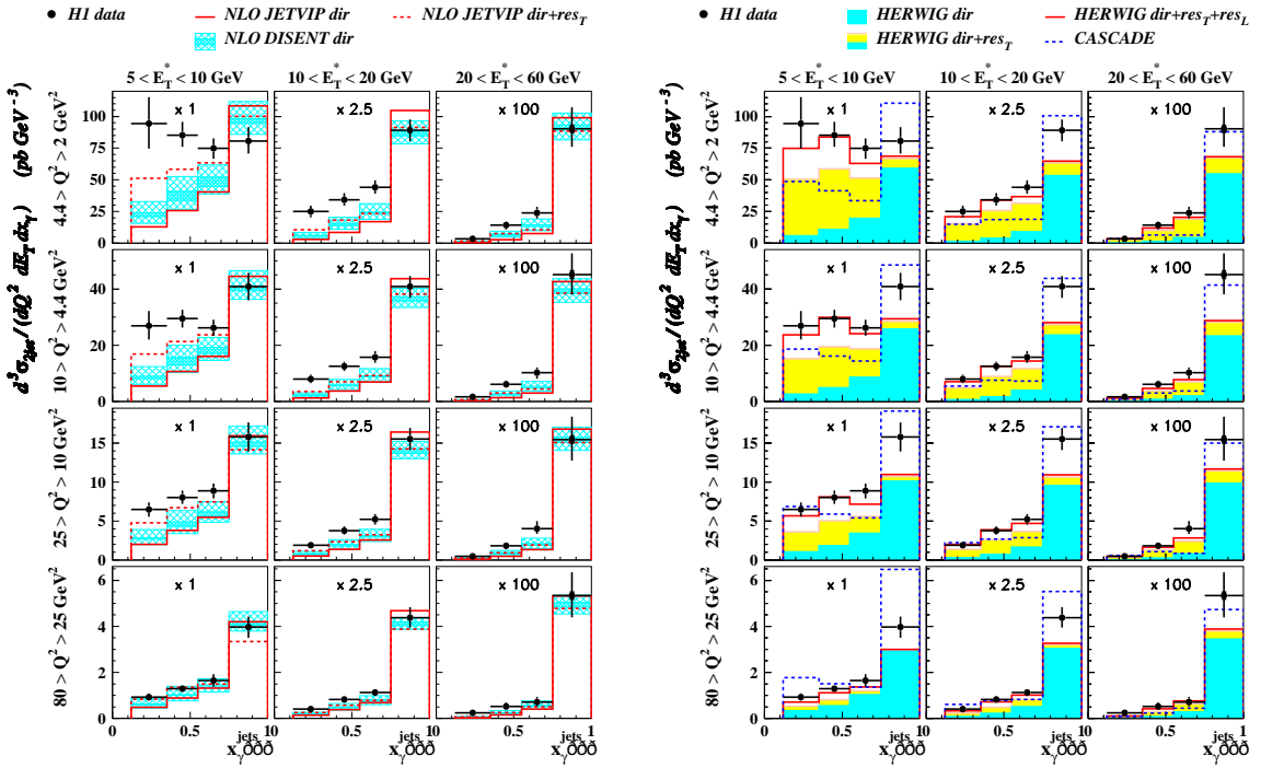
Figure 2: Triple differential cross section d^3 \sigma_{\text{jet}}/dQ^2 dE_T^* dx_\gamma^{\text{jets}} compared to NLO predictions from JETVIP and DISENT (left) and to calculations from the LO program HERWIG and from CASCADE (right).
