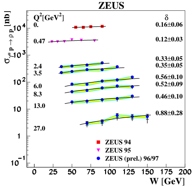
Figure 9. W dependence of the cross section \sigma(\gamma^* p \rightarrow \rho^0 p) for various Q^2 values. The data for Q^2 < 1 \text{ GeV}^2 obtained previously [35] are also shown. The solid lines show a fit with \sigma_{\gamma^* p \rightarrow \rho^0 p} \sim W^\delta . The shaded area indicates normalization uncertainties due to proton dissociation background. From [36].
