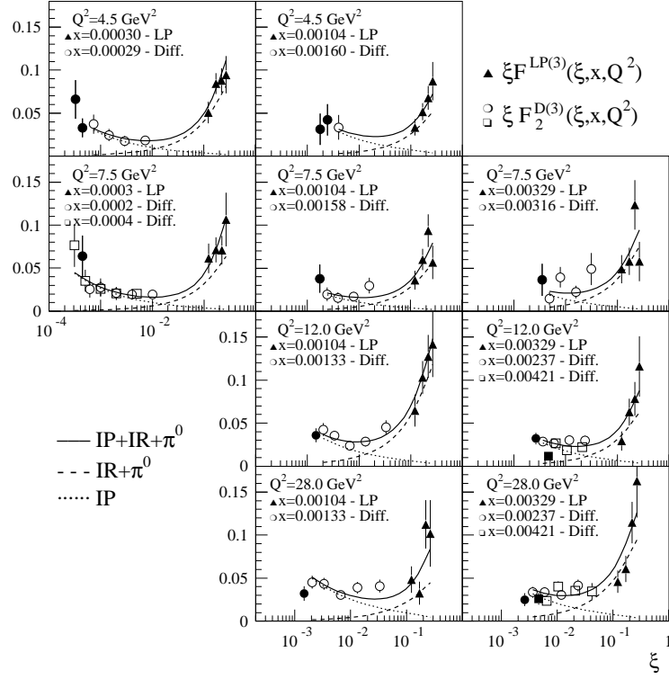
Figure 20. Diffractive (Diff, open circles and open squares) and leading proton (LP, black triangles) structure function data vs. \xi , for fixed x and Q^2 . The figure combines, in each plot, the diffractive and leading proton H1 data with similar values of x and Q^2 . The quoted Q^2 values are those of the diffractive data; the corresponding Leading Proton values are Q^2 = 4.4, 7.5, 13.3 and 28.6 \text{ GeV}^2 . The black circles and black squares are data with M_X < 2 \text{ GeV} . The plotted curves represent a global fit: total (solid line), pomeron (dotted line) and reggeon plus pion contributions (dashed line). For details and references see [45].
