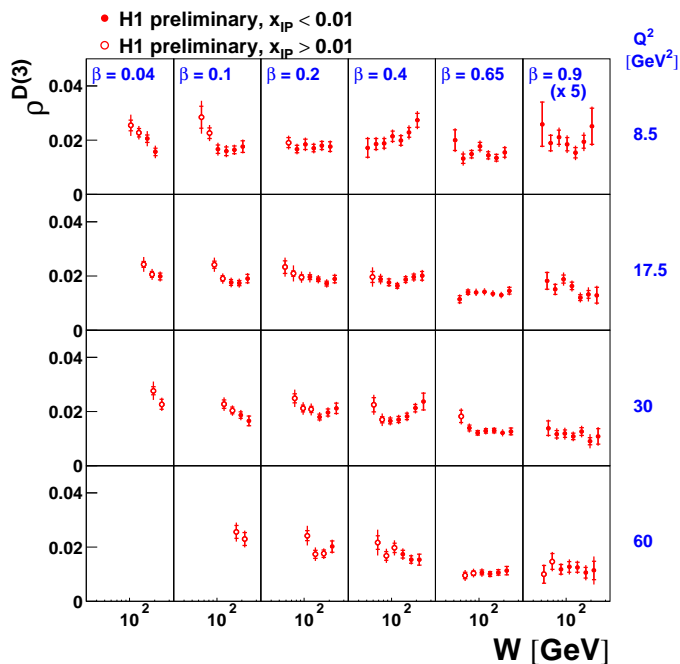
Figure 17. Recent H1 measurements of \rho^{D(3)} , the ratio of the diffractive to the inclusive cross section versus W . Data at \beta = 0.9 are scaled by a factor of five [15].
