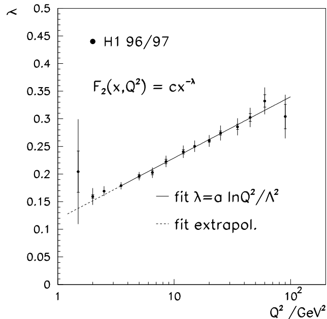
Figure 7. The exponent \lambda_{tot} in \sigma_{tot}^{\gamma^*p} \sim (W^2)^{\lambda_{tot}} , versus Q^2 . The full line shows a fit to the form indicated with a = 0.0481 \pm 0.0013(\text{stat}) \pm 0.0037(\text{syst}) and \Lambda = 292 \pm 20(\text{stat}) \pm 51(\text{syst}) MeV. Extrapolation to Q^2 = 0.48 GeV 2 gives a value of 0.08[31].
