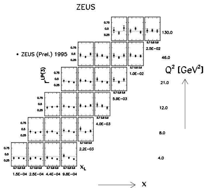
Figure 19. The fraction of leading protons, measured with the ZEUS Leading Proton Spectrometer, as a function of x_L = 1 - \xi in bins of x and Q^2 . From [57].
