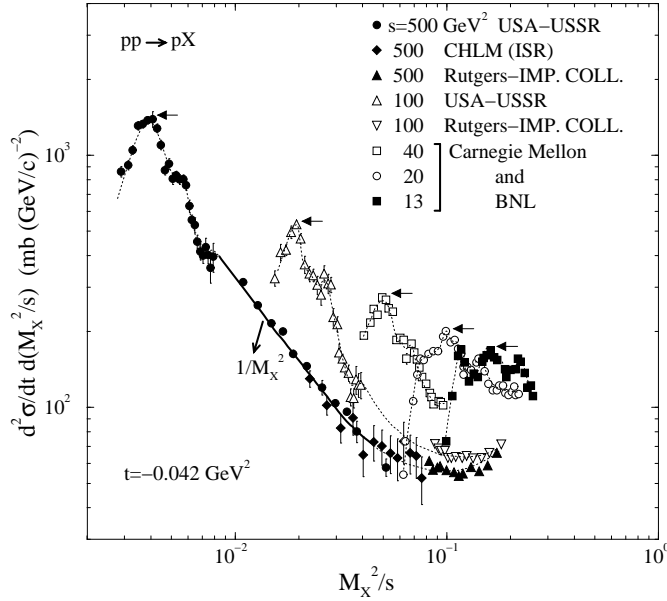
Figure 13. Single diffractive pp cross sections [43]). The figure shows how the characteristic 1/M_X^2 (Regge) behavior of diffraction becomes manifest as s increases. The arrows indicate the low mass ( M_X \approx 2 GeV) resonance region. From [45].
