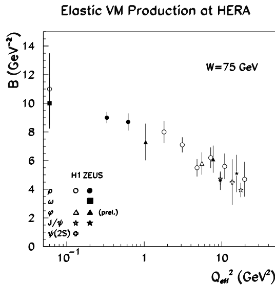
Figure 10. Slope parameter B(s) as a function of Q_{eff}^2 ; Q_{eff}^2 = Q^2 for \rho and \omega , Q_{eff}^2 = Q^2 + M_\phi^2 for \phi , Q_{eff}^2 = Q^2 + M_{J/\psi}^2 for J/\Psi . From [30].
