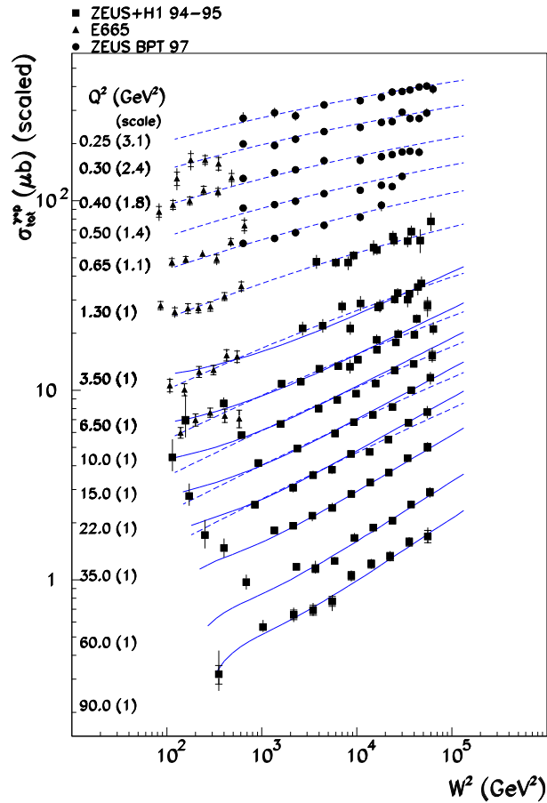
Figure 6. \gamma^*p cross section as a function of W^2 at various Q^2 , shown on the left side together with the scale factor applied to the data for better visibility. The full lines show a QCD-fit [28], the dashed lines are a fit by the Golec-Biernat Wüsthoff saturation model [29]. From [30].
