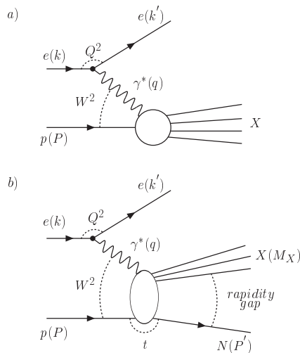
Figure 1. Kinematic variables (a) for the reaction e p \rightarrow e X ; (b) for the semi-inclusive reaction e p \rightarrow e N X with a rapidity gap.
