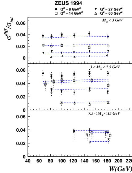
Figure 16. Ratio of diffractive and total cross sections at fixed values of Q^2 , for different regions of the invariant diffractive mass M_X . The lines are predictions of the saturation model [29].
