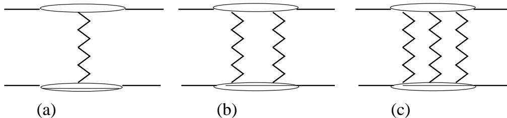
Figure 4. Hadron-hadron scattering via pomeron exchange: (a) one-Pomeron, (b) two-Pomeron, and (c) three-Pomeron exchange graphs. From [24].
