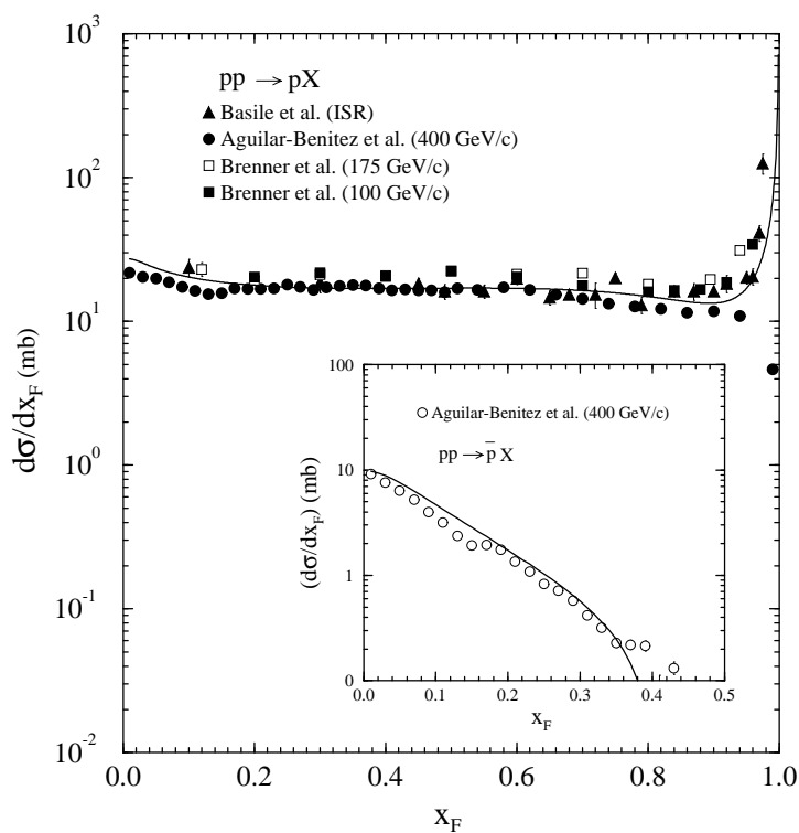
Figure 18. Inclusive spectrum for the reactions pp \rightarrow pX and pp \rightarrow \bar{p}X (insert). From [56].
