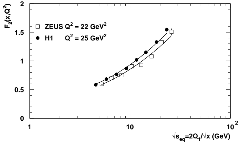
Figure 22. Comparison of e^+e^- data on average charged particle multiplicities versus \sqrt{s} and the HERA low- x F_2 data versus 2Q_1/\sqrt{x} , with Q_1 = 270 MeV, for Q^2 = 22 GeV ^2 (ZEUS) and 25 GeV ^2 (H1). The e^+e^- multiplicity data (solid lines) are represented by curves resulting from a phenomenological fit of a second-order polynomial in \ln s to e^+e^- data. They are normalized to the F_2 data for each Q^2 bin separately. From [81].
