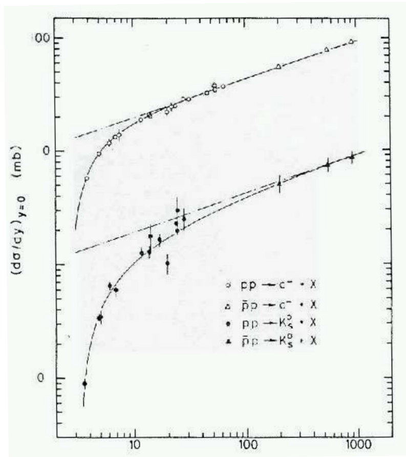
Figure 5. Cross sections of negatively charged particles and K_S^0 in the reactions pp \rightarrow c^- + X , p\bar{p} \rightarrow c^- + X , pp \rightarrow K_S^0 + X and p\bar{p} \rightarrow K_S^0 + X in the central centre-of-mass rapidity region, (d\sigma/dy)_{y=0} . c^- stands for a negatively charged hadron. The solid curves are fits with the double-Regge expression (23) with a super-critical Pomeron: as^\Delta + bs^{(2\Delta-1)/4} + cs^{-1/2} yielding \Delta \simeq 0.17 for all reactions. The dashed lines represent the s^\Delta term. For references to data see [25].
