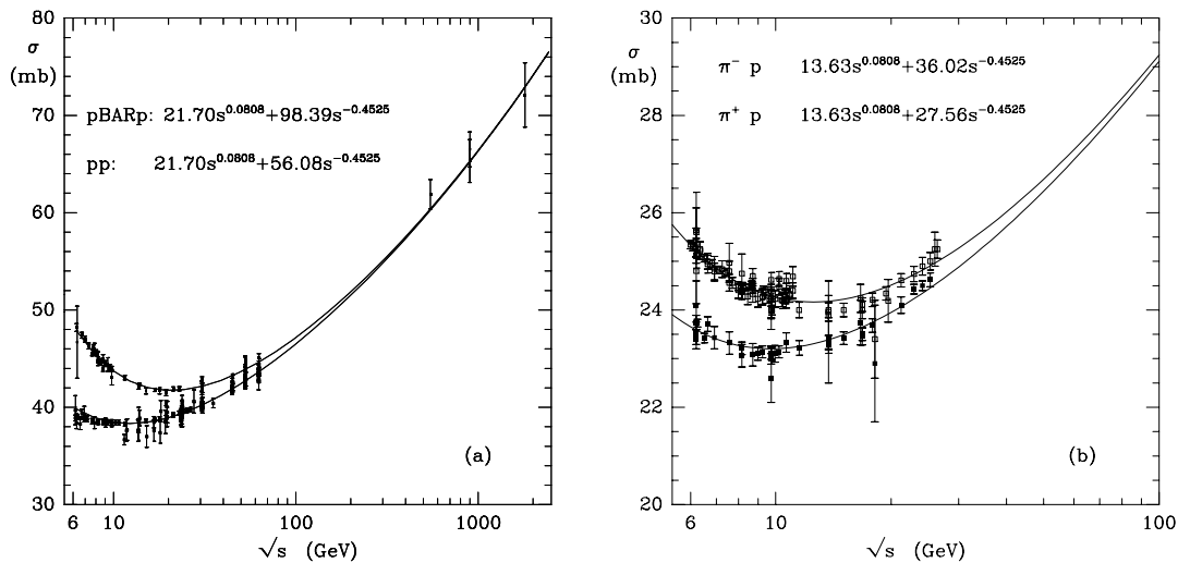
Figure 3. Total cross sections measured in hadronic scattering as a function of the centre-of-mass energy for pp , p\bar{p} , \pi^\pm p scattering. The cross sections show a “universal” rise at high energies of the form \sigma \sim s^{0.08} [16].
