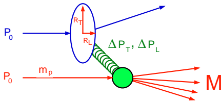
Figure 11. Single diffractive dissociation. The invariant mass of the produced hadrons, M , is denoted by M_X in the main text. From [44].
