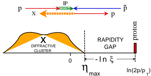
Figure 12. Topology for p\bar{p} \rightarrow pX [44].
