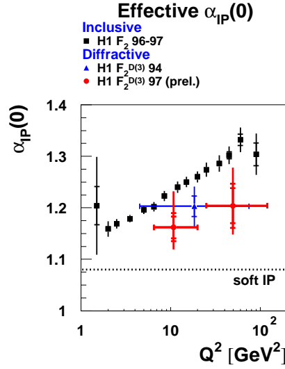
Figure 15. H1: effective value of \alpha_P(0) as function of Q^2 : \bullet extracted from F_2^{D(3)} ; \blacksquare from a fit of F_2(x, Q^2) to the form x^{-\lambda(Q^2)} ; \blacktriangle H1 1994 data [54]. From [15].
