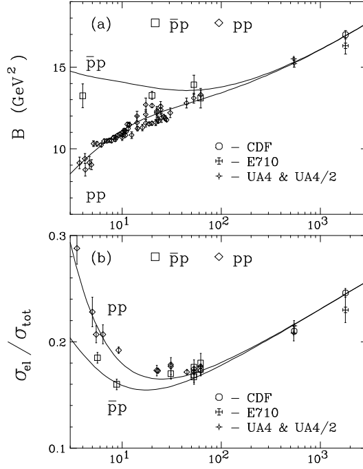
Figure 8. (a) slope parameter B(s) , (b) ratio of elastic to total cross section versus \sqrt{s} for \bar{p}p/pp interactions. The solid lines are Regge fits. For details see [21].
