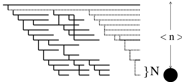
Figure 21. A high energy interaction in the parton model. From [68].
