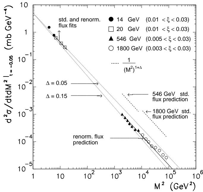
Figure 14. Cross sections d^2\sigma_{sd}/dM_X^2 dt for p + p(\bar{p}) \rightarrow p(\bar{p}) + X at t = -0.05 GeV 2 and \sqrt{s} = 14, 20, 546 and 1800 GeV. For a description of the curves see [13].
