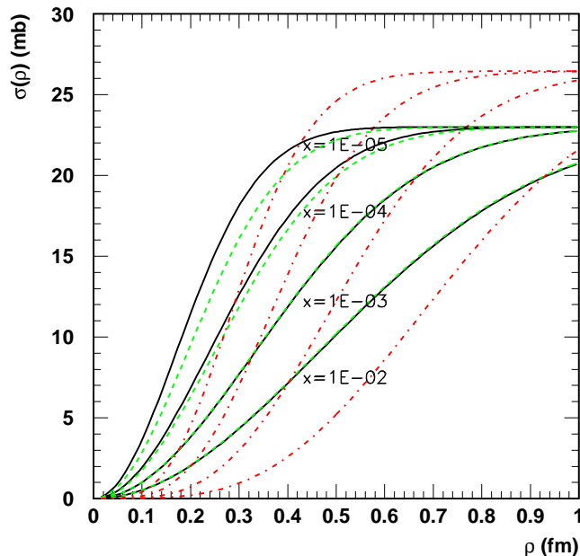
Figure 25. The dipole cross section \sigma(\varrho) for various values of Bjorken- x . The GBW parameterisation, Eqs. 60 and 61, with \lambda = 0.29 is shown as the solid curve. The dashed lines correspond to the 1/x dependence given by Eq. 62 with parameters n_f = 3 , K = 0.288 , \Lambda = 1.03 GeV, taken from [90]. The dot-dashed lines show 0.05 \times \sigma^2(\varrho) .
