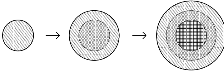
Figure 2. Qualitative picture of the high-energy evolution of a hadronic target in impact parameter space. From [4].
