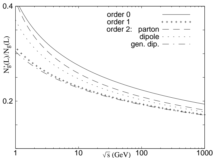
Figure 26. Anomalous multiplicity dimension to different orders in \sqrt{\bar{\alpha}} . The chosen example is N_f = 4 and \Lambda = 0.22 GeV. Anomalous dimension N'_g/N_g as \bar{\alpha} = 3\alpha_s/2\pi (solid line), \sqrt{\bar{\alpha}}(1-2a_1\sqrt{\bar{\alpha}}) (crossed) and \sqrt{\bar{\alpha}}(1-2a_1\sqrt{\bar{\alpha}}-4a_2\bar{\alpha}) for the parton equation (dashed), dipole equation (dotted) and generalized dipole equation (dash-dotted). The constants are a_1 = 0.297 , a_2 = -0.339 . For a detailed discussion see [94].
