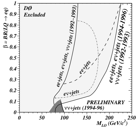
Figure 2. The 95% CL lower limit on the mass of first-generation scalar LQs as a function of the Branching Ratio \beta for the individual eejj , evjj , and \nu\nu jj channels, and for the combined analysis [8].
