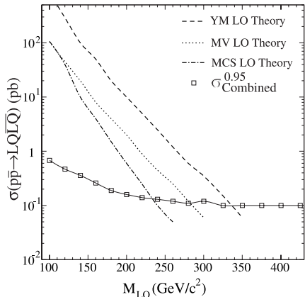
Figure 1. The 95% CL upper limits on cross sections for first generation vector LQ pair production as function of the LQ mass and comparison with LO predictions from different models [8].
