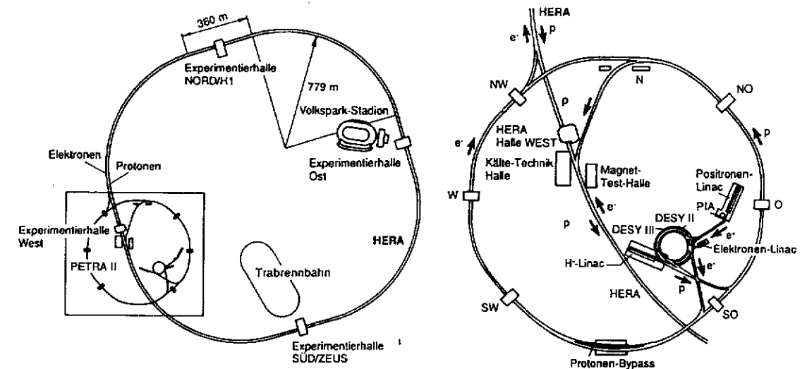
Figure 3.1: HERA and its pre-accelerator system at DESY.
