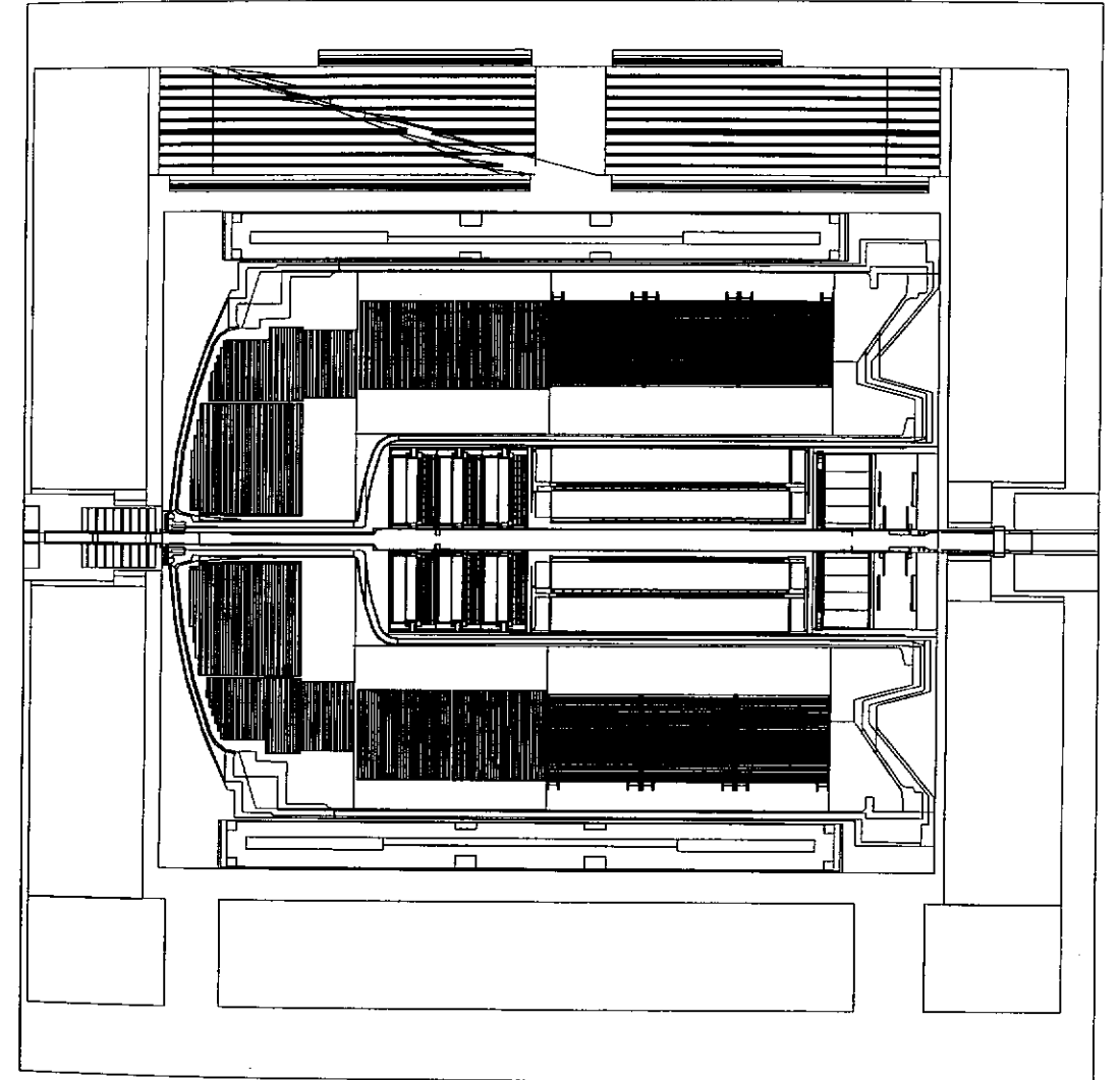
Figure 5.8: Main part of the H1 detector as implemented in the H1 simulation program.
