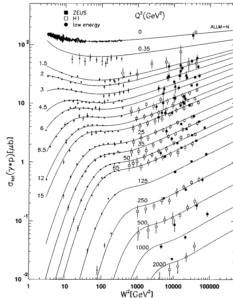
Figure 2.2: Total e-p scattering cross section as a function of W^2 and Q^2 . For real photons ( Q^2 \simeq 0 \text{ GeV}^2 ) the total cross section variation as a function of W^2 is limited between 100 and 200 \mu\text{b} . Much larger variations are observable in the DIS regime for Q^2 larger than 10 \text{GeV}^2 .
