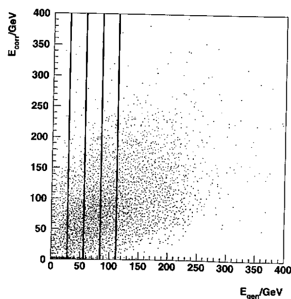
Figure 5.23: Energy correlation plot. The events within the vertical slices have been used to produce the distribution of the corrected energy in fig. 5.24.
