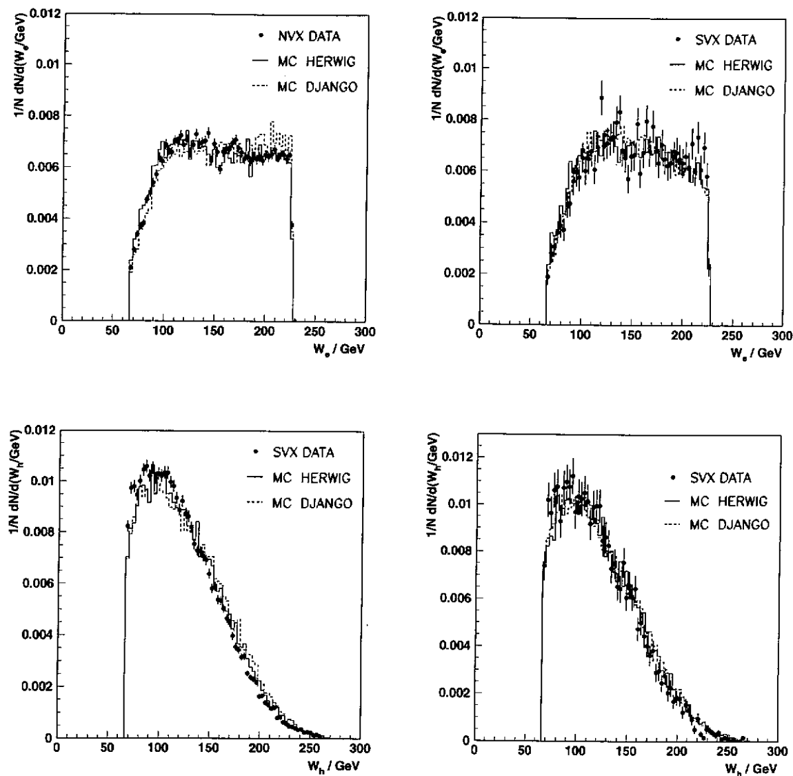
Figure 6.6: Distribution of the invariant mass of the \gamma^* - P system calculated from the electron variables W_e and from hadronic variables W_h , both for the NVX and SVX selections. The data are compared with the MC simulations.
