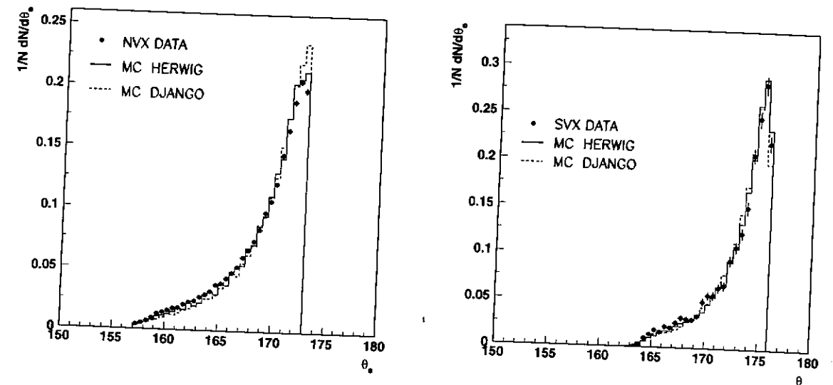
Figure 6.3: Distribution of the electron scattering angle \theta for the NVX and SVX selections. Data are compared to MC simulations.
