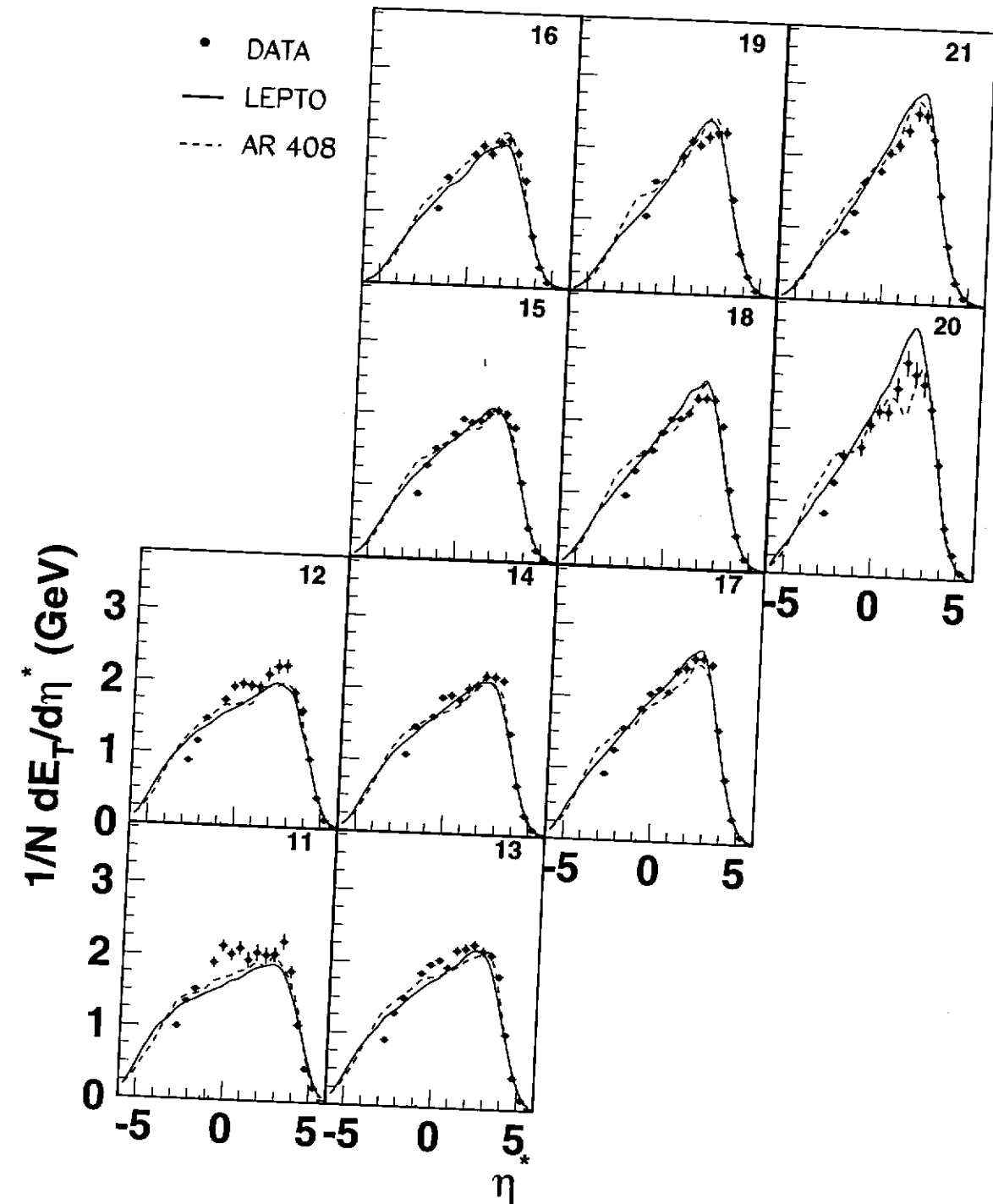
Figure 6.22: The transverse energy flow as a function of the pseudo rapidity \eta^* in the CMS. The measurement concerns the NVX sample and the phase space partition as shown in fig. 6.11. The data is compared with the LEPTO and ARIADNE 4.08 MC-models. The statistical errors are shown.
