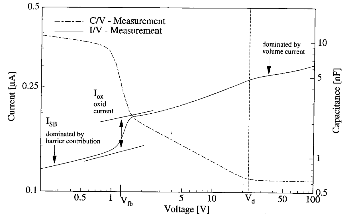
Figure 4.8: Silicon diode current and capacitance vs. voltage characteristics
