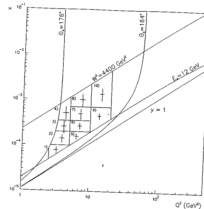
Figure 6.10: Phase space partition for the SVX data sample. The sub-regions (bins) are indicated with the number from 1 to 10 and contain each one the point individuated by the average values of x and Q^2 calculated in the bin. The error bars represent the variable resolution multiplied by the variable average.
