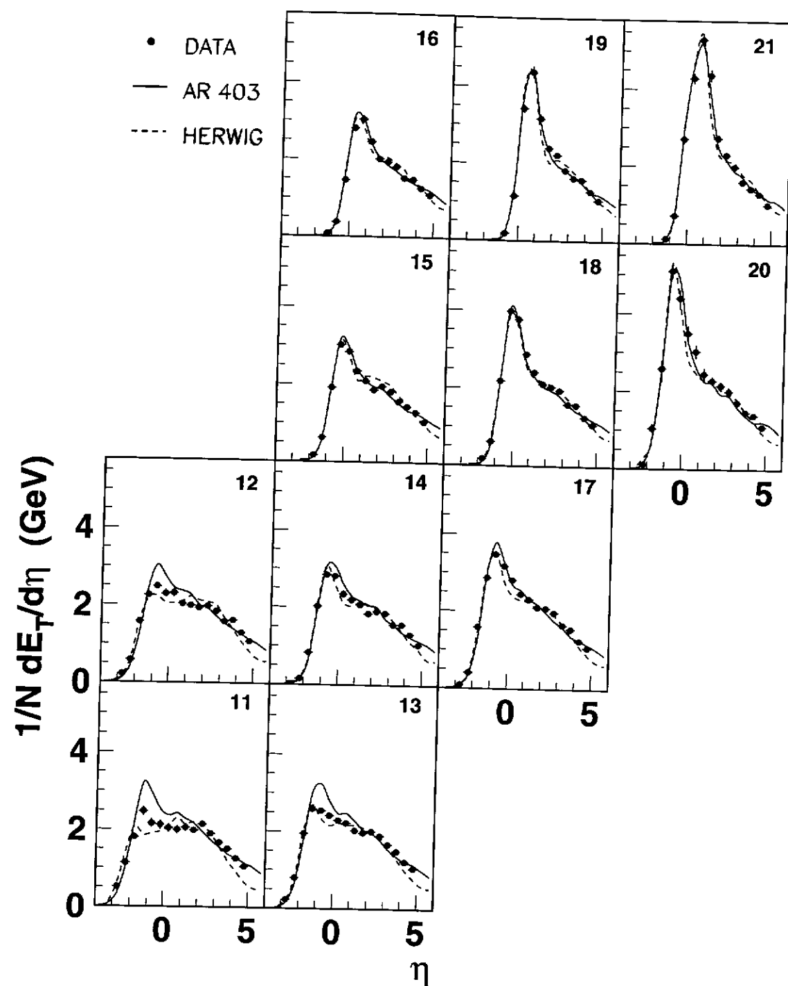
Figure 6.15: The transverse energy flow as a function of the pseudo rapidity \eta in the laboratory system. The measurement concerns the NVX sample and the phase space partition as shown in fig. 6.11. The data is compared with the ARIADNE 4.03 and HERWIG MC-models. Only the statistical errors are shown.
