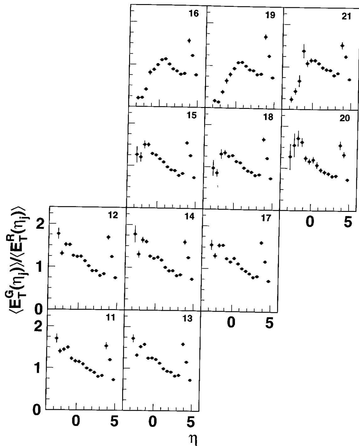
Figure 6.13: Correction factors to the transverse energy flow for the \eta_j interval in the 11 bins indicated with the numbers (11...21) of the phase space (NVX sample). Correction in the laboratory system.
