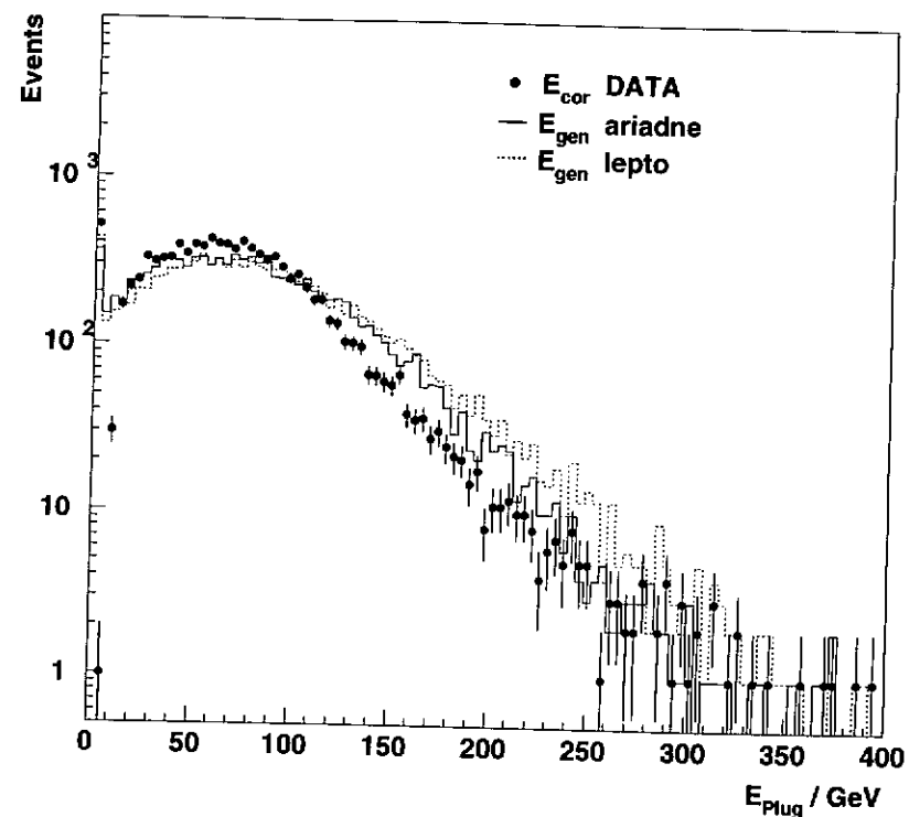
Figure 5.27: Total energy distribution after correction E_{cor} compared to generated energy distributions E_{gen} .
