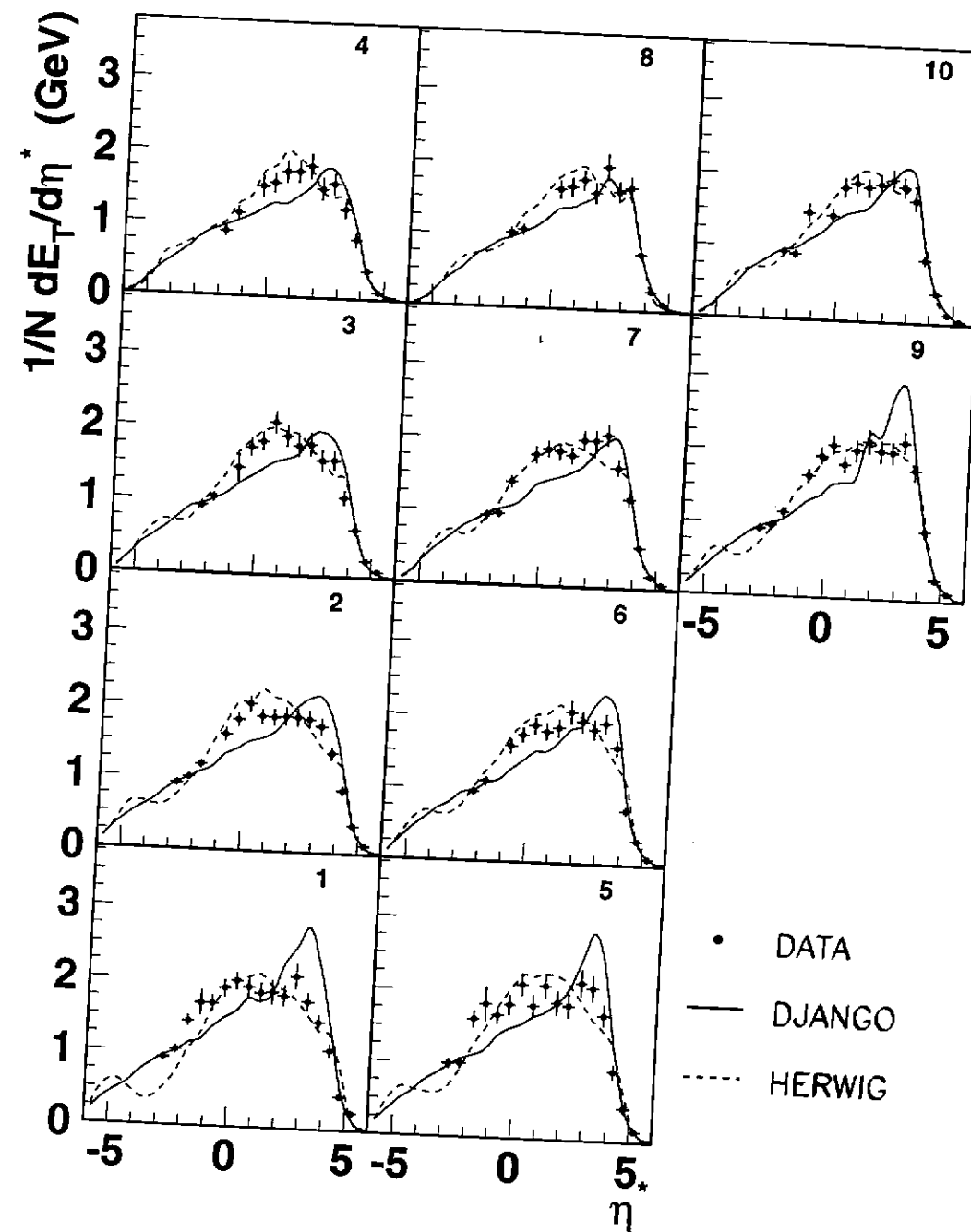
Figure 6.20: The transverse energy flow as a function of the pseudo rapidity \eta^* in the center of mass system (CMS). The measurement concerns the SVX sample and the phase space partition as shown in fig. 6.10. The data is compared with the DJANGO and HERWIG MC-models. The statistical errors are shown.
