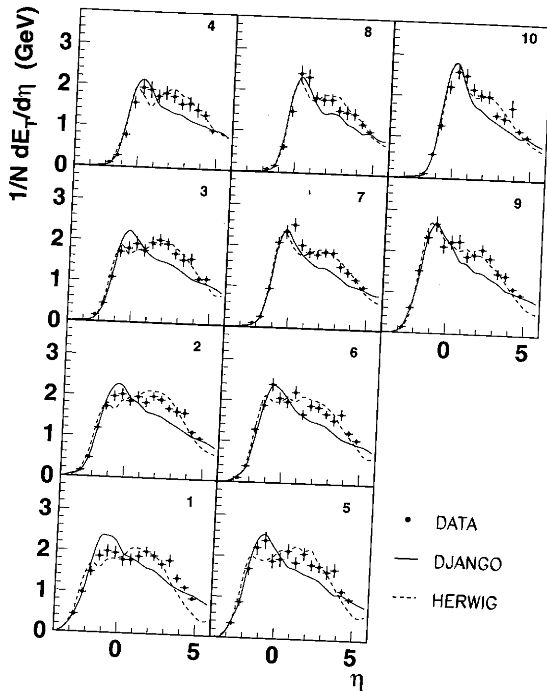
Figure 6.14: The transverse energy flow as a function of the pseudo rapidity \eta in the laboratory system. The measurement concerns the SVX sample and the phase space partition as shown in fig. 6.10. The data is compared with the DJANGO and HERWIG MC-models. Only the statistical errors are shown.
