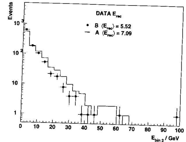
Figure 5.33: Distributions of the reconstructed energy in the central pseudo rapidity bin of the PLUG.
