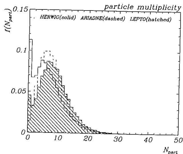
Figure 5.22: Multiplicity distribution generated in the PLUG angular acceptance.
