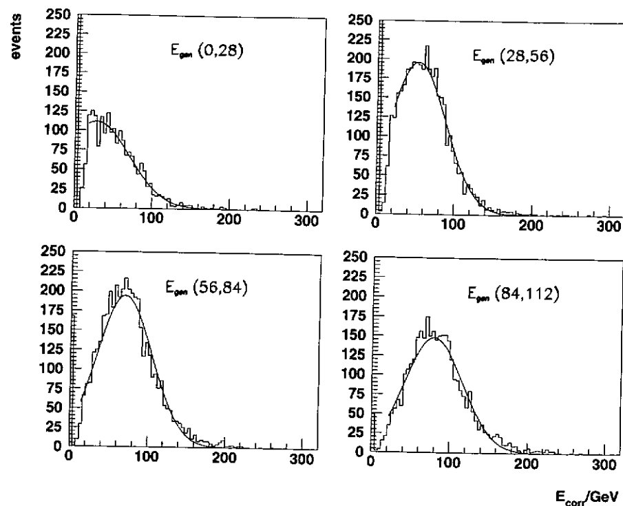
Figure 5.24: Distributions of the corrected energy for different intervals of generated energy E_{gen} shown in the plots. The curves are obtained performing Gaussian fits and avoiding the regions of low corrected energy where the detector is limited in efficiency.
