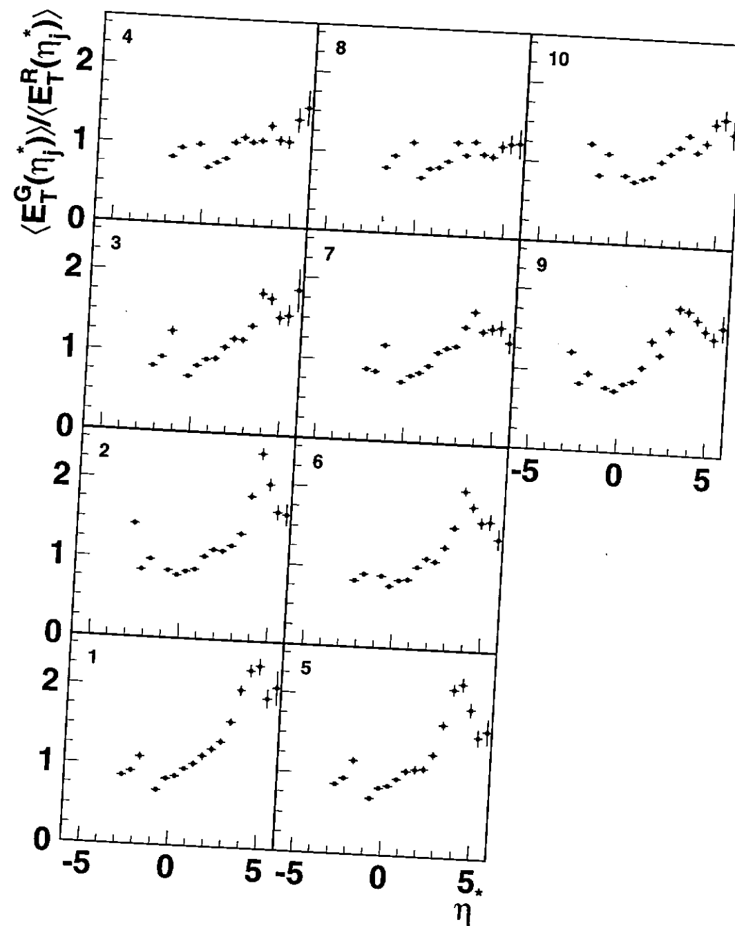
Figure 6.18: Correction factors to the transverse energy flow for the \eta_j^* interval in the 10 bins of the phase space (SVX sample). Correction in the center of mass system.
