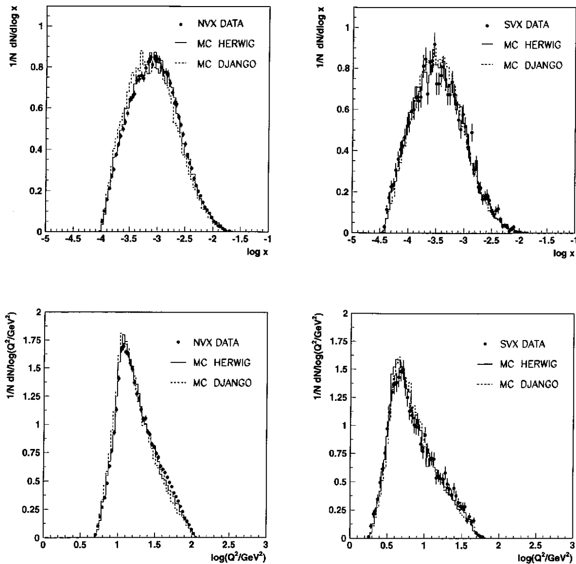
Figure 6.8: Distribution of the kinematic variables x and Q^2 for both the NVX and SVX samples. The data are compared to MC simulations.
