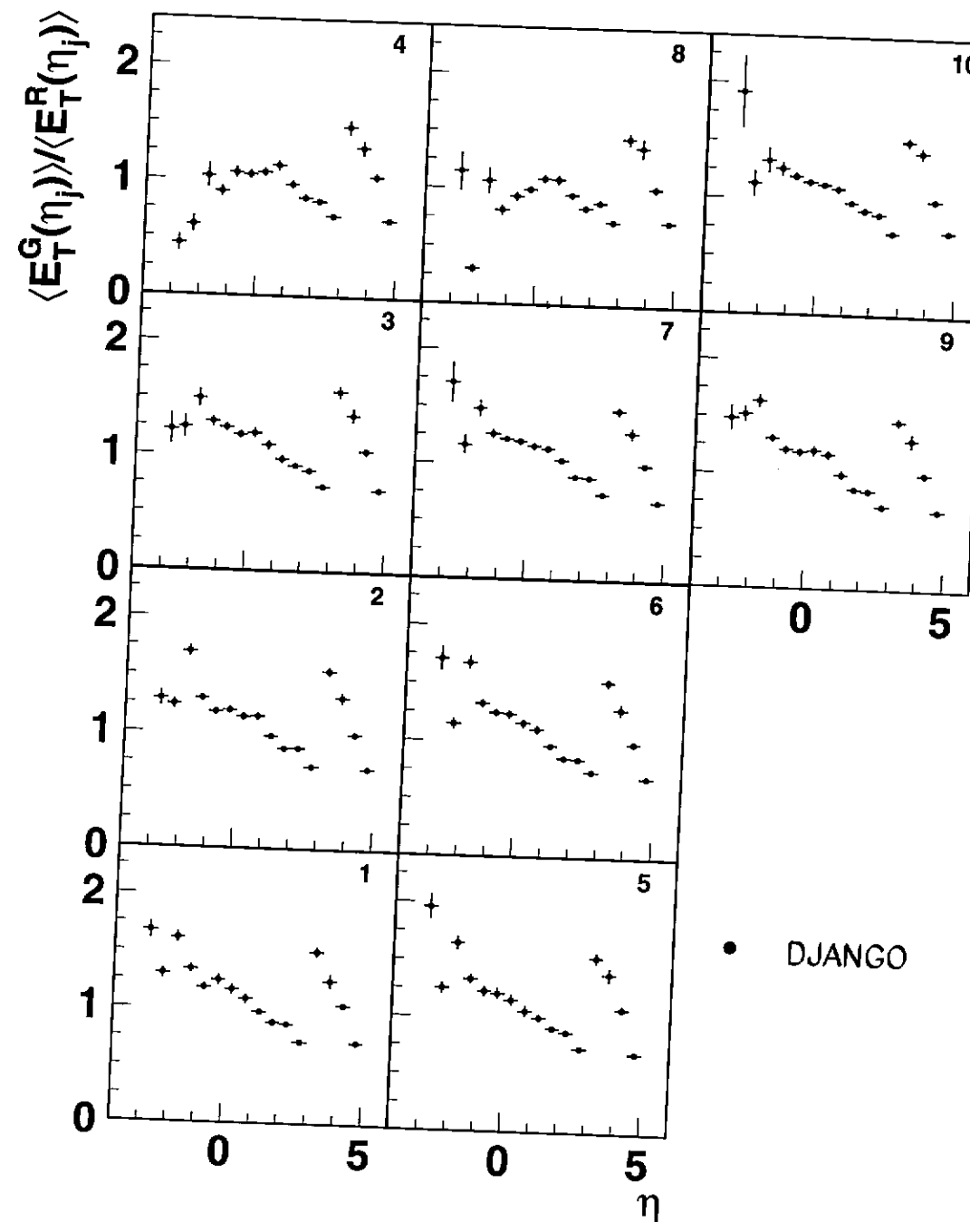
Figure 6.12: Correction factors to the transverse energy flow for the \eta_j interval in the 10 bins of the phase space (SVX sample). Correction in the laboratory system.
