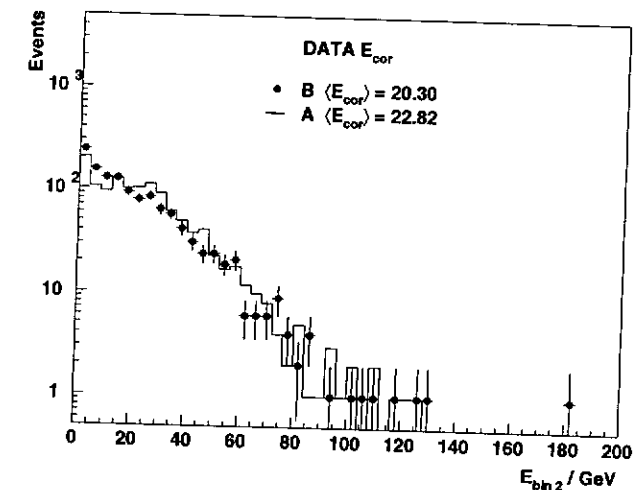
Figure 5.34: Distributions of the corrected energy in the central pseudo rapidity bin of the PLUG.
