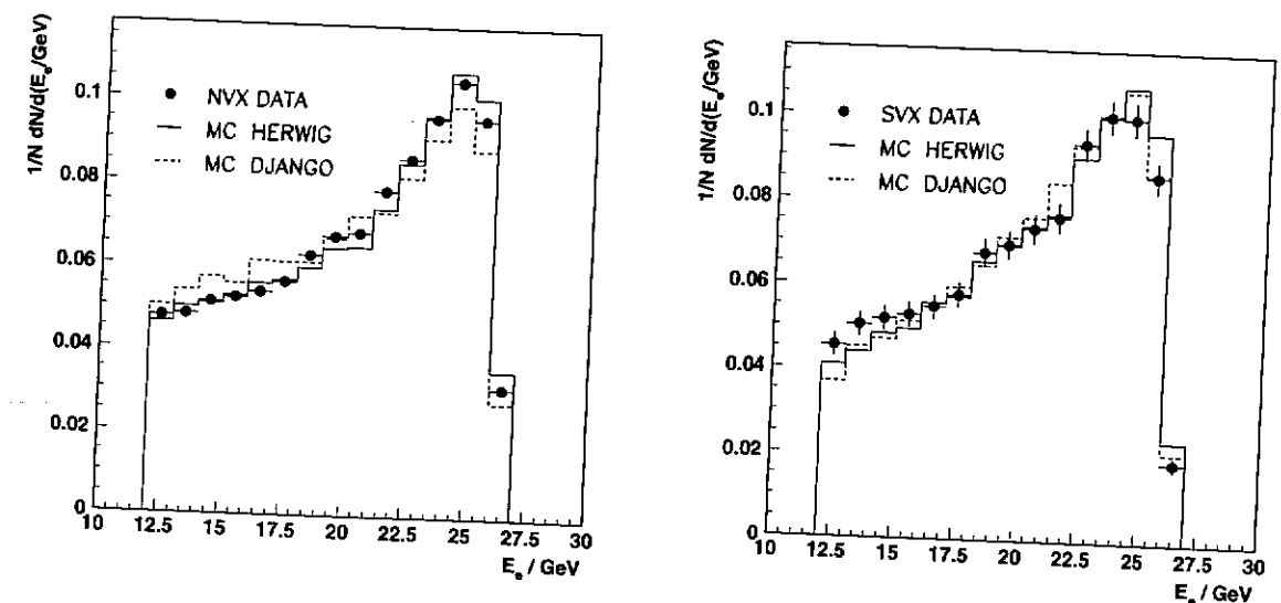
Figure 6.4: Distribution of the scattered electron energy for the NVX and SVX selections. The data are compared to MC simulation.
