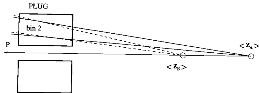
Figure 5.31: The consequence of the vertex displacement on the Plug acceptance in a schematic representation.
