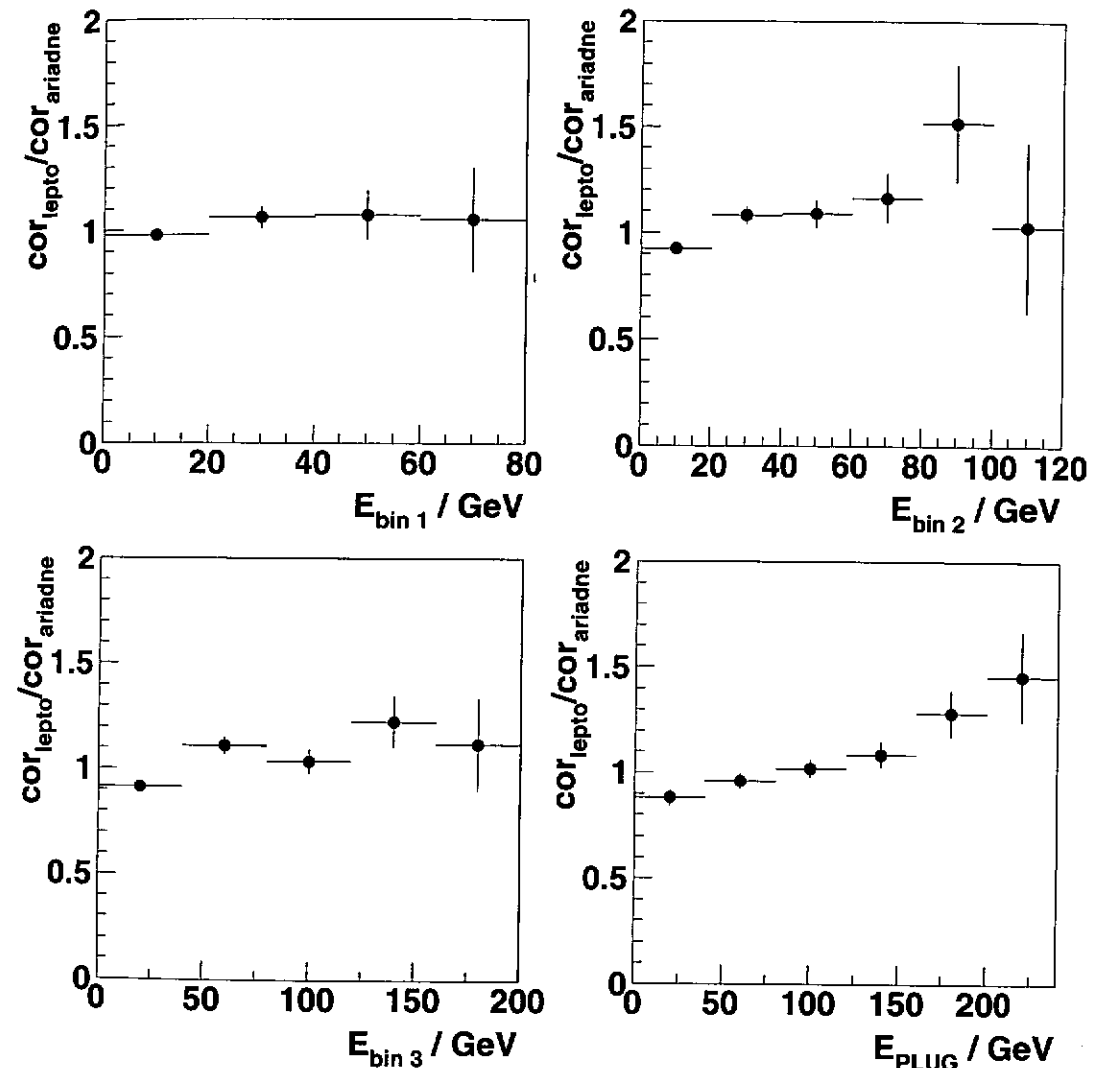
Figure 5.21: Ratio of the corrections bin by bin cor_{lepto}/cor_{ariadne} for the three sub pseudo-rapidity PLUG regions and for their sum.
