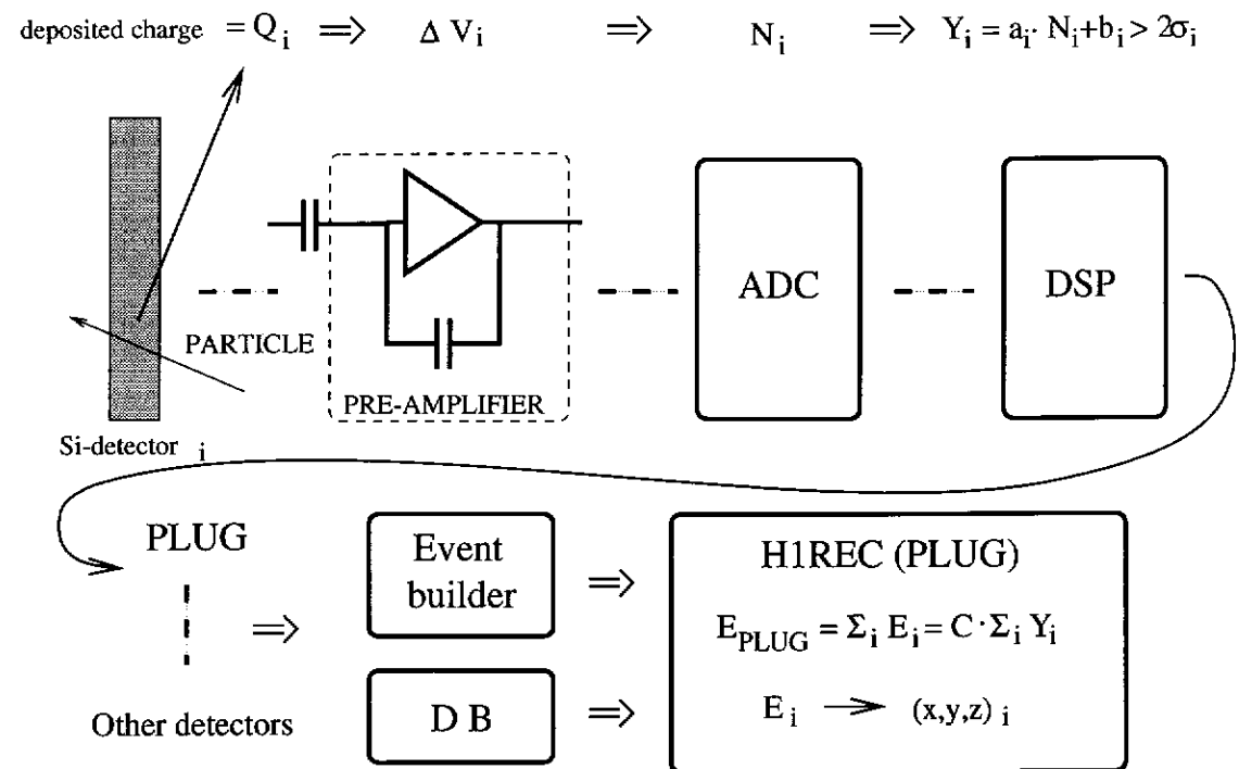
Figure 4.13: Simplified scheme of the data transformation from the detector signal ( Q_i ) to reconstructed data. After the analogue to digital conversion the signal is processed by the DSP. It performs a linear transformation of the signal of each channel. This corresponds to the gain equalization for each of the 336 channel and the pedestal subtraction. The reconstruction program performs further operations and rescales the signals of deposited energy in GeV units taking into account the calorimeter sampling fraction.
