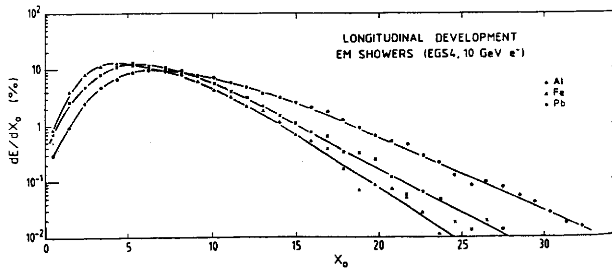
Figure 4.2: Electromagnetic shower development for 10 GeV electrons: specific deposited energy as a function of the radiation length X_0
