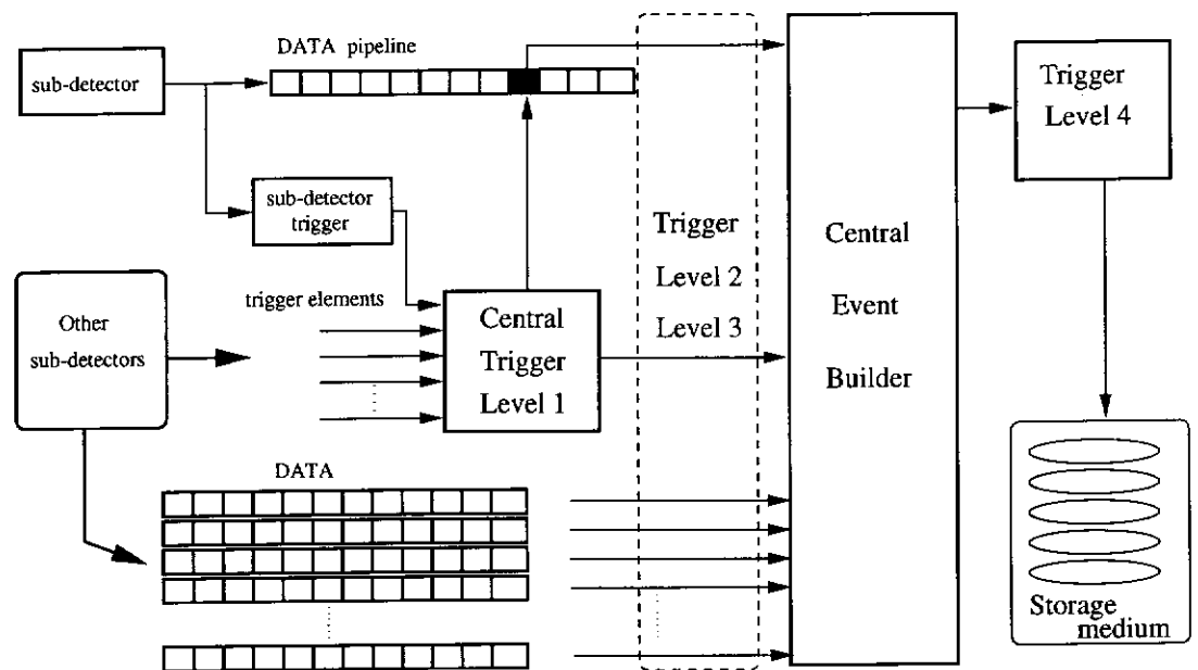
Figure 3.3: Schematic representation of the H1 trigger system.
