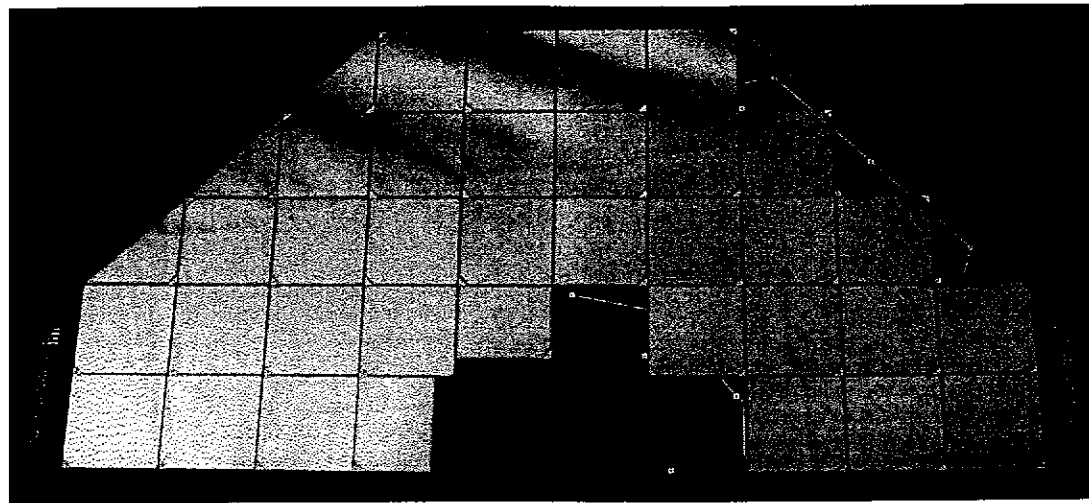
Figure 4.5: Readout board with Si-detectors. This board is contained within two copper slabs each 5 mm thick and constitute a PLUG detector module.
