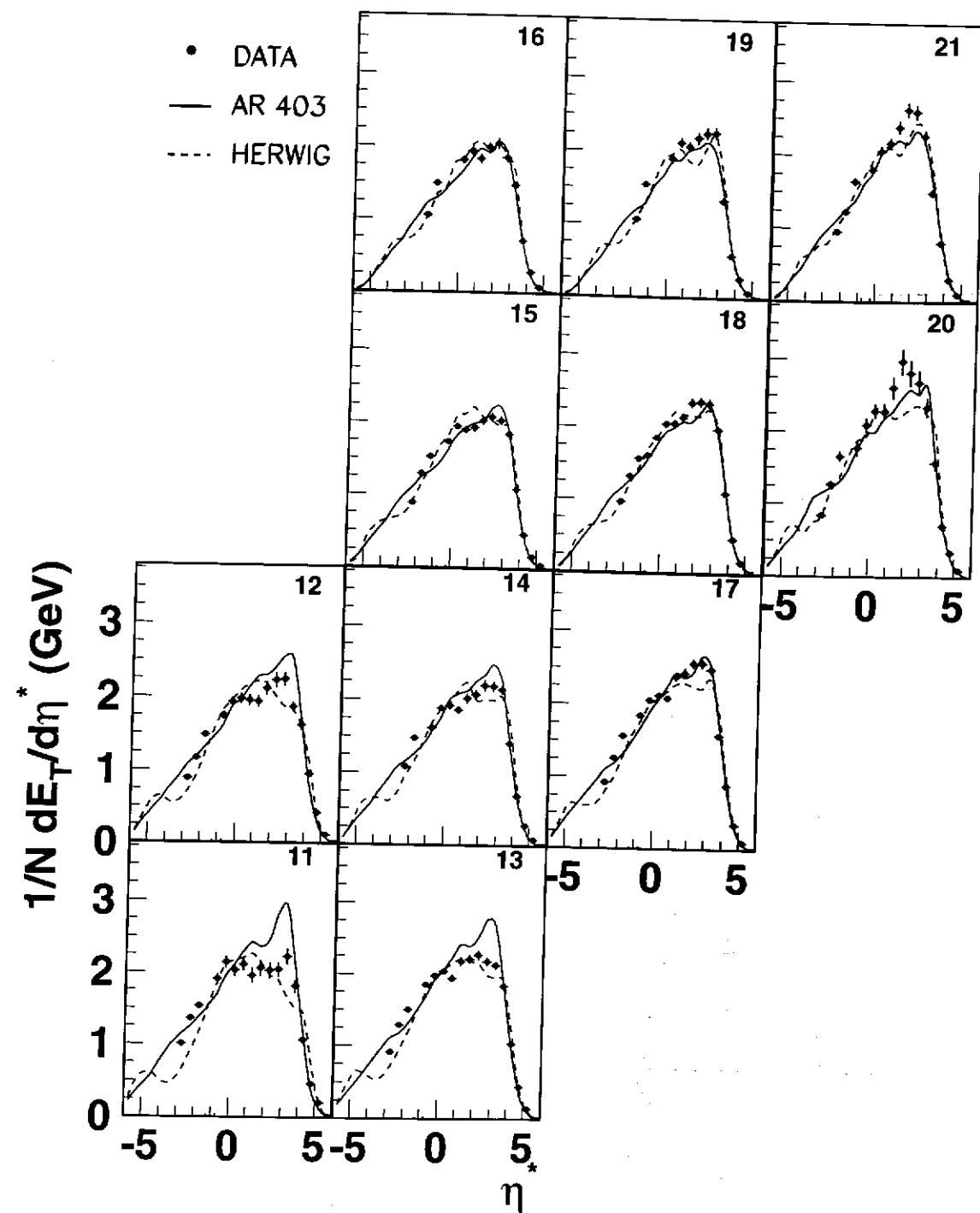
Figure 6.21: The transverse energy flow as a function of the pseudo rapidity \eta^* in the CMS. The measurement concerns the NVX sample and the phase space partition as shown in fig. 6.11. The data is compared with the ARIADNE 4.03 and HERWIG MC-models. The statistical errors are shown.
