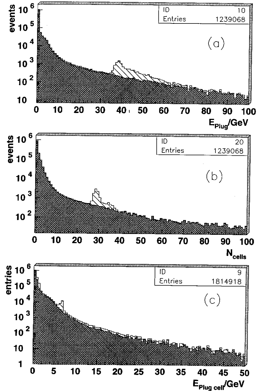
Figure 4.18: The distributions shown here are related to random trigger events collected during 1994 positron running (1807 runs between run N. 82961 and 90419). They show (a) the total energy in the PLUG, (b) the PLUG cell multiplicity and (c) the PLUG cell energy spectrum. The shaded histograms in each plot are after the exclusion of runs with electronics problems
