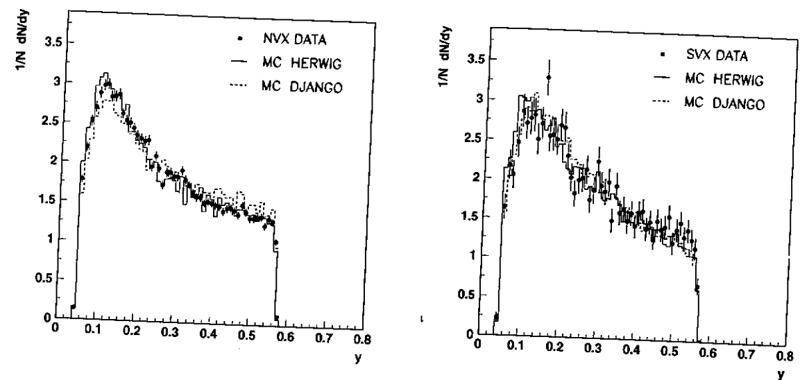
Figure 6.7: Distribution of the kinematic variable y for the NVX and SVX selections. Shown are data compared to MC simulations.
