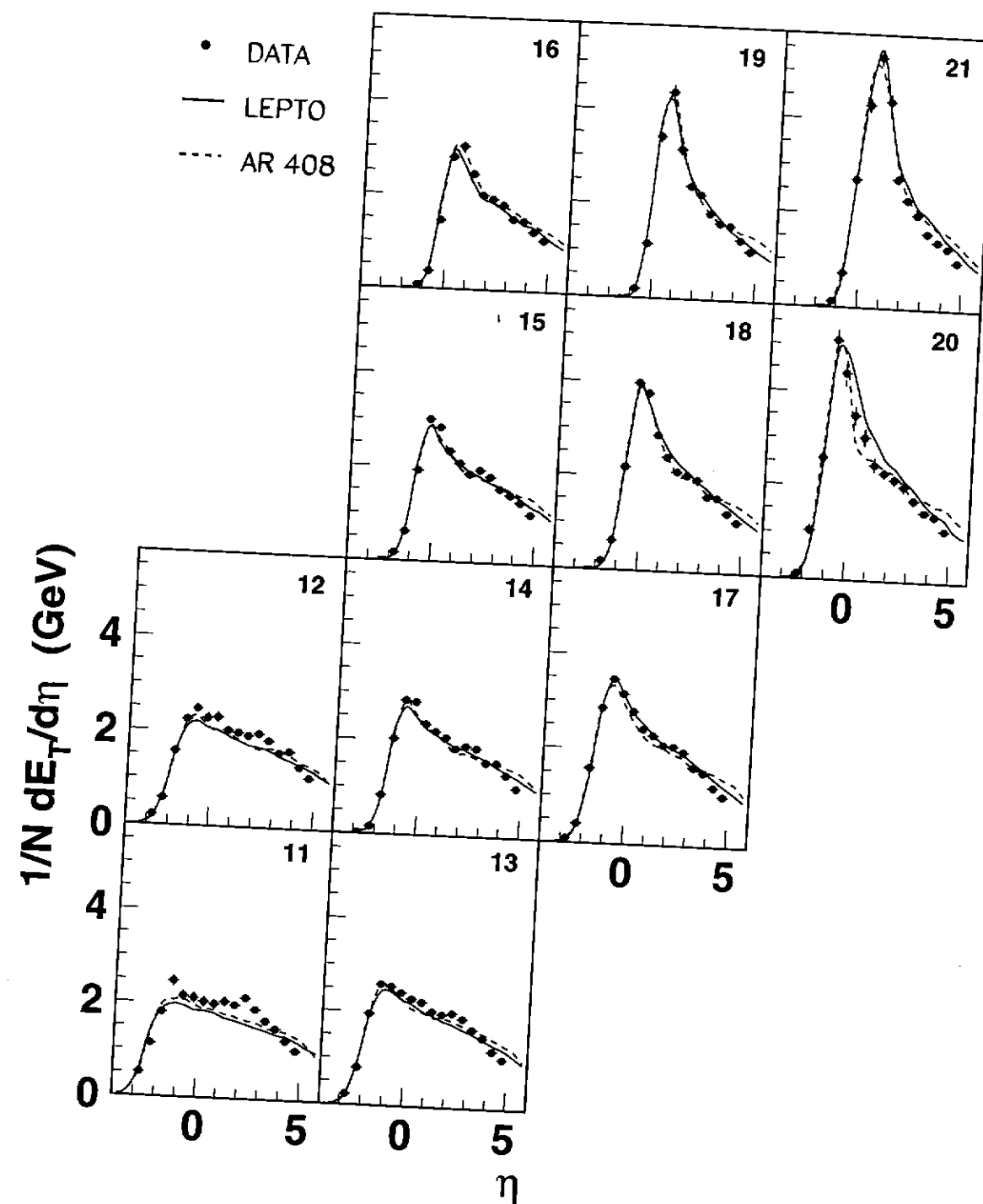
Figure 6.16: The transverse energy flow as a function of the pseudo rapidity \eta in the laboratory system. The measurement concerns the NVX sample and the phase space partition as shown in fig. 6.11. The data are compared with the LEPTO6.5 and ARIADNE 4.08 MC-models. Only the statistical errors are shown.
