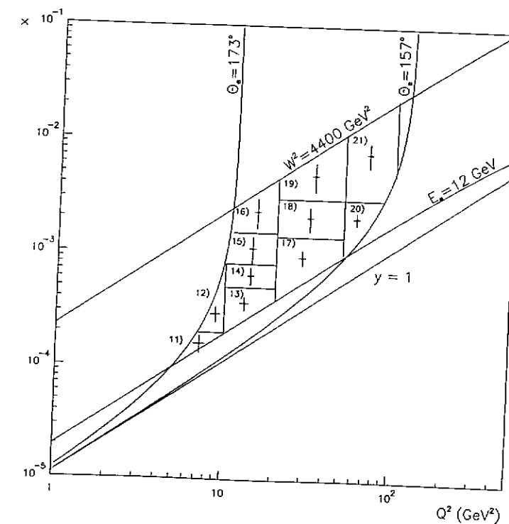
Figure 6.11: Phase space partition for the NVX data. The bins are indicated with the number from 11 to 21. The average values of x and Q^2 calculated in each bin are shown with error bars representing the variable resolution multiplied the variable average.
