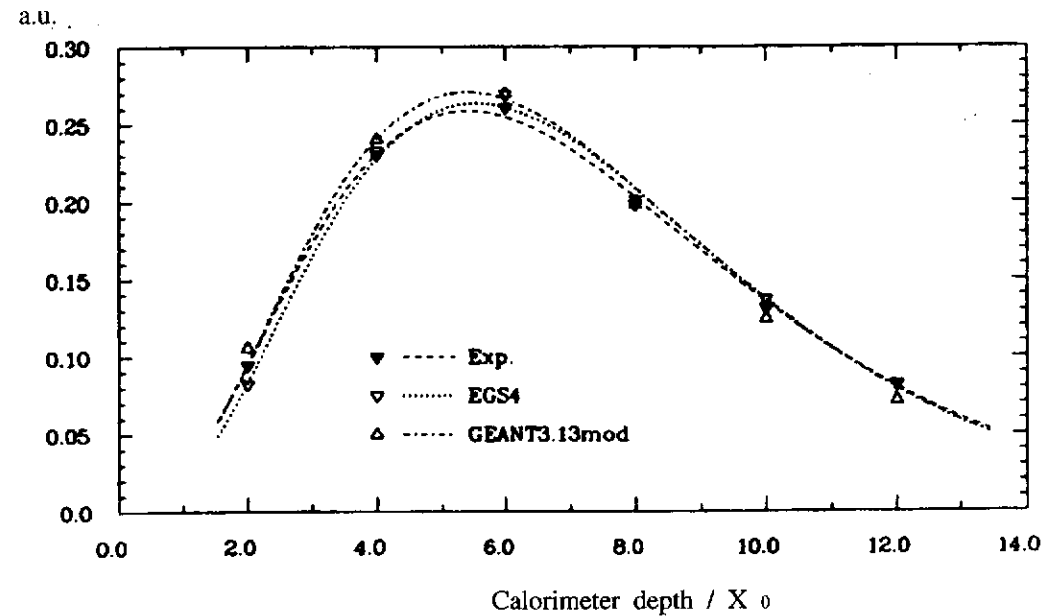
Figure 5.7: Electromagnetic shower development induced by 6 GeV electrons in a Si-W calorimeter compared with MC simulation.
