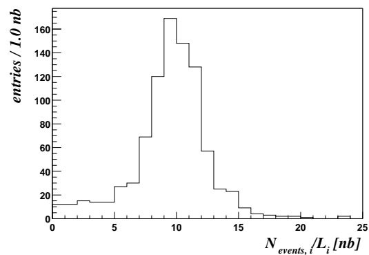
Figure 3.4: Stability of S50: Part a) shows the number selected events ( N ) as function of the accumulated luminosity ( \mathcal{L} ), b) shows the ratio N/\mathcal{L} of events per run as function of the run number and c) shows the frequency distribution of the ratio N/\mathcal{L} .
