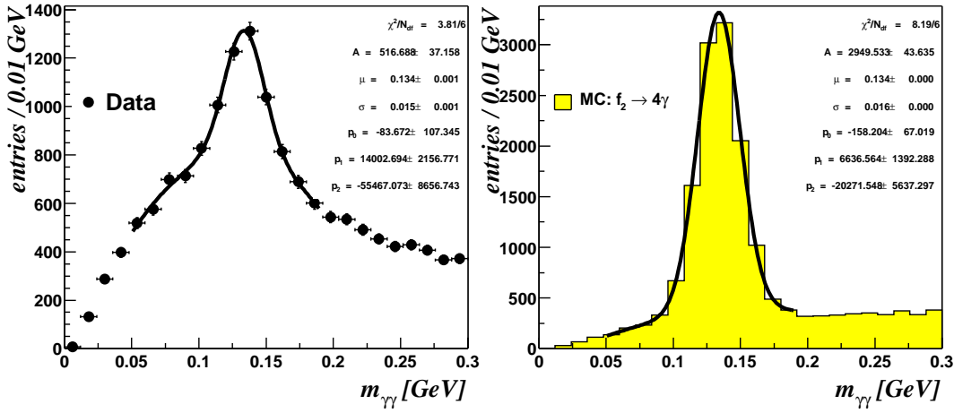
Figure 6.1: Pion-candidates as seen in data and Monte Carlo: The spectra of photon-photon masses are shown for data in the left and Monte Carlo ( \mathcal{O}PIUM f_2 \rightarrow \pi^0\pi^0 ) in the right. The curve shows fits of a Gaussian together with third order polynomial.
