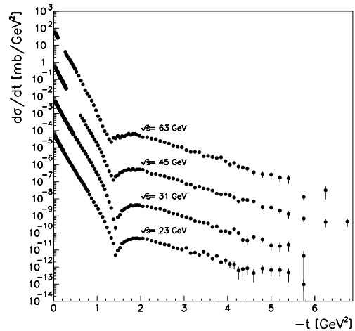
Figure 1.4: Angular spectrum in nucleon nucleon scattering: d\sigma/d|t| as seen in pp scattering at centre of mass energies of \sqrt{s} = 23.5, 30.7, 44.7 and 62.5 GeV measured at the ISR [7]. The respective cross sections were scaled by factors of 10^{-6}, 10^{-4} and 10^{-2} for better visibility.
