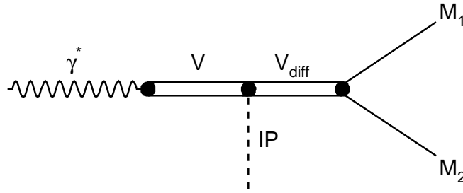
Figure 4.2: Diffractive dissociation as modelled by Pythia: A photon is turned into a vector meson V according to the VMD and subsequently interacts with the Pomeron. This interaction excites the vector meson into a state called V_{\text{diff}} , that decays into two mesons M_1 and M_2 if m_{V_{\text{diff}}}^2 < (|\mathbf{p}_{V_{\text{diff}}}| - \hat{m})^2 .
