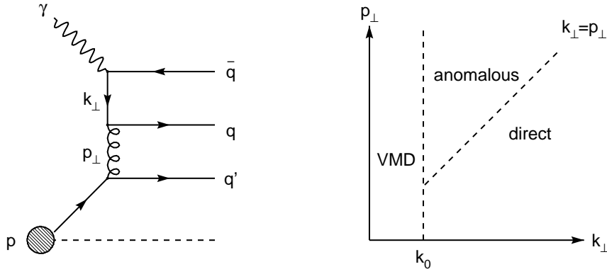
Figure 1.3: The scales k_{\perp} and p_{\perp} in photoproduction: The left part shows an illustration of the scales k_{\perp} and p_{\perp} in a schematic graph of a hard \gamma p interaction. The right part shows the classification of \gamma p interactions in the (k_{\perp}, p_{\perp}) -phase space.
