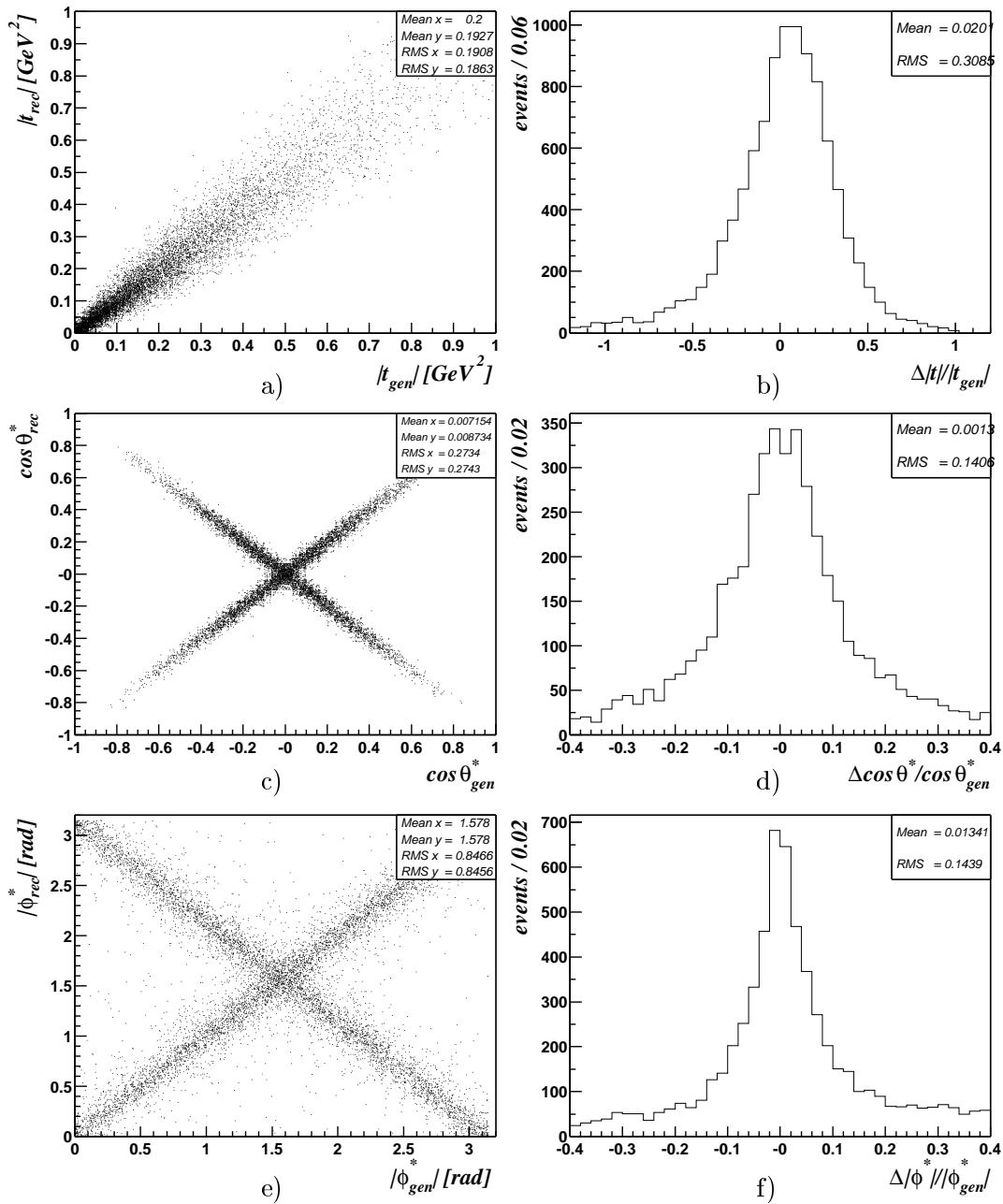
Figure 6.14: Resolutions for the f_2 (IV): The figure shows the same as in figure 6.11 but for the momentum transfer squared |t| a)+b), the decay-angular distributions \cos\vartheta^* c)+d) and |\varphi^*| .
