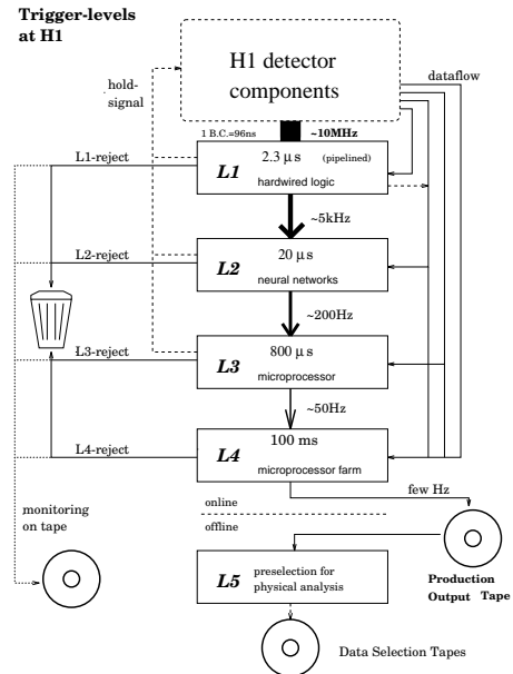
Figure 2.5: The trigger concept of H1: The figure shows the H1 trigger concept with its 5 levels and the respective input rates entering the various levels.
