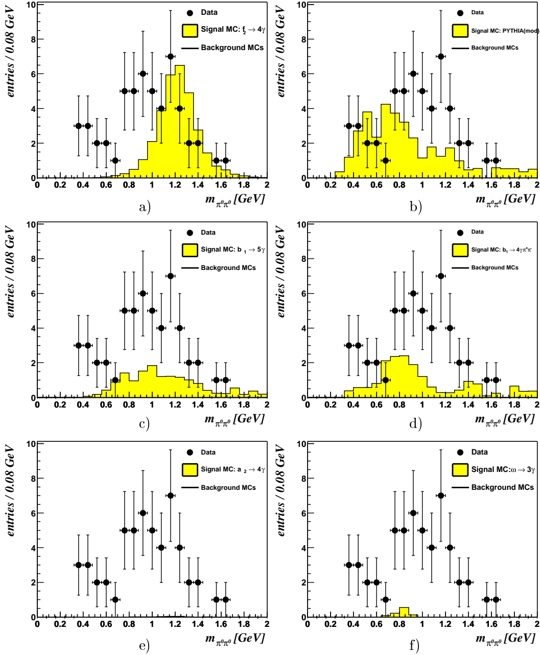
Figure 6.6: Contributions of the Monte Carlos: The mass distributions of the Monte Carlos contributing to the \pi^0\pi^0 sample are shown separately together with data. Part a) shows the signal process f_2 \rightarrow \pi^0\pi^0 , part b) shows the dominant background as predicted by PYTHIA(mod). The two panels in the middle c) and d) show the b_1 decaying purely into photons b_1 \rightarrow \omega\pi^0 \rightarrow (\pi^0\gamma)\pi^0 \rightarrow 5\gamma and b_1 \rightarrow \omega\pi^0 \rightarrow (\pi^+\pi^-\pi^0)\pi^0 \rightarrow \pi^+\pi^-4\gamma , and panels e) and f) show respectively how the a_2 \rightarrow \pi^0\eta and the \omega \rightarrow \pi^0\gamma contribute.
