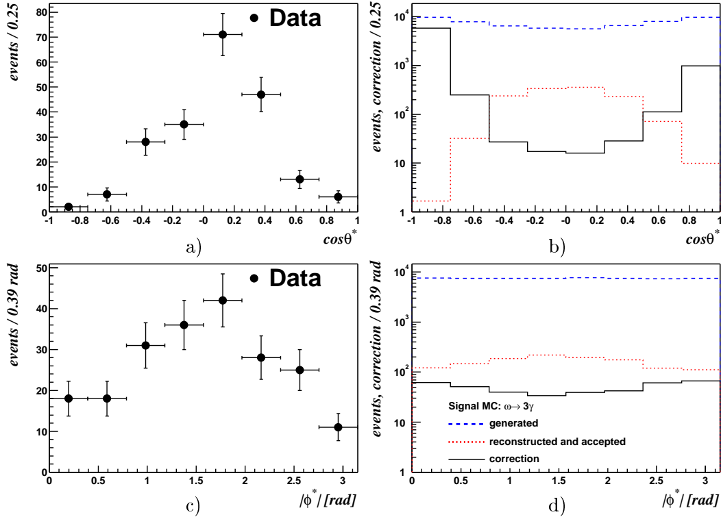
Figure 5.13: Decay angular distributions and their corrections: Parts a) and c) show the \cos\vartheta^* - and the |\varphi^*| distributions before the correction is applied. Parts b) and d) show respectively the Monte Carlo distributions as they were generated (upper dashed histogram) and how they are reconstructed after application of the cuts (lower dashed histogram). The full histogram is the correction to be applied to data.
