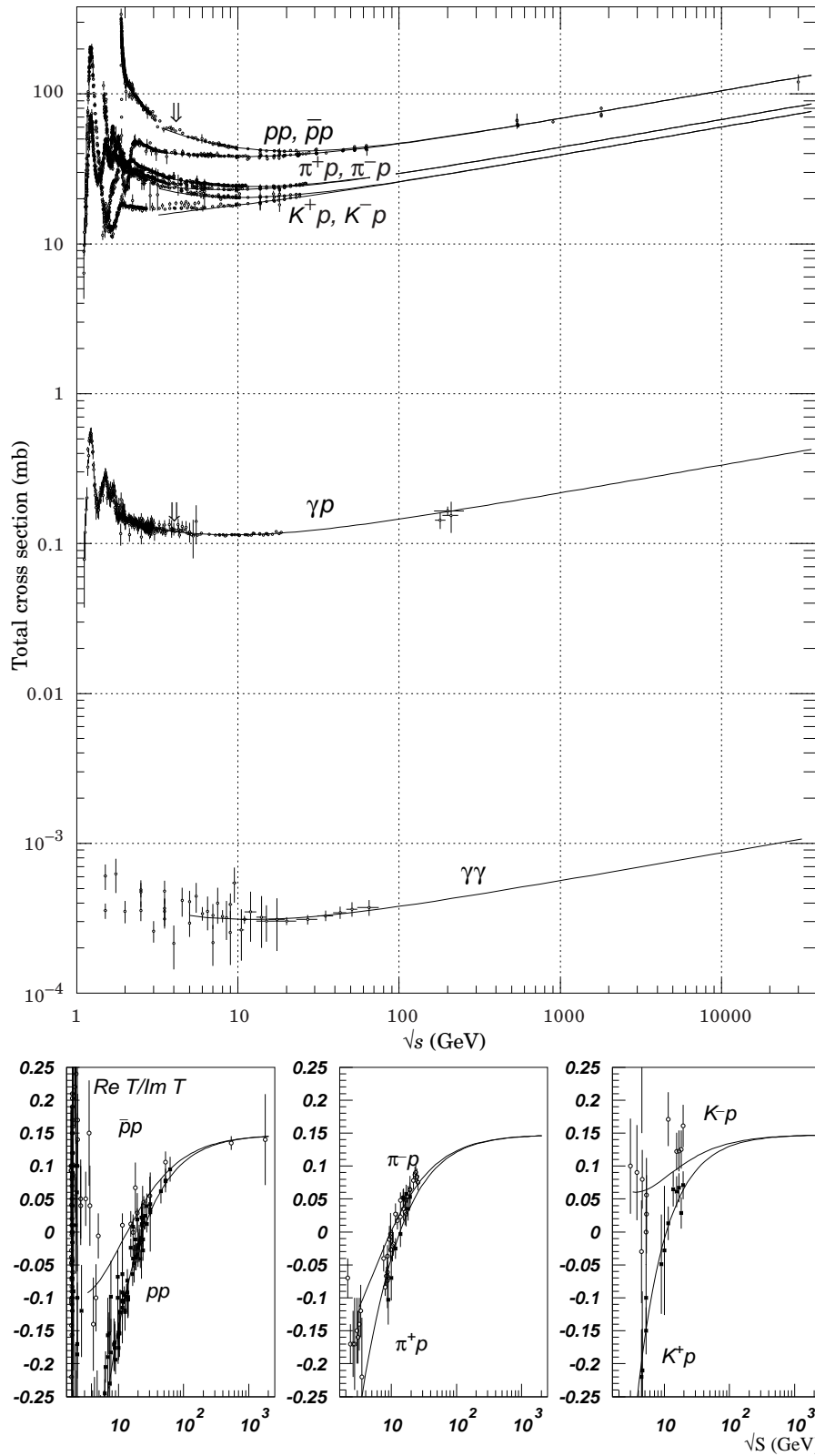
Figure 1.9: Fit to total cross sections and \rho -parameters: The upper part shows a fit performed in [34] to total cross sections for p^\pm p , \pi^\pm p , \pi^\pm p , \gamma p and \gamma\gamma reactions. The lower part shows the fit to the \rho -parameter for p^\pm p , \pi^\pm p and K^\pm p reactions.
