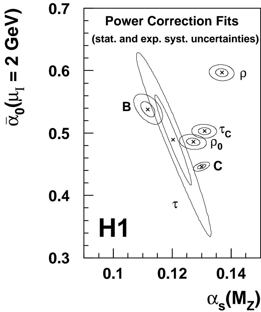
Figure 2: Results of power correction fits to the mean values of event shape variables \tau , \tau_C , B , C , \rho and \rho_0 (p-scheme) with contours of \chi^2(\alpha_s, \bar{\alpha}_0) = \chi_{min}^2 + 1 and \chi^2(\alpha_s, \bar{\alpha}_0) = \chi_{min}^2 + 4 including statistical and experimental systematic uncertainties.
