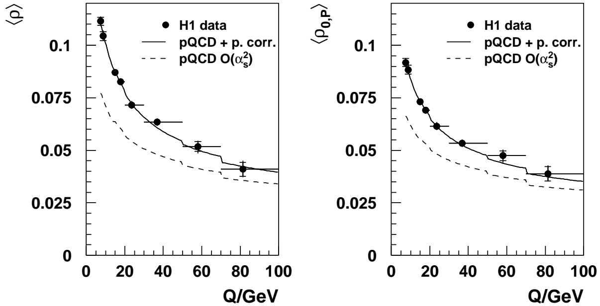
Figure 1: Mean values of \rho (left, from [1]) and \rho_0 in the p-scheme (right) as a function of Q . The error bars represent statistical and systematic uncertainties. The full line corresponds to a power correction fit with parameters \bar{\alpha}_0 and \alpha_s ; the dashed line shows the pQCD contribution.
