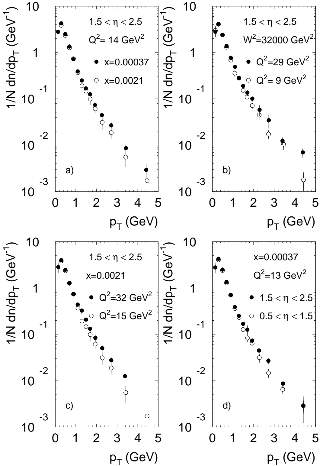
Figure 3: a) Comparison of the p_T spectra at high x (bin 6) and at low x (bin 3) for fixed (intermediate) Q^2 . b) Comparison of the p_T spectra at two different Q^2 values (bins 2 and 7) for fixed (large) W . c) Comparison of the p_T spectra at two different Q^2 values (bins 6 and 8) for fixed (large) x . d) Comparison of the p_T spectra in two different \eta intervals in the kinematic bin 3 (low x , intermediate Q^2 ). The mean values of x and Q^2 are indicated in the figures. The error bars represent the quadratic sum of the statistical and systematic errors.
