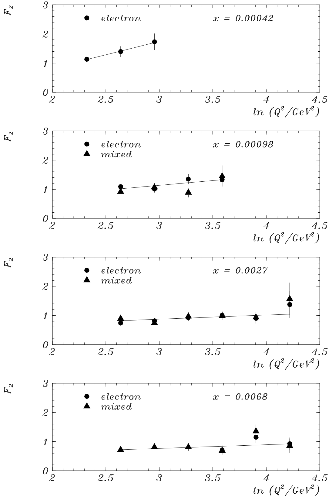
Figure 1: The measured structure function F_2(x, Q^2) for different values of x with statistical errors only. All points are subject to a global normalization uncertainty of 8% [2]. The lines are straight line fits to the electron data for x < 0.001 and to the mixed data at higher x .
