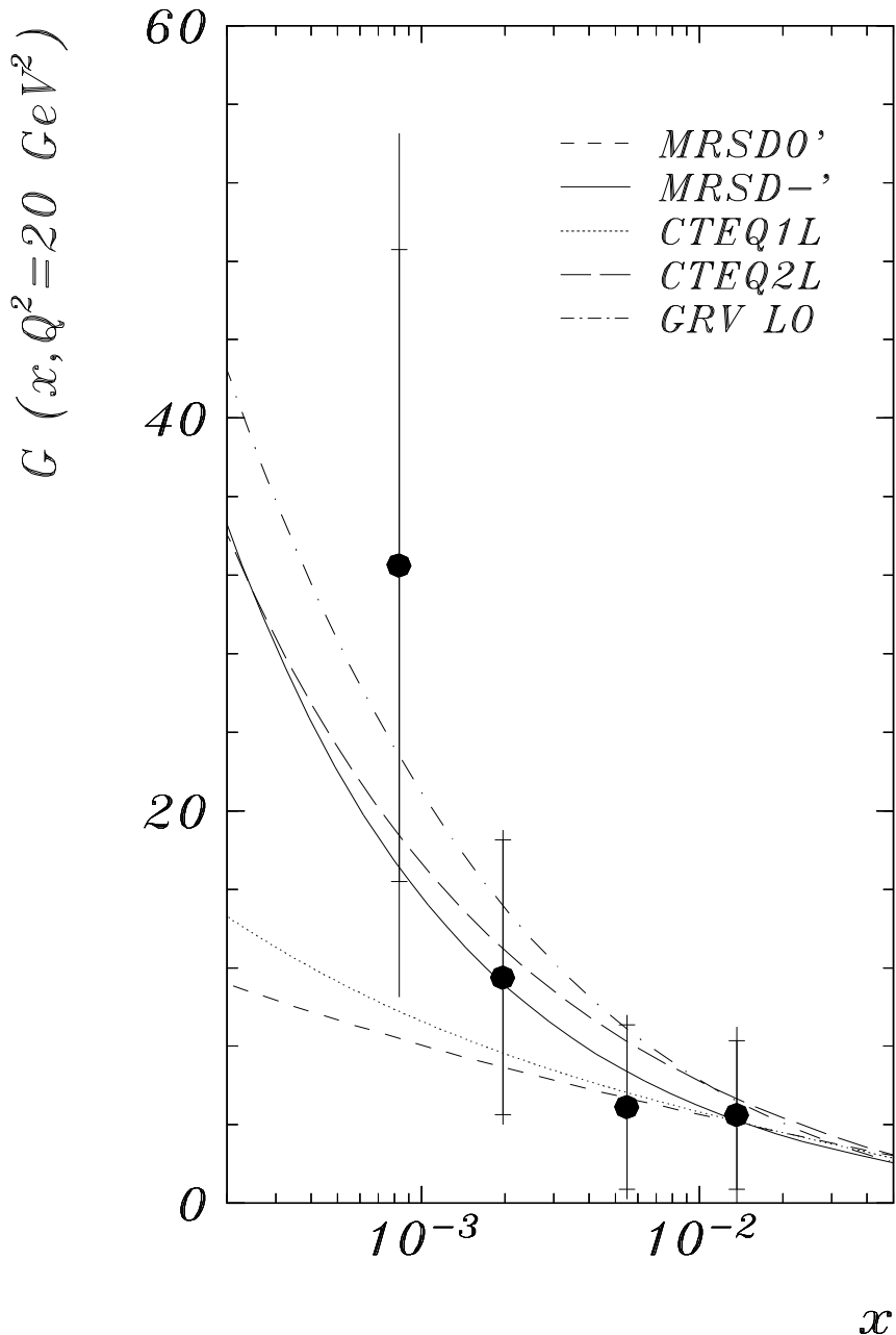
Figure 2: The gluon distribution function G(x, Q^2) at Q^2 = 20 \text{ GeV}^2 . The inner errors are the statistical errors, the full bars represent the systematic and the statistical errors added in quadrature. The curves represent different parametrizations of G [14, 15, 16]. The CTEQ and GRV curves are leading-order parametrizations, while the MRS parametrizations are given in the DIS renormalization scheme. CTEQ2 denotes a global analysis including the recent HERA structure function data.
