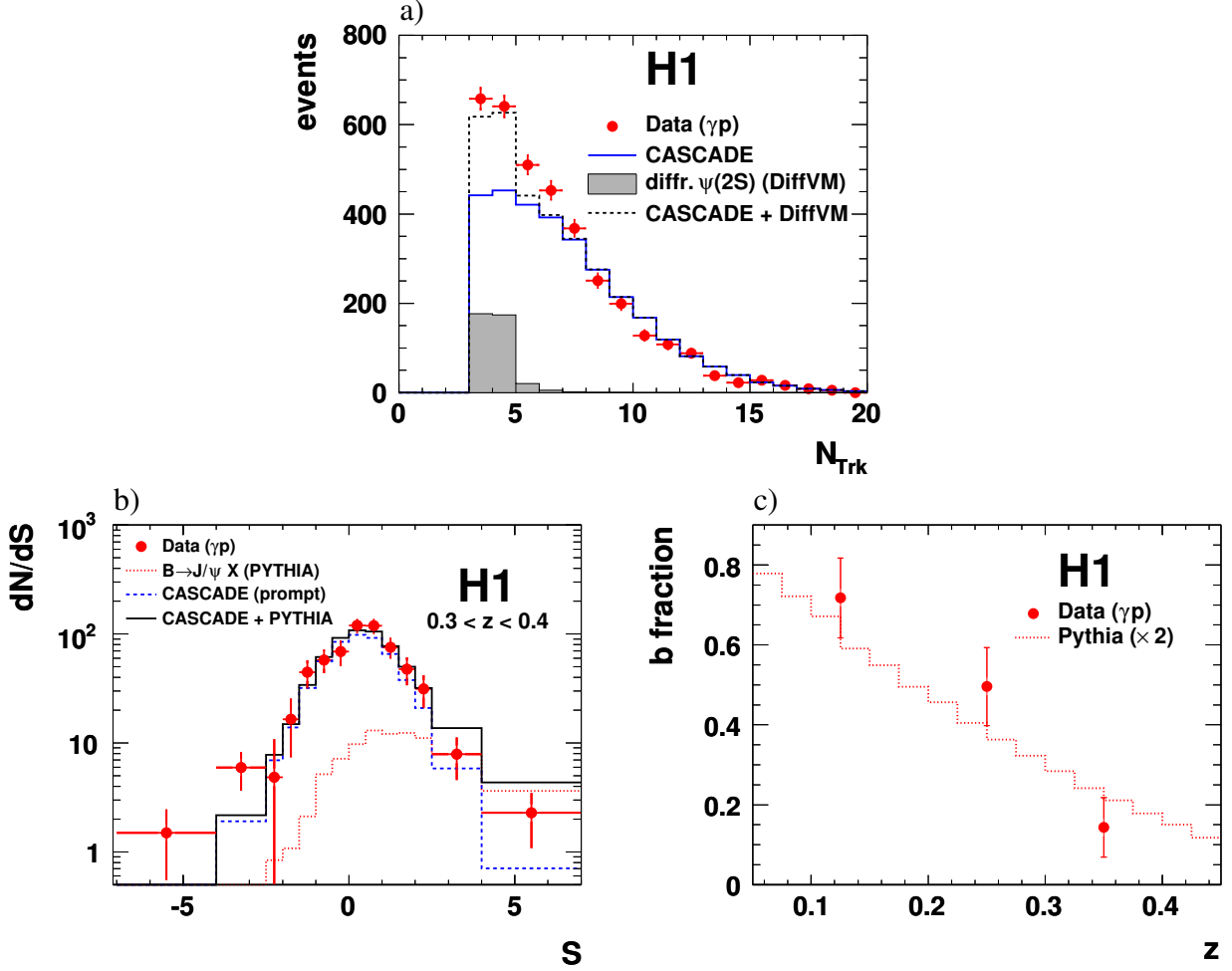
Figure 4: a) Distribution of the multiplicity of tracks, N_{Trk} , in the central region of the detector ( 20^\circ < \theta < 160^\circ ) for the photoproduction sample, b) signed significance distribution S for the photoproduction sample at low elasticities ( 0.3 < z < 0.4 ) and c) measured contribution from b hadron decays for three bins of the elasticity z in comparison with the prediction based on PYTHIA (scaled up by a factor of two) and CASCADE.
