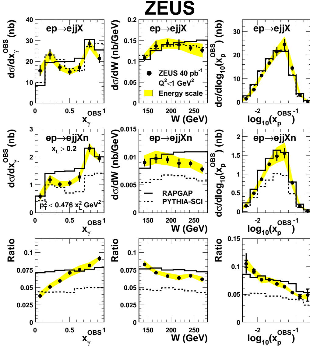
Figure 3: Differential neutron-tagged and untagged dijet photoproduction cross sections as functions of x_\gamma^{\text{OBS}} , W and \log_{10}(x_p^{\text{OBS}}) . The ratios between cross sections, the neutron yields, are also given. Details are as in Fig. 2.
