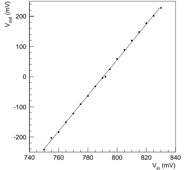
Figure 8. Calibration measurement based on the integration of an externally applied current to the amplifier input. Horizontal scale ( V_{in} ): proportional to input current, Vertical scale: pulse height at chip output
