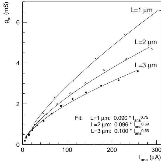
Figure 5. Transconductance g_m versus current for different channel length L measured on a test-structure for the new APC128-DMILL. A fit of the form g_m = aI_{ana}^b was performed.
