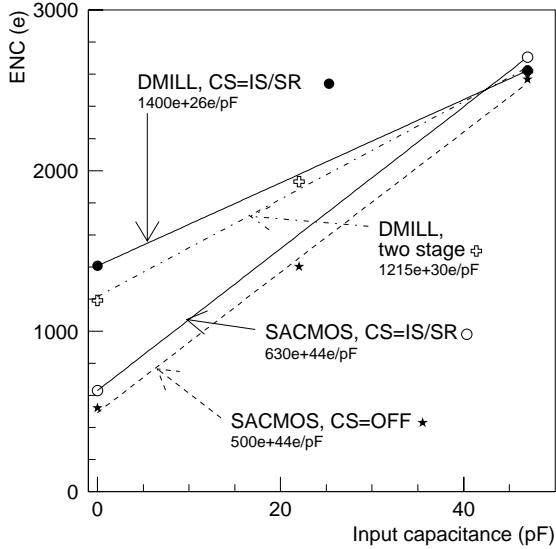
Figure 9. Measured noise performance (ENC) as a function of the input capacitance for different operation modes of the APC chip in SACMOS and DMILL technology (see text for details).
