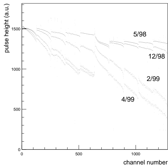
Figure 2. Four sets of pedestals of the SACMOS Analog Pipeline Chip in the CST-Detector at H1 indicating radiation damage of the chips as a function of date from May '98 to April '99. The channel number is proportional to the time the channel waits until it is read out (see text for details).
