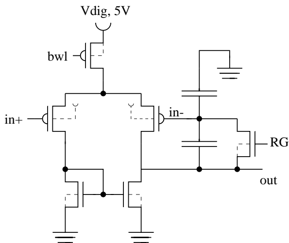
Figure 3. Simple transconductance amplifier with feedback loop as described in the text.
