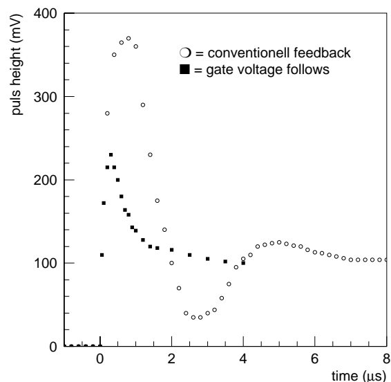
Figure 7. Response of the second amplifier stage to a 100 mV signal step applied to the input.
