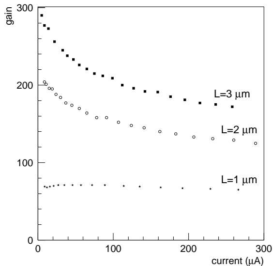
Figure 6. Open loop gain versus current for different channel length L measured on a test-structure for the new APC128-DMILL
