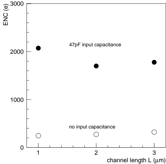
Figure 10. Measured ENC for single-stage-amplifier with channel length of L=1 \mu\text{m} , L=2 \mu\text{m} and L=3 \mu\text{m} .
