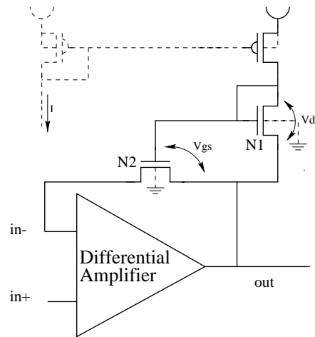
Figure 4. Feedback configuration of second prototype variation for the pipeline buffer stage, see text for details. The capacitive divider is omitted for clarity.
