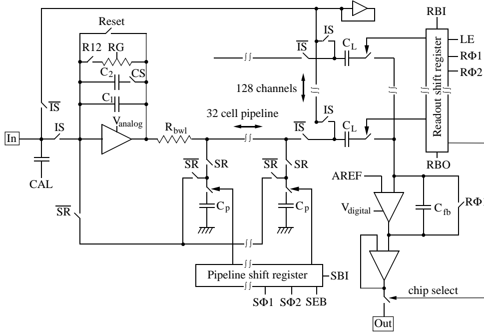
Figure 1. Electrical diagram of the Analog Pipeline Chip
