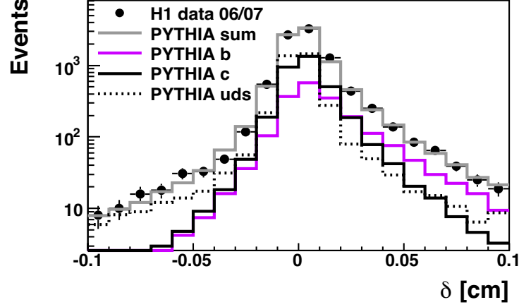
Figure 6.4: The \delta distribution for the selected events. The data (points) in comparison to the PYTHIA Monte Carlo simulation.
