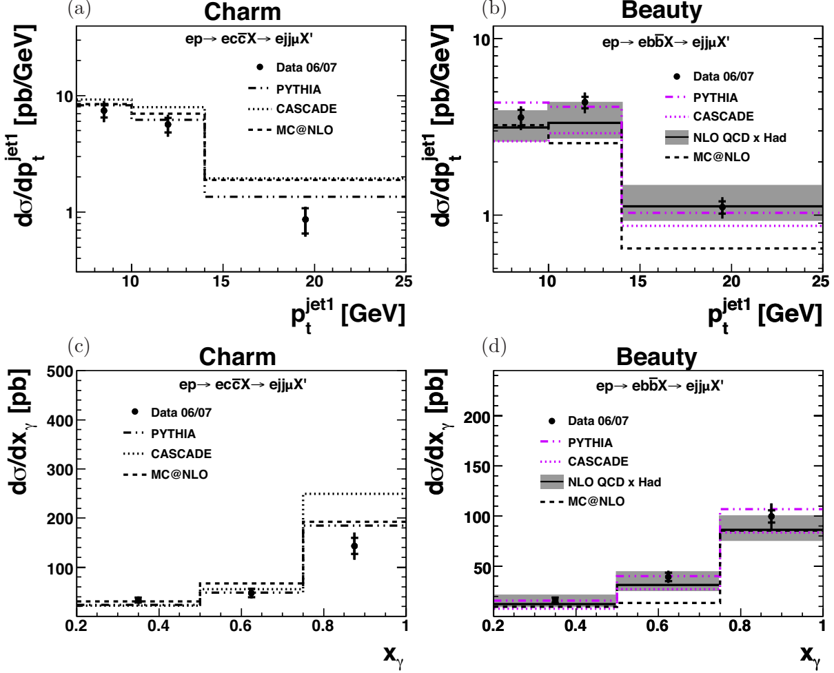
Figure 7.5: Differential charm and beauty cross sections as a function of p_t^{jet1} [(a), (b)] and x_\gamma^{obs} [(c), (d)]. The results are compared to the PYTHIA (dotted-dashed line) and CASCADE (dotted line) simulations representing LO QCD. The solid line indicates the central value of the FMNR NLO prediction on hadron level, while the grey shaded band represents its error. The MC@NLO prediction on hadron level is shown as dashed line.
