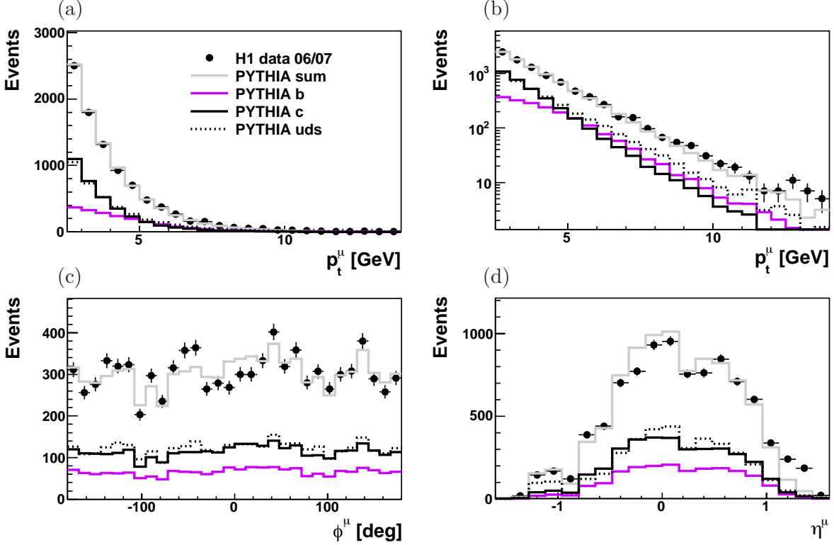
Figure 5.2: The transverse momentum p_t^\mu in (a) and (b), the azimuthal angle \phi^\mu in (c) and the pseudorapidity \eta^\mu in (d) of the selected muon candidate for data (points) and PYTHIA (lines) in comparison. All cuts discussed in this section are applied.
