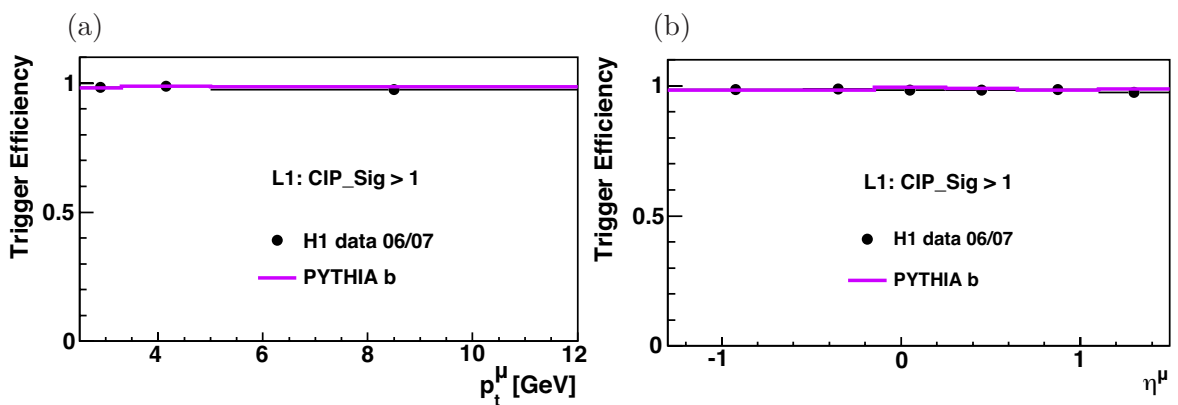
Figure 4.18: Efficiency of the z vertex trigger element CIP_Sig on L1. The data (points) shows an efficiency of nearly 100% and is compared to PYTHIA (solid line). In (a) the efficiency is plotted as a function of p_t^\mu and in (b) as a function of \eta^\mu .
