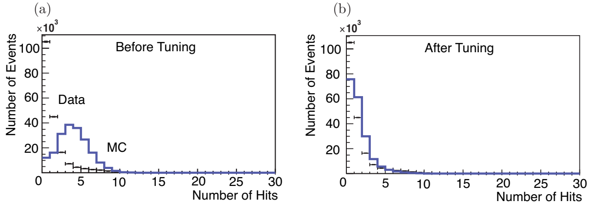
Figure 4.7: Occupancy of one half ladder side for 2006 data (points) and Monte Carlo simulation (solid line) in comparison. Figure (a) shows a very high occupancy for the untuned simulation while in (b) a good description of the data can be seen. Again, this plot is done for one of the 64 half ladders.
