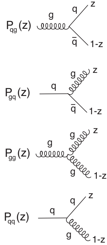
Figure 2.5: A parton evolution diagram is shown on the left (a). Figure (b) illustrates the splitting functions P_{ab}(z) .
