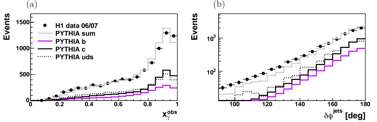
Figure 5.11: The observable x_\gamma^{obs} in (a) and \delta\phi^{jets} in (b) for data (points) and PYTHIA (lines) in comparison after all cuts.
