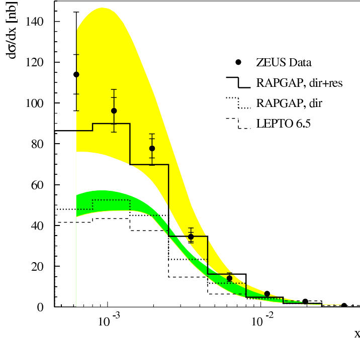
Figure 43: Forward jet cross section as a function of x . The shaded bands correspond to the factorization scale uncertainty.
