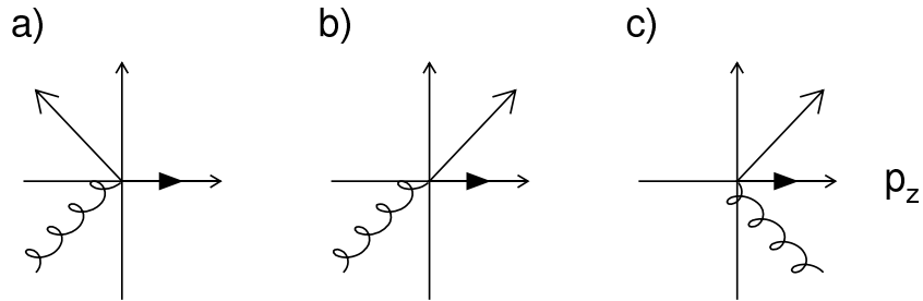
Figure 47: Possible parton configurations after absorption of the virtual photon in the Breit frame. The proton remnant points to the right.
