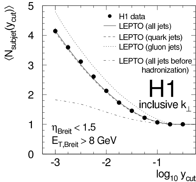
Figure 15: Mean subjet multiplicity in dijet events
