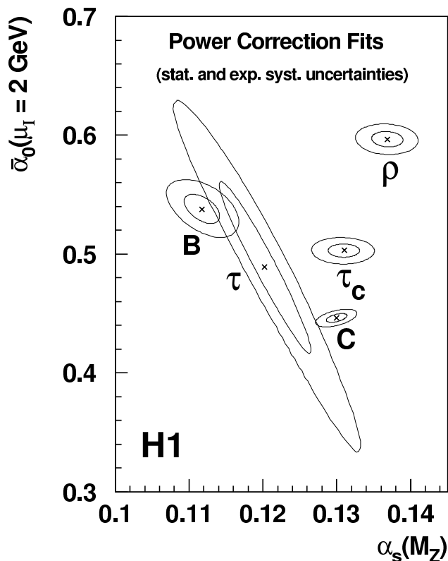
Figure 32: Values of \alpha_s(M_Z) and \bar{\alpha}_0 from power correction fits for different event shape variables. The circles correspond to the 1- \sigma and 2- \sigma contours of the experimental errors.
