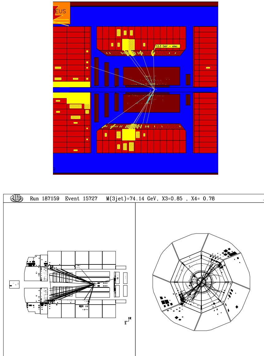
Figure 13: Neutral current DIS events with the scattered electron and two jets (top) or three jets (bottom).
