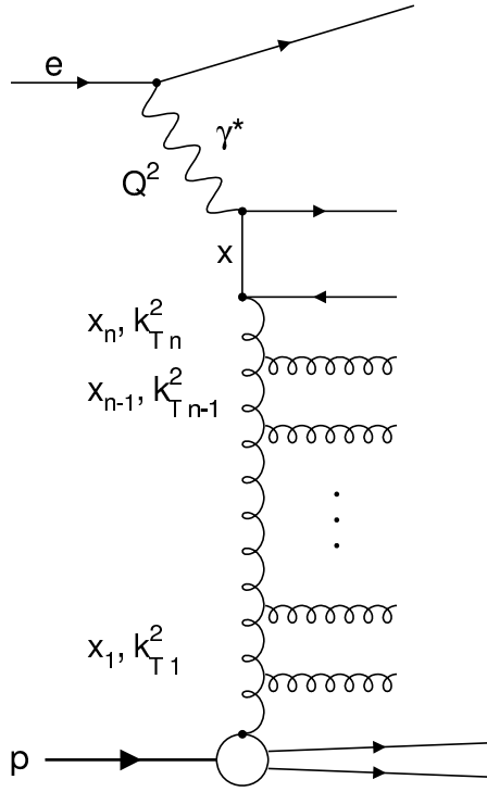
Figure 8: Ladder diagram to illustrate parton evolution.
