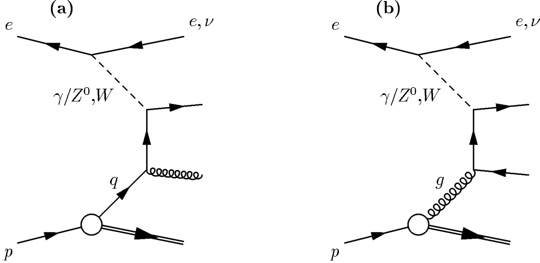
Figure 6: Feynman graphs contributing to DIS in O(\alpha_s) : QCD-Compton scattering (a) and boson-gluon-fusion (b).
