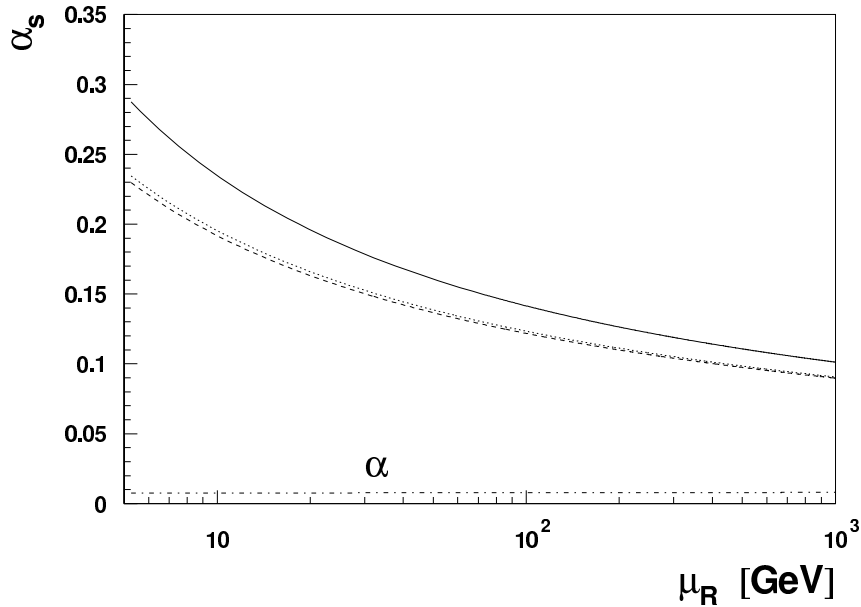
Figure 3: Running of \alpha_s in leading order (full line), NLO (dashed line) and NNLO (dotted line). The running of \alpha is also shown (dashed-dotted line).
