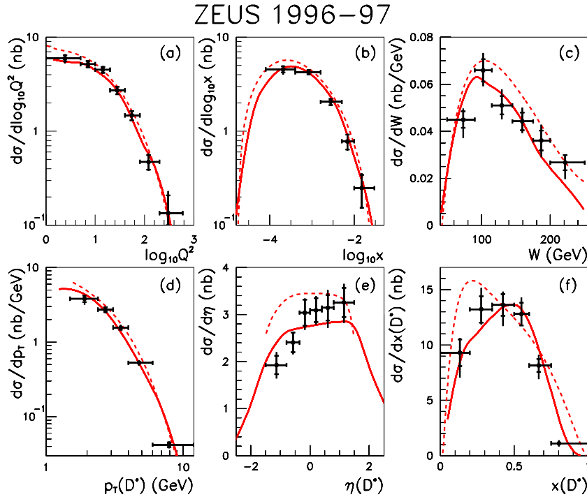
Figure 36: Differential D^* cross sections compared with NLO predictions.
