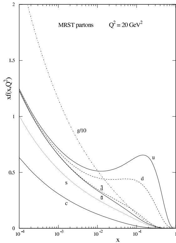
Figure 10: Example of parton density functions taken from MRST [42].
