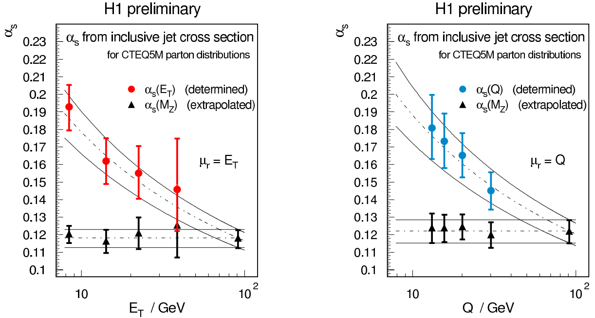
Figure 28: Renormalization scale dependence of \alpha_s for either choice of scale E_{T \text{ jet}} or Q^2 .
