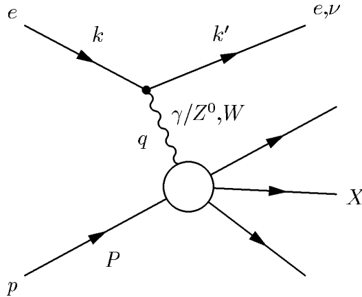
Figure 4: Illustration of deep-inelastic electron-proton scattering.
