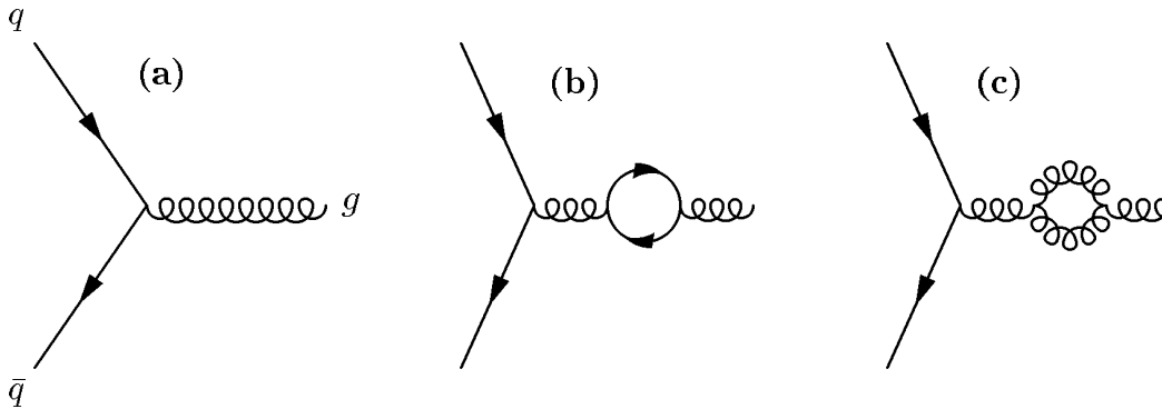
Figure 2: Feynman graphs related to the running of \alpha_s
