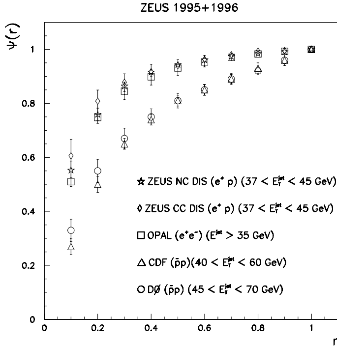
Figure 14: Jet shape distributions
