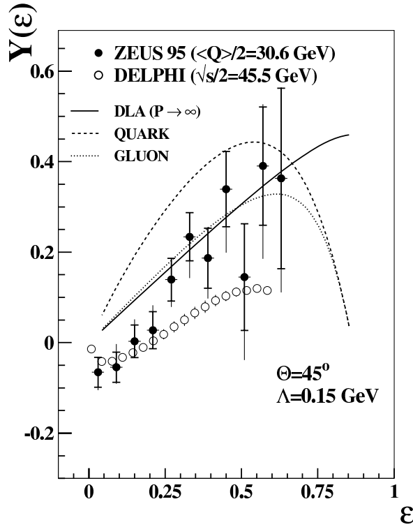
Figure 53: The correlation function Y(\epsilon) for Q^2 > 2000 \text{ GeV}^2 compared with analytical QCD predictions and results from e^+e^- annihilation.
