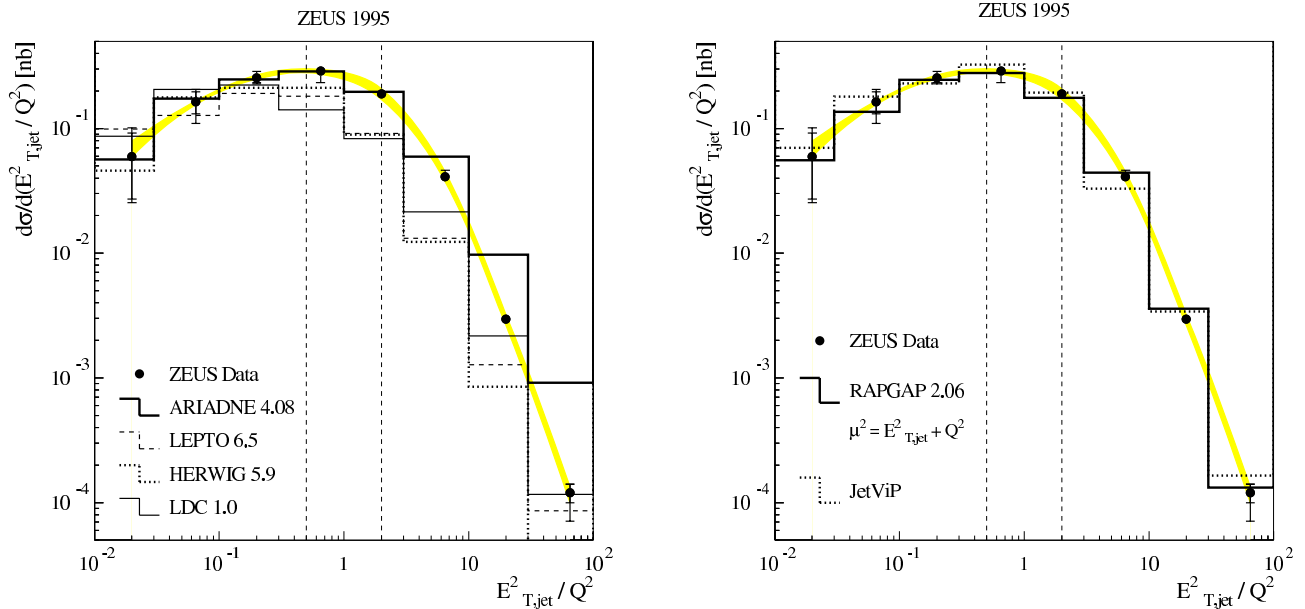
Figure 44: Forward jet cross section as a function of E_T^2 / Q^2 . The shaded bands correspond to the uncertainty of the energy scale of the calorimeter.
