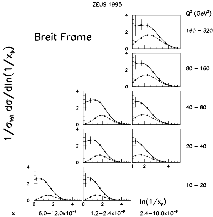
Figure 50: \ln(1/x_p) distributions for the target and current hemispheres.
