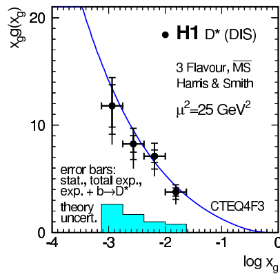
Figure 38: Gluon density from measurement of D^* cross sections.
