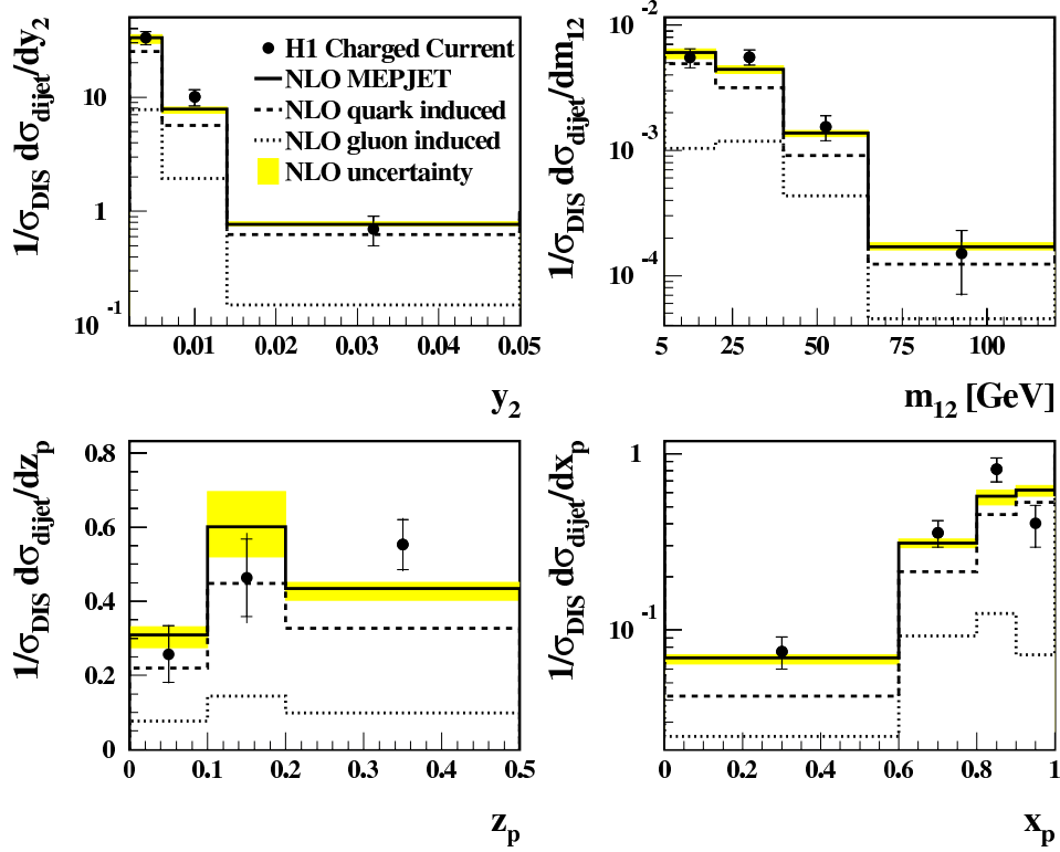
Figure 19: Dijet event distributions in CC processes at Q^2 > 640 \text{ GeV}^2 compared with perturbative QCD predictions in NLO.
