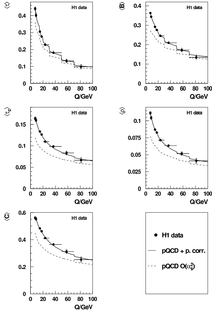
Figure 31: Mean values of event shape distributions compared with perturbative QCD calculations combined with power corrections fitted to the data.
