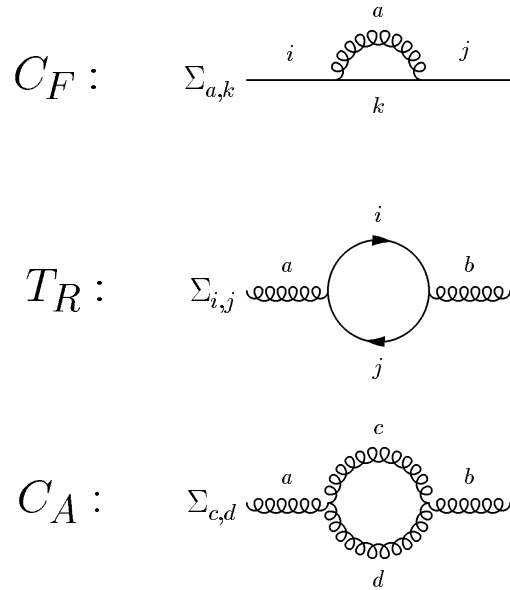
Figure 1: Illustration of the relation of colour factors C_F, T_R, C_A with gluon bremsstrahlung, gluon splitting and the three-gluon interaction.
