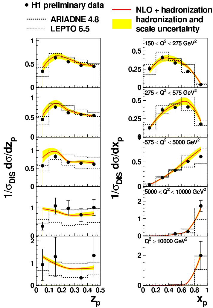
Figure 20: Dijet event distributions as a function of z_p and x_p at highest Q^2 .
