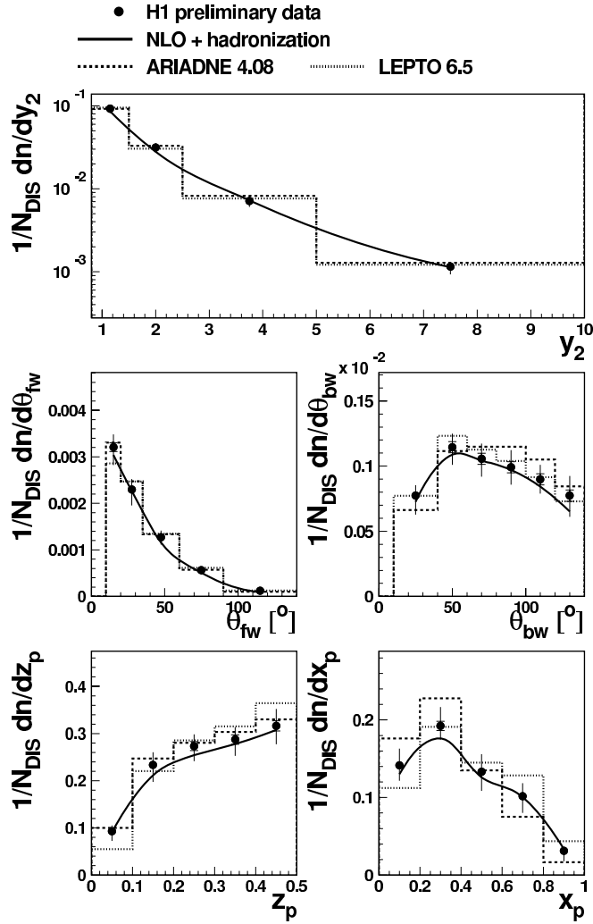
Figure 18: Dijet event distributions in NC processes at Q^2 > 150 \text{ GeV}^2 compared with the predictions of QCD models and perturbative QCD in NLO.
