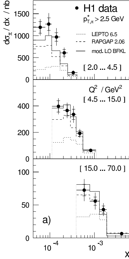
Figure 45: Inclusive forward \pi^0 cross section as a function of x in three ranges of Q^2 .
