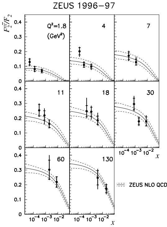
Figure 37: Ratio of F_2^{c\bar{c}} and F_2 compared with predictions based on the parton densities extracted from F_2 [133].
