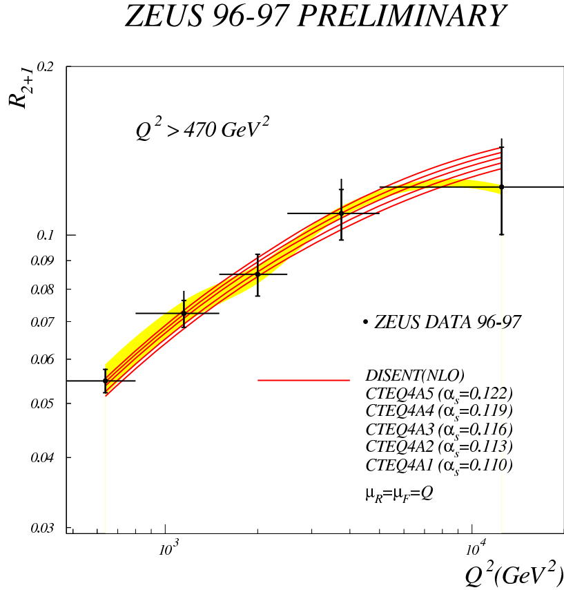
Figure 30: Dijet rate R_{2+1}(Q^2) compared with NLO predictions for the CTEQ4A PDF series.
