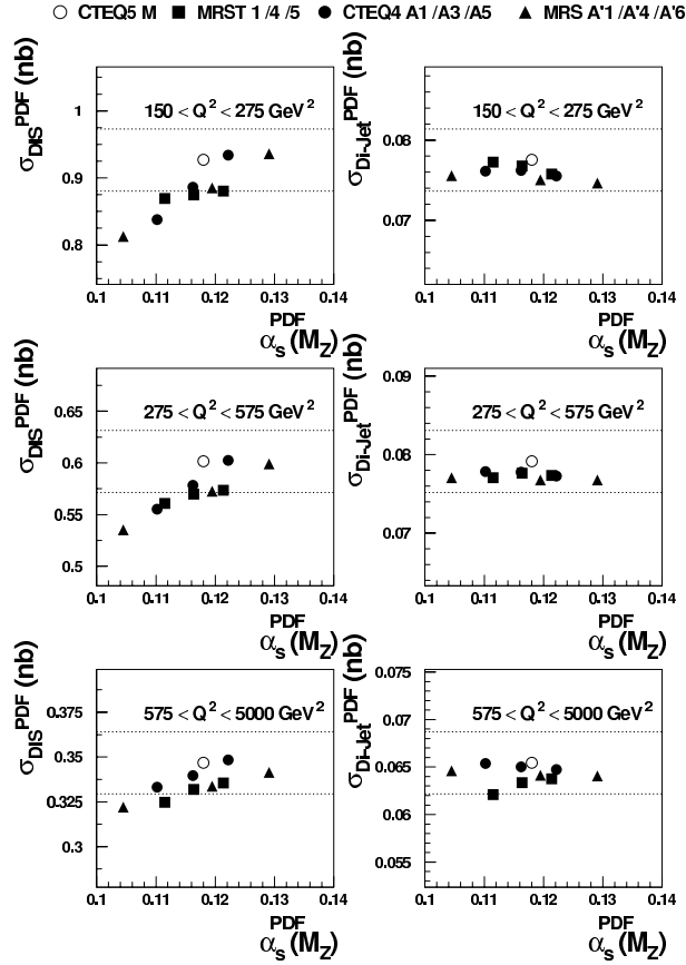
Figure 29: Inclusive DIS cross sections \sigma_{DIS} (left) and dijet cross sections \sigma_{dijet} (right) calculated in NLO for different sets of PDFs with different \alpha_s^{PDF} . The dotted horizontal lines correspond to a deviation of \pm 5\% from the CTEQ5M expectation.
