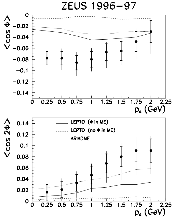
Figure 22: The mean values of \cos \phi and \cos 2\phi as a function of minimum transverse particle momentum.
