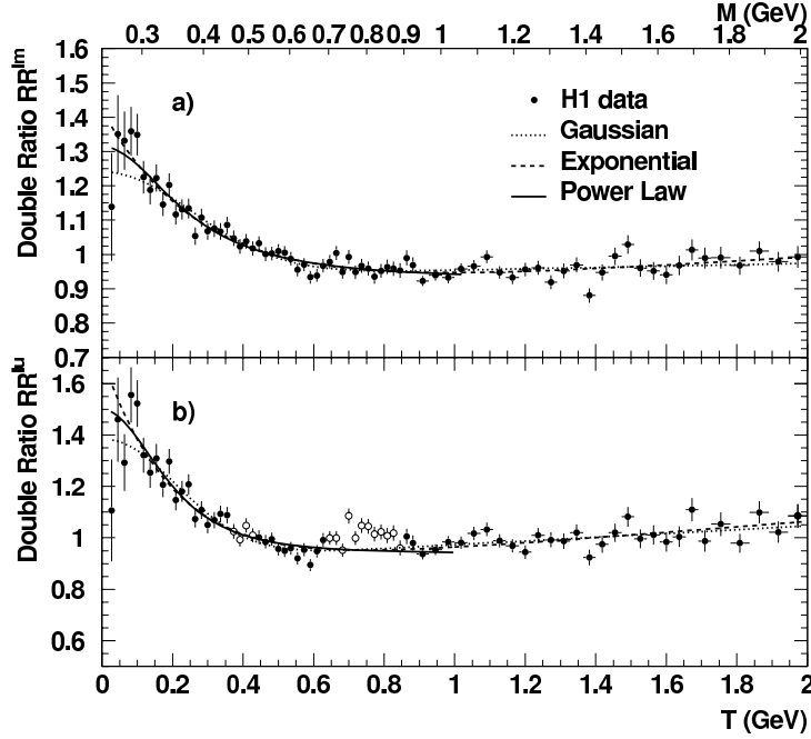
Figure 55: Bose-Einstein-correlations for reference samples based on event-mixing (top) and unlike-charge pairs (bottom) fitted to different parameterizations of the correlation function.
