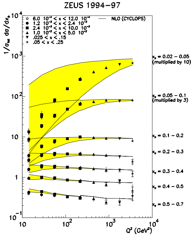
Figure 48: Fragmentation functions in the current hemisphere of the Breit frame compared with NLO predictions combined with a power correction.
