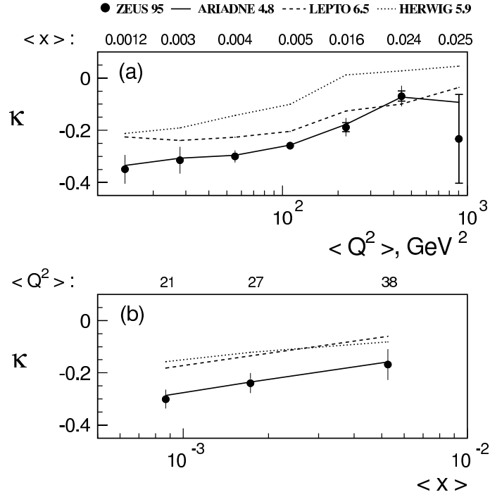
Figure 54: Multiplicity correlations between the current and target hemisphere of the Breit frame.
