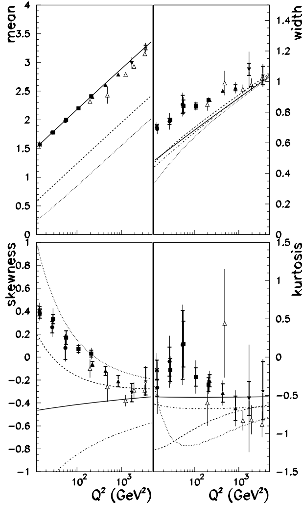
Figure 49: Q^2 dependence of mean, width and higher moments of the \xi distributions measured in the current hemisphere of the Breit frame. Also shown are fits to MLLA predictions.
