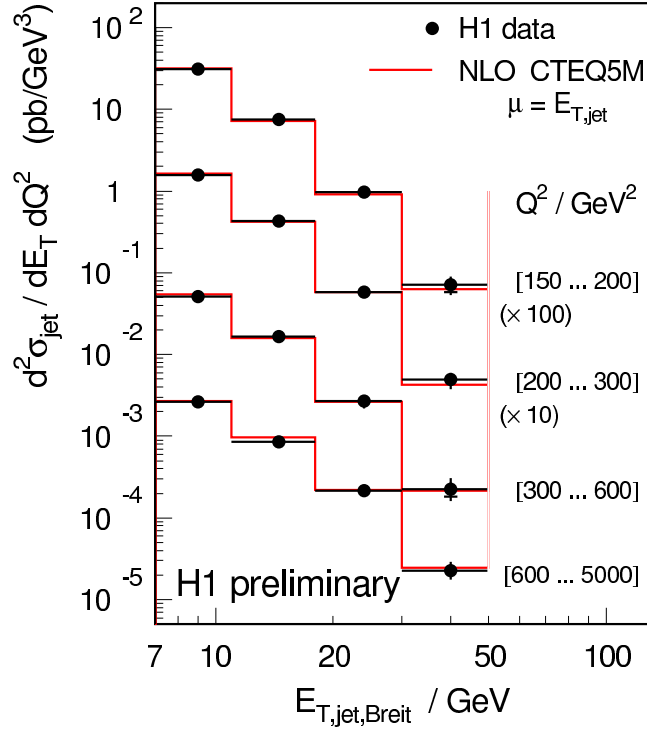
Figure 26: Inclusive jet cross sections as a function of E_{T,jet}^{Breit} for different values of Q^2 .
