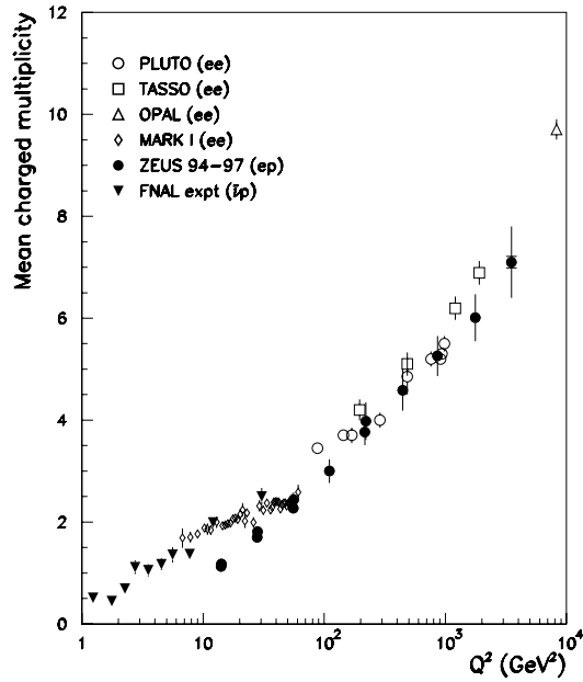
Figure 46: Mean charged particle multiplicity in the current hemisphere of the Breit frame. Measurements from e^+e^- annihilation and fixed-target DIS are also shown.
