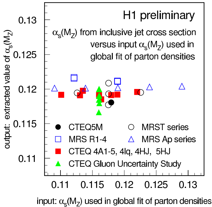
Figure 27: Correlation of \alpha_s^{fit} with \alpha_s^{PDF} .
