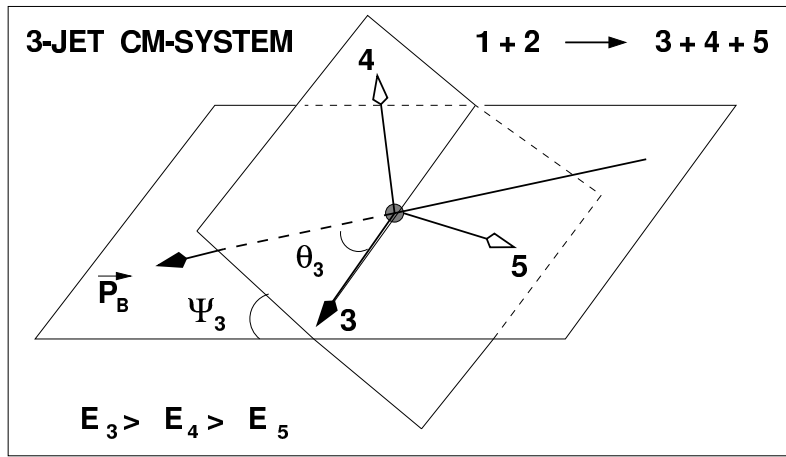
Figure 23: Definition of three-jet variables in the jet centre-of-mass system.
