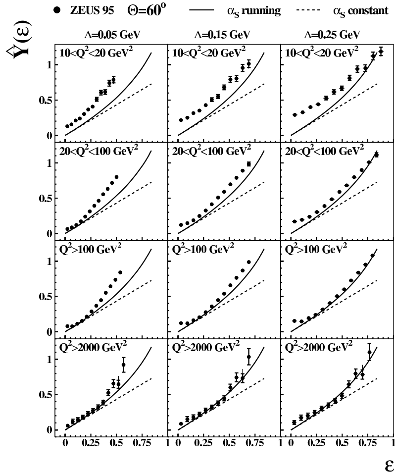
Figure 52: The normalized two-particle density \hat{Y}(\epsilon) compared with analytical QCD predictions in the DLA.
