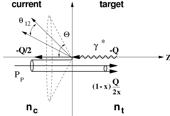
Figure 51: Illustration of the correlations between particles in a cone of opening angle \Theta separated by the angle \theta_{12} in the current hemisphere of the Breit frame.
