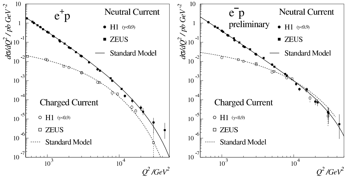
Figure 5: NC and CC differential cross sections d\sigma/dQ^2 for e^+p and e^-p DIS as measured by H1 [28, 29] and ZEUS [30, 31].
