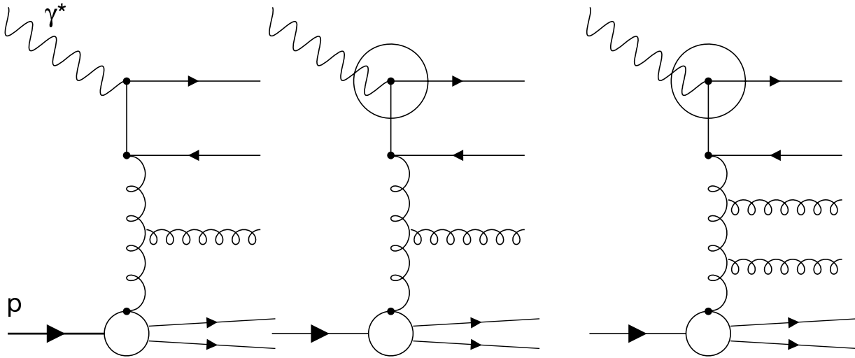
Figure 41: NLO diagram without photon structure \gamma^*g \rightarrow q\bar{q}g (left), LO diagram with photon structure \bar{q}g \rightarrow \bar{q}g (middle) and NLO diagram with photon structure \bar{q}g \rightarrow \bar{q}gg (right).
