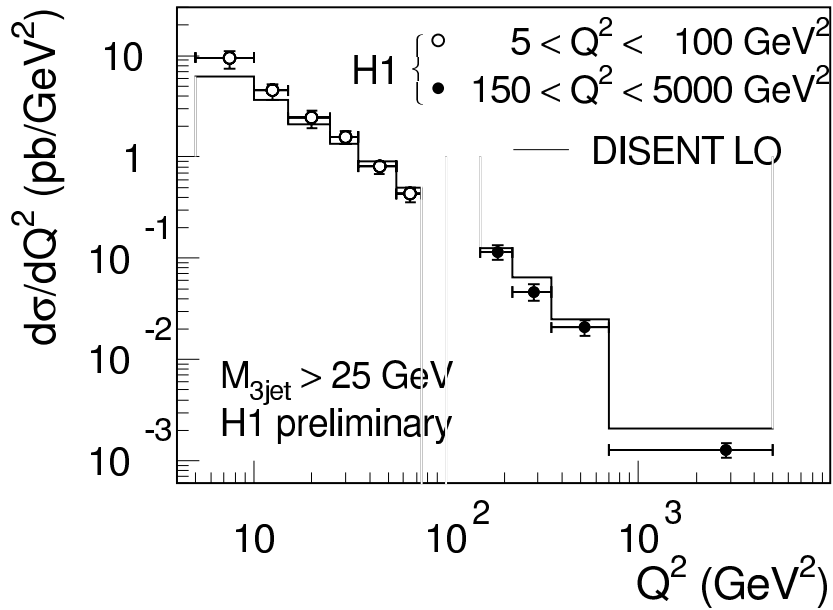
Figure 24: Three-jet cross section d\sigma/dQ^2 in the range of 5 < Q^2 < 5000 \text{ GeV}^2 compared with perturbative QCD calculations in LO. Hadronization corrections are not applied. They lower the QCD prediction by 20-40%.
