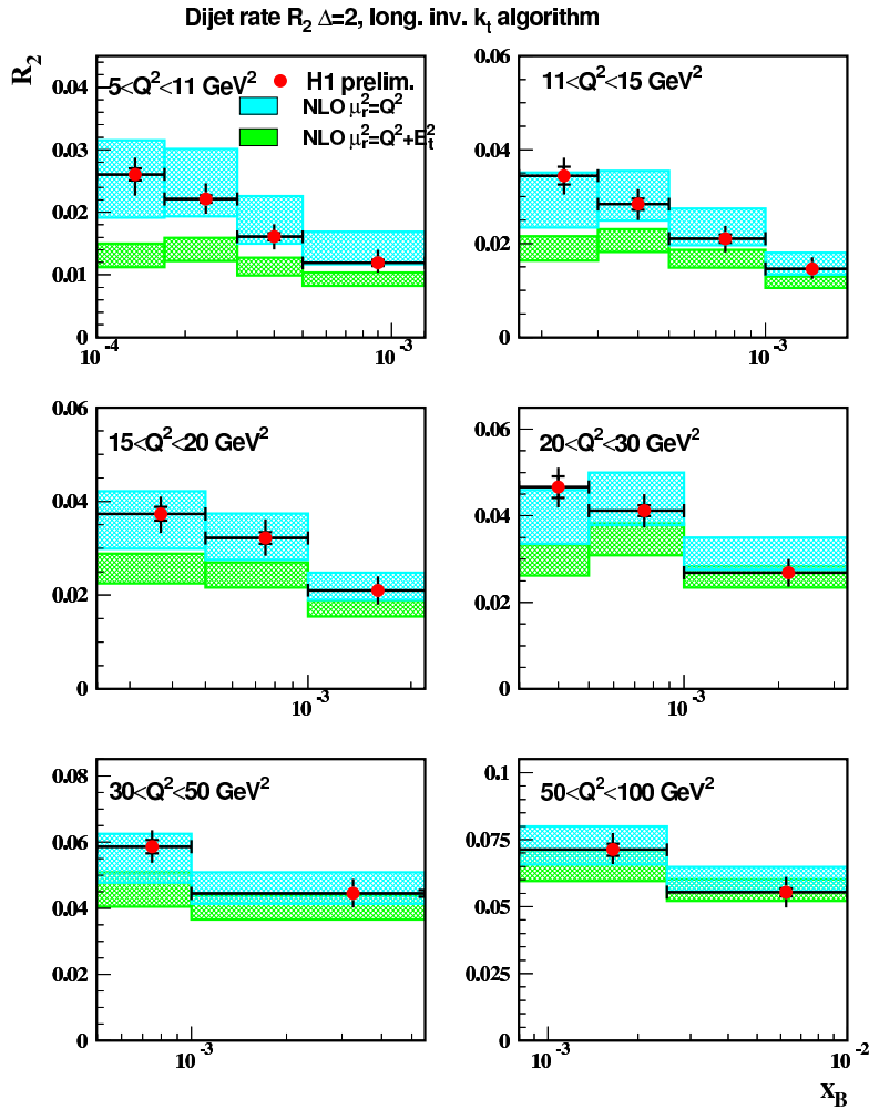
Figure 17: Dijet event rate R_2(x) in the range 5 < Q^2 < 100 \text{ GeV}^2 compared with QCD predictions in NLO.
