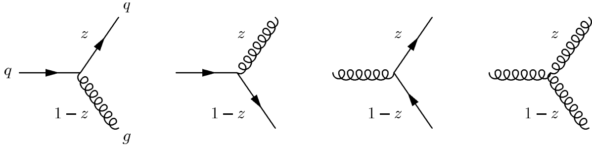
Figure 7: Vertices corresponding to the splitting functions P_{qq} , P_{gq} , P_{qg} and P_{gg} (from left to right).
