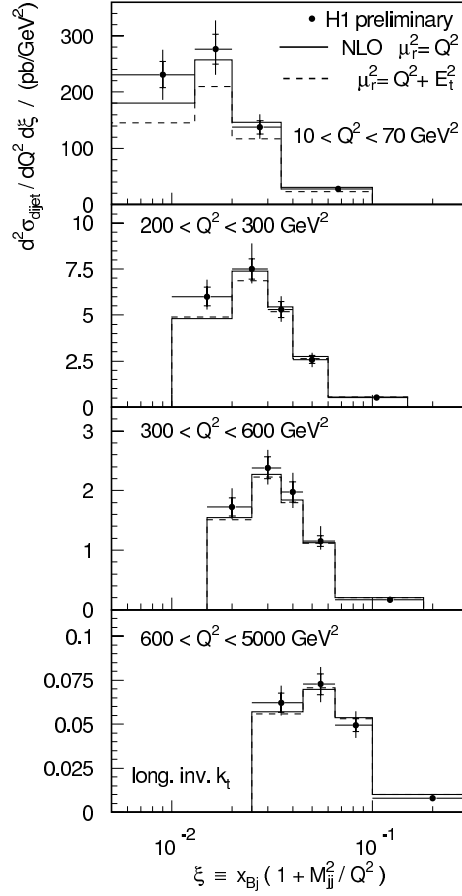
Figure 33: Dijet cross section d^2\sigma/dQ^2 d\xi compared with QCD predictions in NLO.
