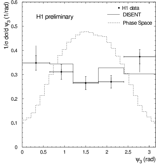
Figure 25: Three-jet distribution of \Psi_3 in the range 5 < Q^2 < 100 \text{ GeV}^2 compared with a perturbative QCD calculation in LO and a phase space prediction. Hadronization corrections are not applied.
