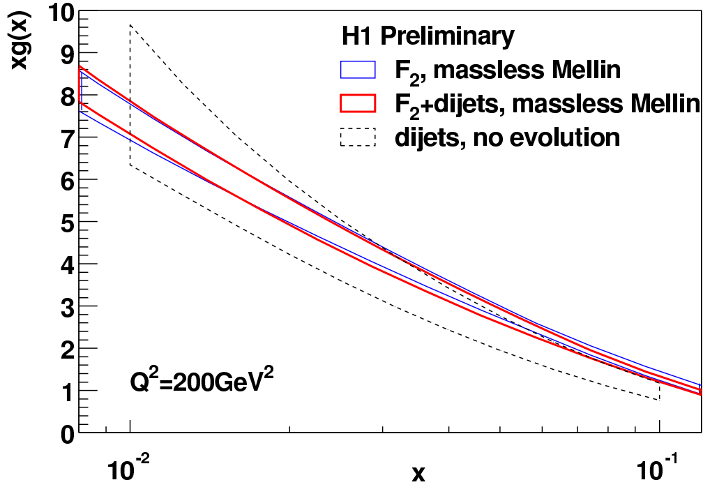
Figure 34: Gluon density at large momentum fractions determined using dijet and F_2 measurements.
