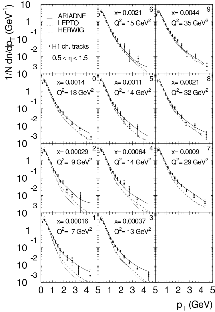
Figure 39: Charged particle transverse momentum spectra in different ranges of Q^2 and x .
