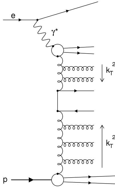
Figure 9: Diagram illustrating the effect of unordered k_T introduced through a resolved photon.
