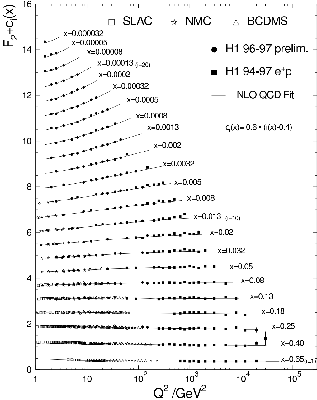
Figure 11: Overview of F_2 measurements of H1 [43, 28] and fixed target experiments [24, 25, 27] and comparison with perturbative QCD predictions in NLO [28].
