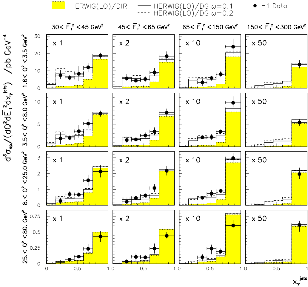
Figure 42: Triple differential dijet cross sections at low Q^2
