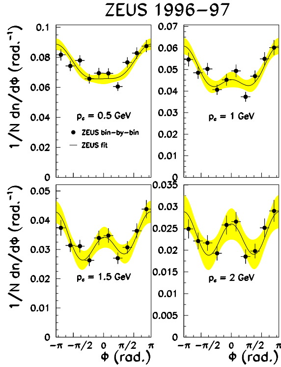
Figure 21: Azimuthal distribution of the leading charged particles for different requirements on the minimum transverse particle momentum p_c in the hadronic centre-of-mass frame.
