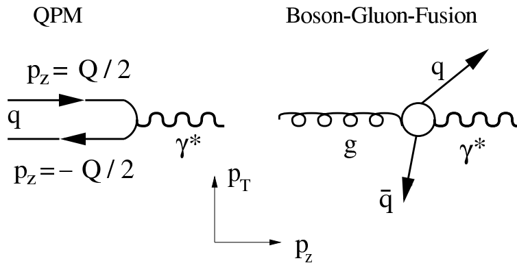
Figure 12: Illustration of the scattering process as seen in the Breit frame for quark scattering in the QPM and boson-gluon-fusion.
