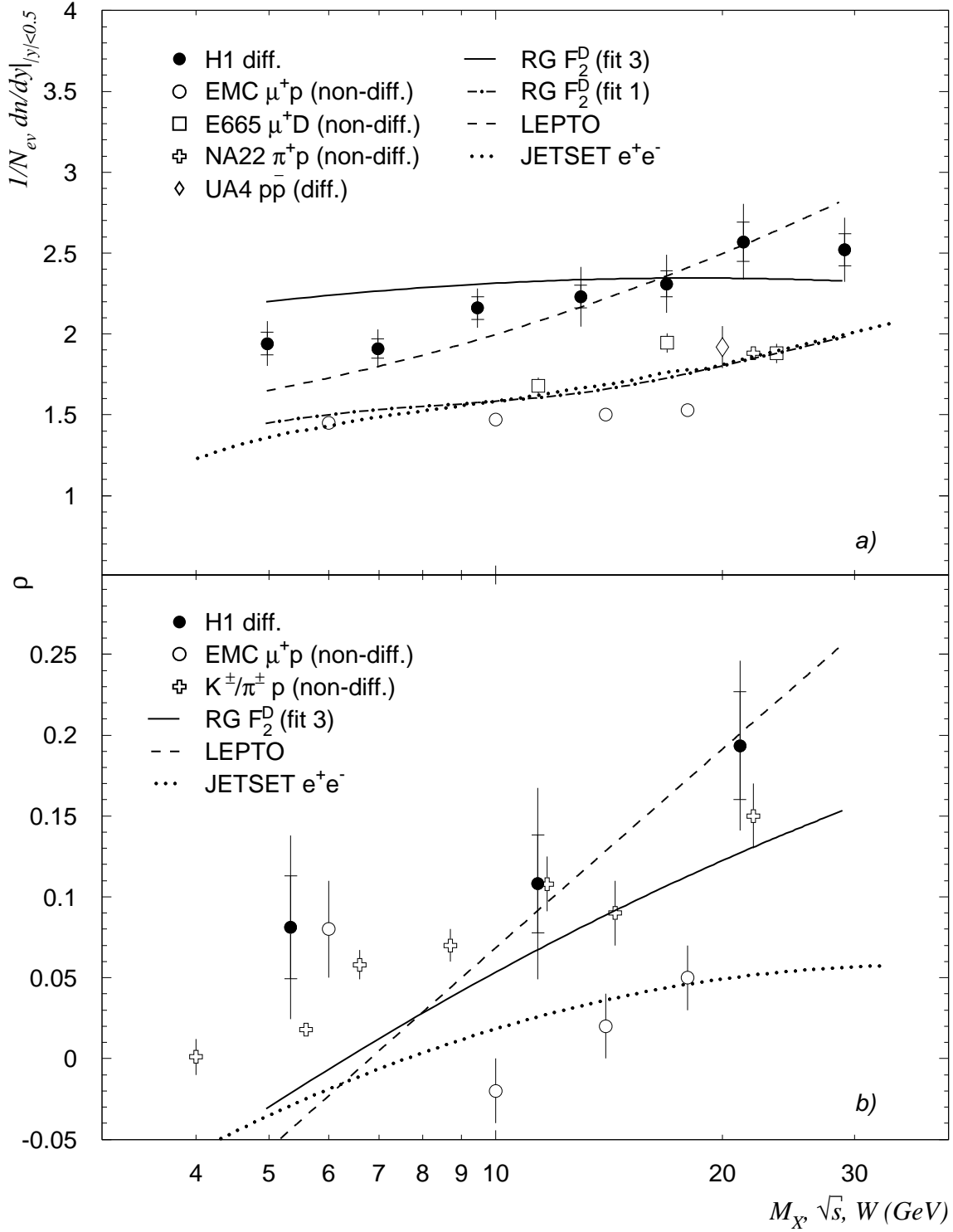
Figure 4: (a) Central region charged particle density ( -0.5 < y < 0.5 ); (b) The parameter \rho (H1) and b (others), which reflects the correlation between the number of particles in the forward and backward hemispheres, as a function of M_X (H1), W = \langle M_X \rangle ( \mu p ), M_X (hadron diffraction), \sqrt{s} (non-diffractive hadron-hadron), \sqrt{s} (JETSET e^+e^- ). Also shown are predictions of several DIS Monte Carlo models (see text).
