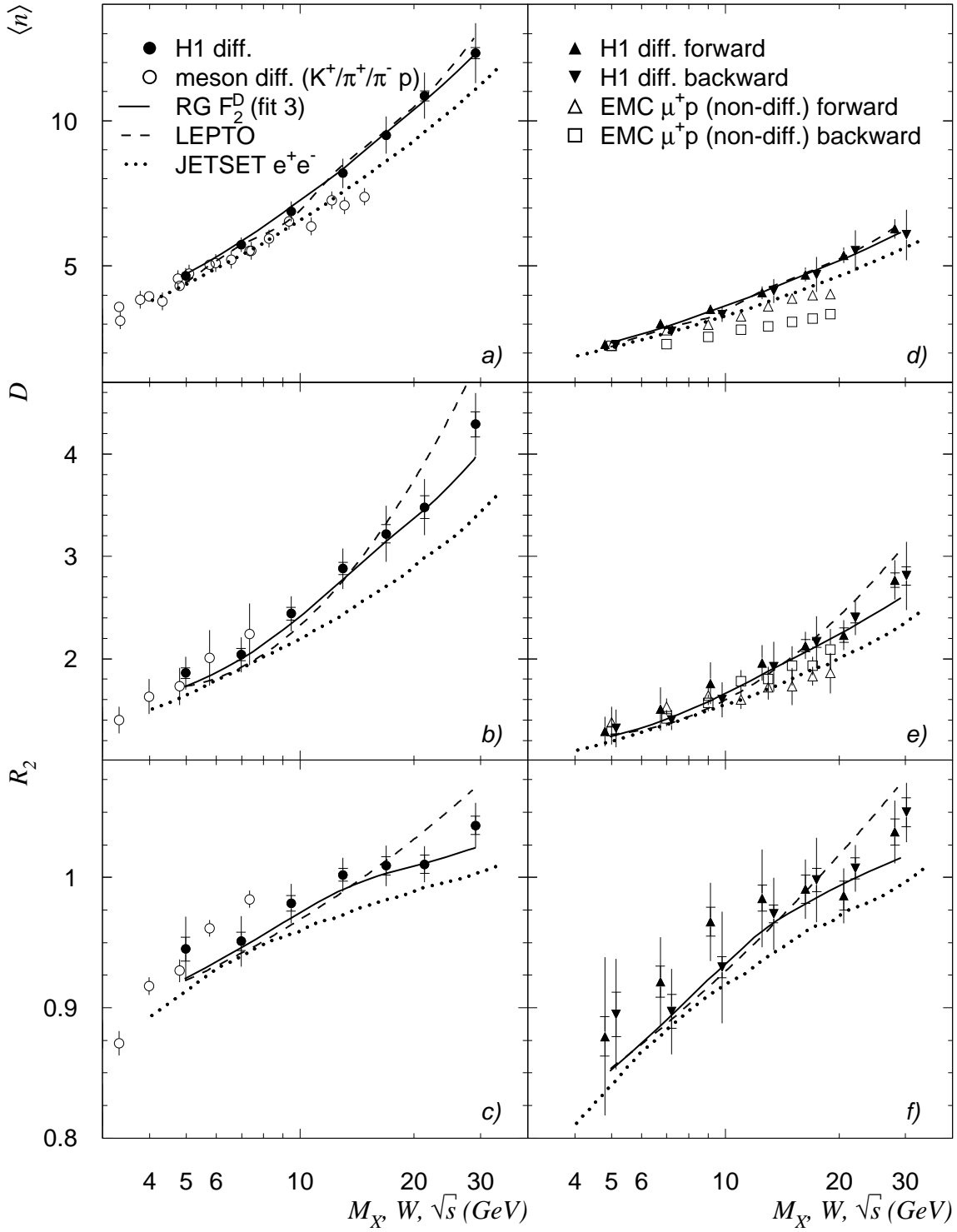
Figure 1: Multiplicity moments \langle n \rangle , D and R_2 in full phase space (a-c) and in single hemispheres (d-f) for charged hadrons as a function of M_X (H1), M_X (meson diffraction), W (EMC), \sqrt{s} ( e^+e^- ), respectively. For clarity, H1 data points in single hemispheres are slightly shifted in the horizontal direction with respect to their true positions. Also shown are predictions of several Monte Carlo models (see text). The Monte Carlo curves in forward and backward hemispheres are symmetric and their average is plotted.
