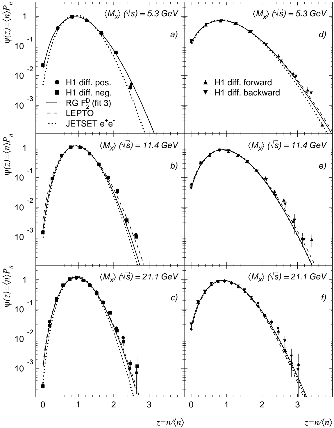
Figure 2: The multiplicity distribution in KNO form for three intervals in M_X (DIS data and Monte Carlo) and at \sqrt{s} = \langle M_X \rangle (JETSET e^+e^- ), in full phase space for positive and negative particles separately ( a-c ), and for all charges in single hemispheres ( d-f ). The error bars show statistical errors only. Also shown are predictions of several Monte Carlo models (see text). The Monte Carlo curves are charge and forward-backward symmetric and their average is plotted.
