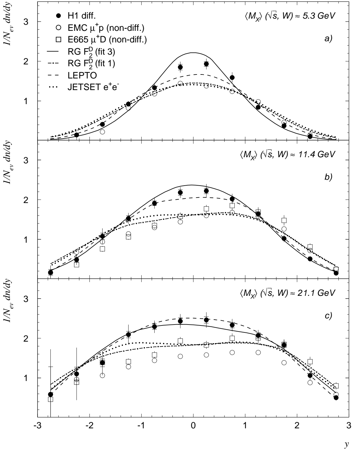
Figure 3: Charged particle rapidity spectra for three intervals in M_X (H1), at W = \langle M_X \rangle ( \mu N ) and at \sqrt{s} = \langle M_X \rangle (JETSET e^+e^- ). The \langle W \rangle values for EMC and E665 differ slightly from the ones indicated for H1 and are equal to 5.2, 11 and 19 GeV and 11.4 and 23.6 GeV, respectively. Also shown are predictions of several Monte Carlo models (see text).
