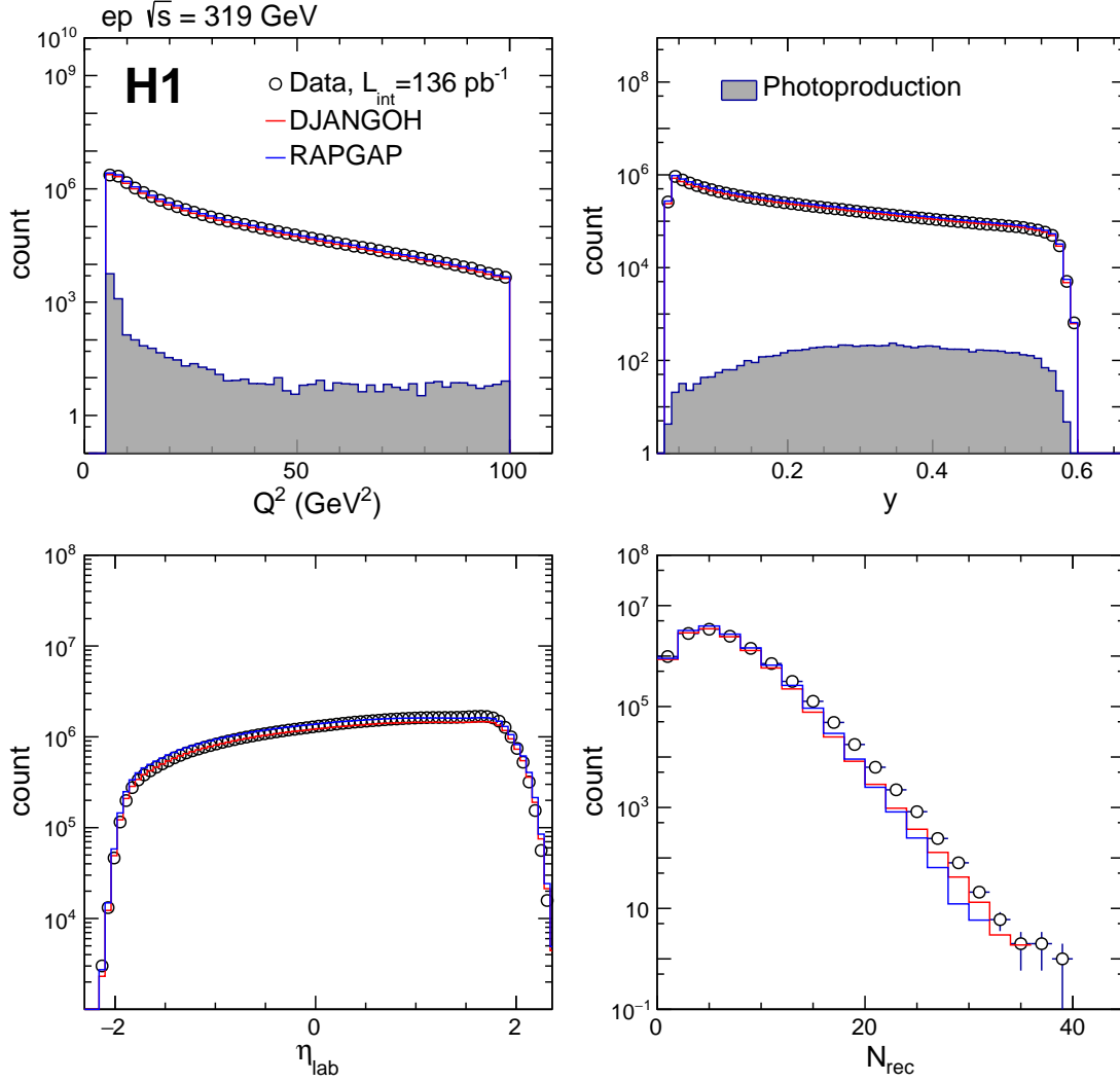
Figure 1: Reconstructed momentum transfer Q^2 , inelasticity y , pseudorapidity \eta_{\text{lab}} , and charged particle multiplicity N_{\text{rec}} for data (open circle), and the DJANGO (red line) and the RAPGAP (blue line) MC models. The phase space restrictions are given in Table 1. The photoproduction background simulated from PYTHIA 6.4 [54] is shown for the Q^2 and y distributions. Error bars indicate the statistical uncertainty of data.
