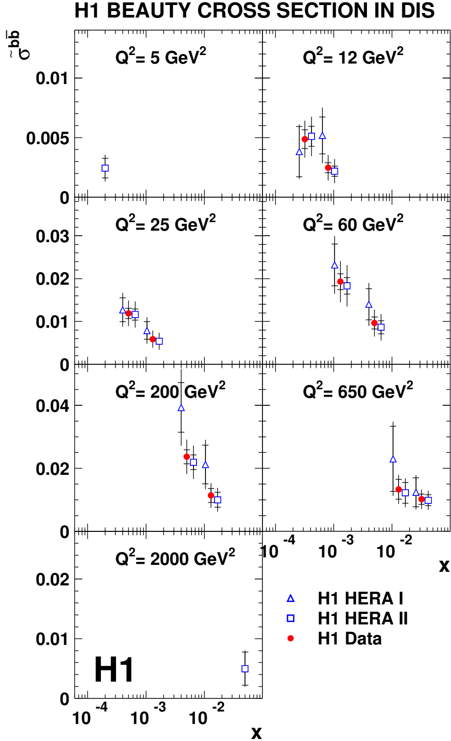
Figure 12: The measured reduced cross section \tilde{\sigma}^{b\bar{b}} shown as a function of x for different Q^2 values. The inner error bars show the statistical error, the outer error bars represent the statistical and systematic errors added in quadrature. The HERA II measurements are compared with those from HERA I. The combined H1 data are also shown. The x values of the HERA I and HERA II data are shifted for visual clarity.
