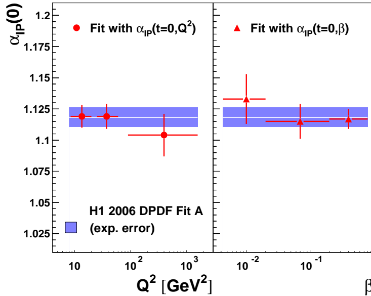
Figure 14: Results from modified versions of the ‘H1 2006 DPDF Fit A’ in which additional free parameters are included, corresponding to the value of \alpha_{\mathbb{P}}(0) in a number of different ranges of Q^2 (left) or \beta (right). The data points correspond to the results for \alpha_{\mathbb{P}}(0) in each interval of Q^2 or \beta , with error bars corresponding to the full experimental uncertainties. The bands show the result and experimental uncertainty from the standard fit in which a single parameter is used for \alpha_{\mathbb{P}}(0) .
