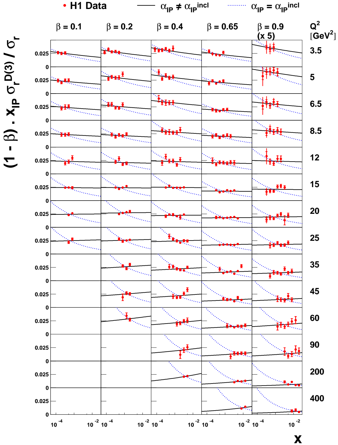
Figure 19: The ratio of the diffractive to the inclusive reduced cross section, multiplied by (1 - \beta) x_{\text{P}} . Data at \beta = 0.9 are multiplied by a further factor of 5 for visibility. Data which are significantly influenced by the sub-leading exchange or the longitudinal structure function according to the NLO QCD fit are excluded. The remaining data are compared with models motivated by Regge phenomenology as described in the text, for which the diffractive and inclusive effective pomeron trajectories are the same ( \alpha_{\text{P}} = \alpha_{\text{P}}^{\text{incl}} ) and for which they are different ( \alpha_{\text{P}} \neq \alpha_{\text{P}}^{\text{incl}} ).
