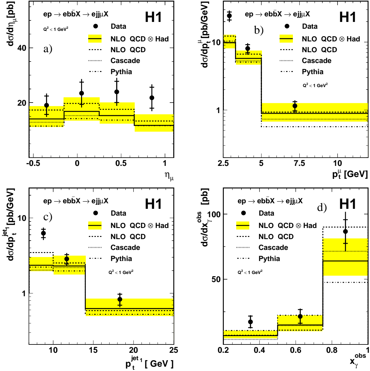
Figure 8: Differential cross sections for the photoproduction process ep \rightarrow ebb\bar{X} \rightarrow ejj\mu X' in the kinematic range Q^2 < 1 \text{ GeV}^2 , 0.2 < y < 0.8 , p_t^\mu > 2.5 \text{ GeV} , -0.55 < \eta^\mu < 1.1 , p_t^{jet1(2)} > 7(6) \text{ GeV} and |\eta^{jet}| < 2.5 . The cross sections are shown as functions of a) the muon pseudo-rapidity \eta^\mu , b) the muon transverse momentum p_t^\mu , c) the jet transverse momentum p_t^{jet1} of the highest transverse momentum jet and d) the quantity x_\gamma^{obs} . The inner error bars show the statistical error, the outer error bars represent the statistical and systematic uncertainties added in quadrature. The NLO QCD predictions at the parton level (dashed line) are corrected to the hadron level (solid line) using the PYTHIA generator. The shaded band around the hadron level prediction indicates the systematic uncertainties as estimated from scale variations (see text). Predictions from the Monte Carlo generator programs CASCADE (dotted line) and PYTHIA (dash-dotted line) are also shown.
