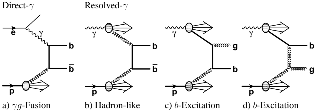
Figure 1: Beauty production processes in leading order pQCD.
