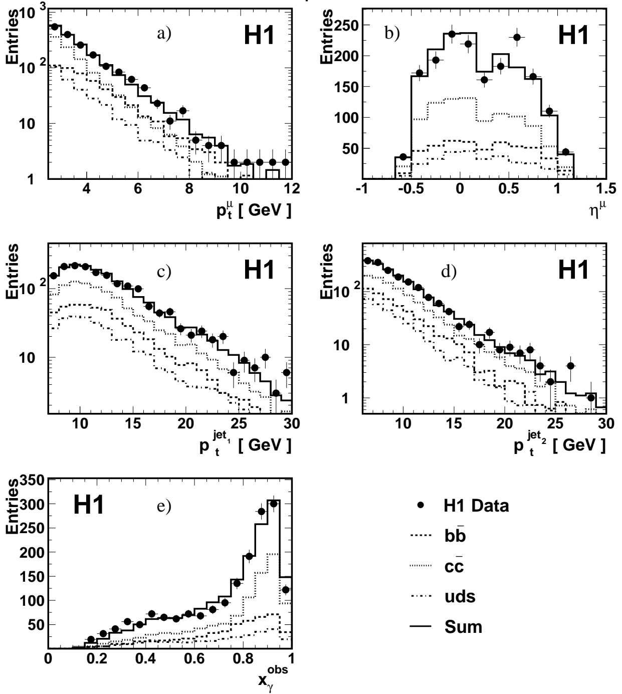
Figure 2: Distributions in photoproduction of a) the muon transverse momentum p_t^\mu , b) the pseudo-rapidity of the muon \eta^\mu , c) and d) the transverse momenta p_t^{\text{jet}_{1(2)}} of the highest and the second-highest p_t jets, respectively and e) the observable x_\gamma^{\text{obs}} . Included in the figure are the estimated contributions of events arising from b quarks (dashed line), c quarks (dotted line) and light quarks (dash-dotted line). The shapes of the distributions from the different sources are taken from the PYTHIA Monte Carlo simulation and their relative fractions are determined from a fit to the two-dimensional data distribution of p_t^{\text{rel}} and \delta (see text).
