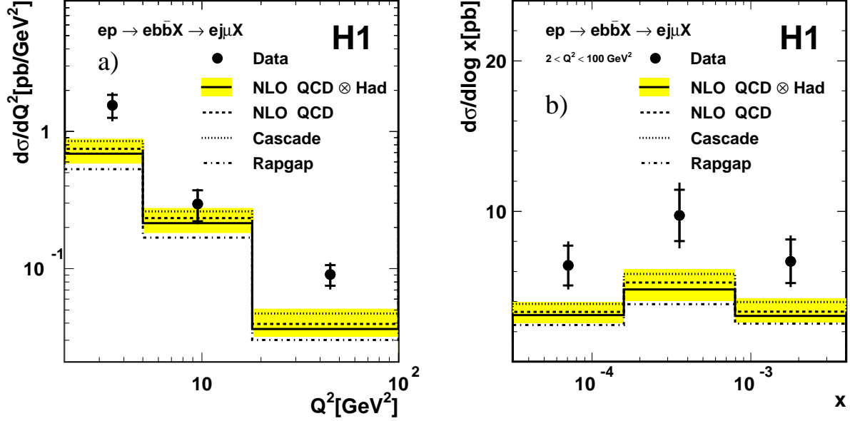
Figure 9: Differential cross sections for the electroproduction process ep \rightarrow ebb\bar{X} \rightarrow ej\mu X' in the kinematic range 2 < Q^2 < 100 \text{ GeV}^2 , 0.1 < y < 0.7 , p_t^\mu > 2.5 \text{ GeV} , -0.75 < \eta^\mu < 1.15 , p_{t,jet}^{Breit} > 6 \text{ GeV} and |\eta^{jet}| < 2.5 . The cross sections are shown as functions of a) the photon virtuality Q^2 and b) the Bjorken scaling variable x . The inner error bars show the statistical error, the outer error bars represent the statistical and systematic uncertainties added in quadrature. NLO QCD predictions at the parton level (dashed line) are corrected to the hadron level (solid line) using the RAPGAP generator. The shaded band around the hadron level prediction indicates the systematic uncertainty as estimated from scale variations (see text). Predictions from the Monte Carlo generator programs CASCADE (dotted line) and RAPGAP (dash-dotted line) are also shown.
