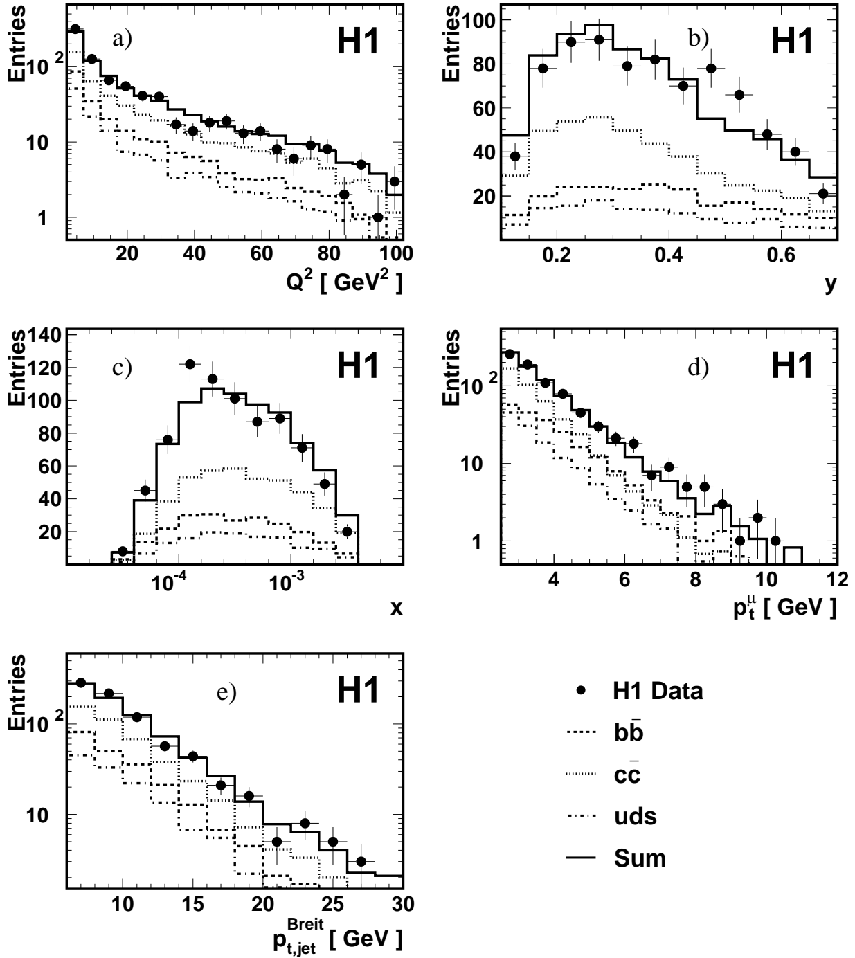
Figure 3: Distributions in electroproduction of a) the photon virtuality Q^2 , b) the inelasticity y , c) Bjorken x , d) the muon transverse momentum and e) the transverse momentum p_{t,jet}^{Breit} of the selected jet in the Breit frame. Included in the figure are the estimated contributions of events arising from b quarks (dashed line), c quarks (dotted line) and light quarks (dash-dotted line). The shapes of the distributions from the different sources are taken from the RAPGAP Monte Carlo simulation and their relative fractions are determined from a fit to the two-dimensional data distribution of p_t^{rel} and \delta (see text).
