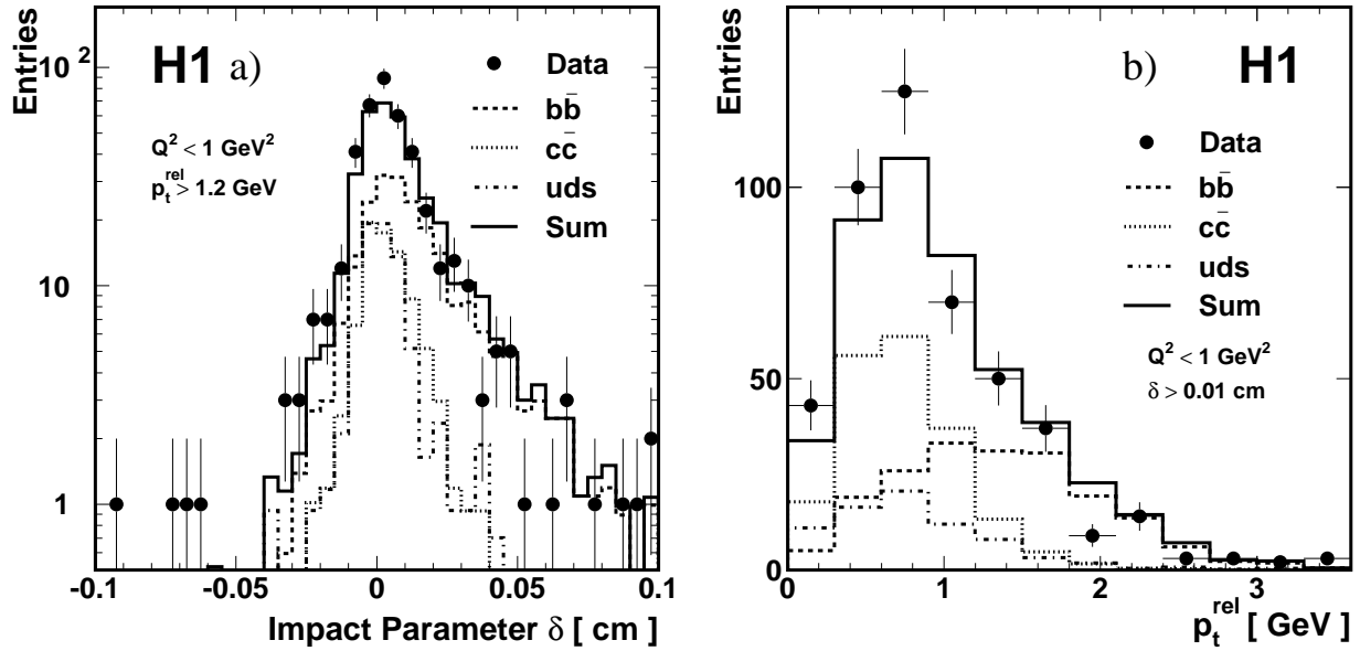
Figure 6: Distributions in the restricted photoproduction sample of a) the impact parameter \delta for events with p_t^{\text{rel}} > 1.2 \text{ GeV} and b) the transverse muon momentum p_t^{\text{rel}} relative to the jet axis for tracks with impact parameter \delta > 0.01 \text{ cm} . The predictions for the contributions to the restricted sample from b events (dashed line), c events (dotted line) and light quark events (dash-dotted line), as determined from a fit to the two-dimensional distribution of p_t^{\text{rel}} and \delta in the full data sample (see text), are also shown.
