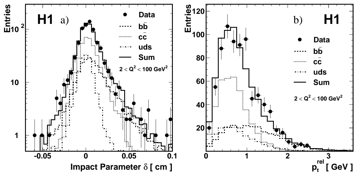
Figure 5: Distributions in electroproduction of a) the impact parameter \delta of the muon track and b) the transverse muon momentum p_t^{rel} relative to the axis of the associated jet. Included in the figure are the estimated contributions of events arising from b quarks (dashed line), c quarks (dotted line) and the light quarks (dash-dotted line). The shapes of the distributions of the different sources are taken from the RAPGAP Monte Carlo simulation and their relative fractions are determined from a fit to the two-dimensional data distribution of p_t^{rel} and \delta (see text).
