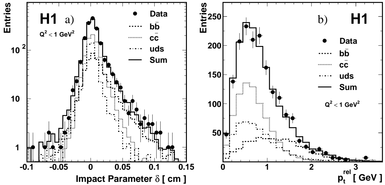
Figure 4: Distributions in photoproduction of a) the impact parameter \delta of the muon track and b) the transverse muon momentum p_t^{\text{rel}} relative to the axis of the associated jet. Included in the figure are the estimated contributions of events arising from b quarks (dashed line), c quarks (dotted line) and the light quarks (dash-dotted line). The shapes of the distributions of the different sources are taken from the PYTHIA Monte Carlo simulation and their relative fractions are determined from a fit to the two-dimensional data distribution of p_t^{\text{rel}} and \delta (see text).
