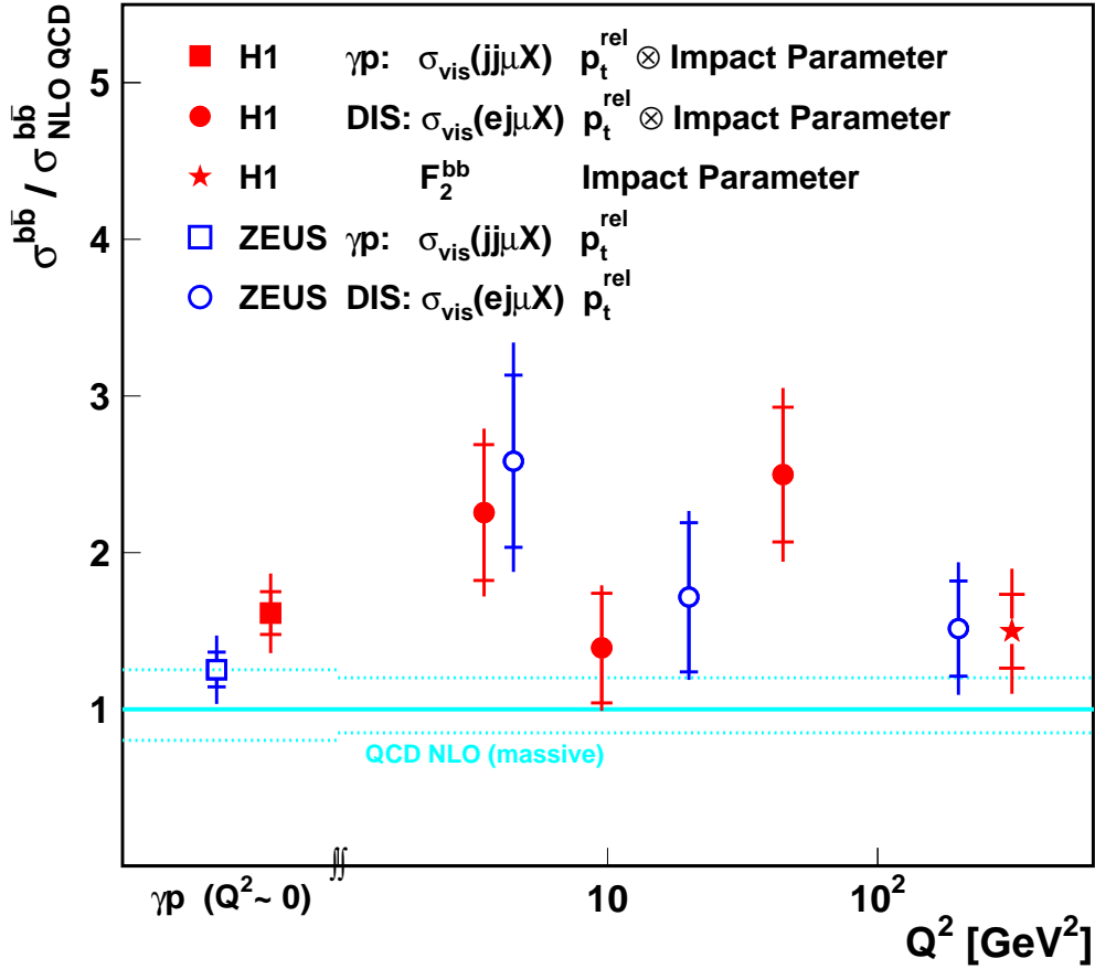
Figure 11: Ratio of beauty production cross section measurements at HERA to NLO QCD predictions. The results of this paper (solid circles and squares) are compared with ratios determined using the measurements taken from [5–7]. The photoproduction points are plotted at different horizontal positions for better visibility. Note that cross section definitions and kinematic ranges are somewhat different for the different data points. The dotted lines indicate the typical theoretical error due to scale uncertainties. The theoretical prediction used to form the ratio with the measurement by the ZEUS Experiment [6], shown as an open square, is calculated using the same program and parameter choices as for the prediction for this measurement (full square). Different parameter choices, e.g. for the modelling of the hadronisation and decay of the B -hadron, lead to a variation of the prediction of \sim 10\% .
