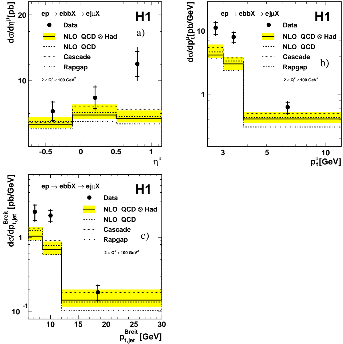
Figure 10: Differential cross sections for the electroproduction process ep \rightarrow ebb\bar{X} \rightarrow ej\mu X' in the kinematic range 2 < Q^2 < 100 \text{ GeV}^2 , 0.1 < y < 0.7 , p_t^\mu > 2.5 \text{ GeV} , -0.75 < \eta^\mu < 1.15 , p_{t,jet}^{Breit} > 6 \text{ GeV} and |\eta^{jet}| < 2.5 . The cross sections are shown as functions of a) the muon pseudo-rapidity \eta^\mu , b) the muon transverse momentum p_t^\mu and c) the transverse momentum p_{t,jet}^{Breit} of the leading jet in the Breit frame. The inner error bars show the statistical error, the outer error bars represent the statistical and systematic uncertainties added in quadrature. The NLO QCD predictions at the parton level (dashed line) are corrected to the hadron level (solid line) using the RAPGAP generator. The shaded band around the hadron level prediction indicates the systematic uncertainty as estimated from scale variations (see text). Predictions from the Monte Carlo generator programs CASCADE (dotted line) and RAPGAP (dash-dotted line) are also shown.
