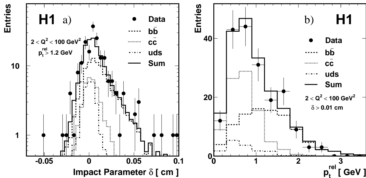
Figure 7: Distributions in the restricted electroproduction sample of a) the impact parameter \delta for events with p_t^{rel} > 1.2 GeV and b) the transverse muon momentum p_t^{rel} relative to the jet axis for tracks with impact parameter \delta > 0.01 cm. The predictions for the contributions to the restricted sample from b events (dashed line), c events (dotted line) and light quark events (dash-dotted line), as determined from a fit to the two-dimensional distribution of p_t^{rel} and \delta in the full data sample (see text), are also shown.
