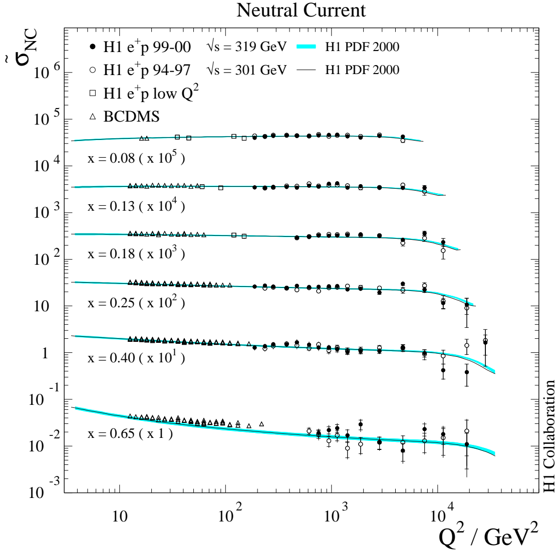
Figure 11: The NC reduced cross section \bar{\sigma}_{NC}(x, Q^2) , shown for the new e^+p (solid points) and previously published 94 – 97 e^+p (open points) data. The results are compared with the corresponding Standard Model expectations determined from the H1 PDF 2000 fit at \sqrt{s} = 319 GeV (error bands) and \sqrt{s} = 301 GeV (full curves), respectively. Also shown are data from H1 measured at lower Q^2 (open squares), as well as from the fixed-target experiment BCDMS (open triangles). The BCDMS data are not used in the fit. The error bars and bands are defined as for fig. 5.
