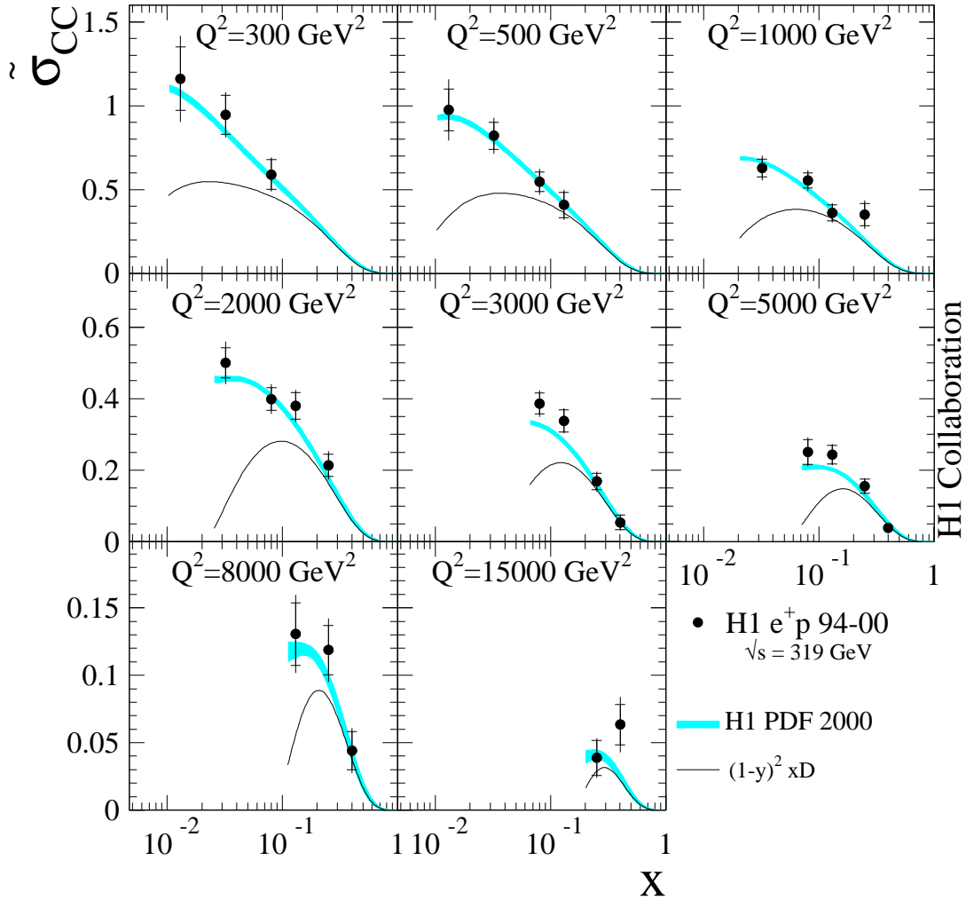
Figure 13: The CC reduced cross section \tilde{\sigma}_{CC}(x, Q^2) , shown for the combined 94 – 00 e^+p data (solid points). The results are compared with the corresponding Standard Model expectation (error bands) determined from the H1 PDF 2000 fit at \sqrt{s} = 319 GeV. The full curves indicate the expected xD contributions. The error bars and bands are defined as for fig. 5.
