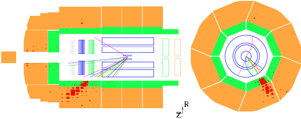
Figure 4.1: The CC event event in the H1 detector shows large deposition of energy in the LAr calorimeter characteristic to CC events. Since the neutrino escapes undetected this energy is unbalanced.
