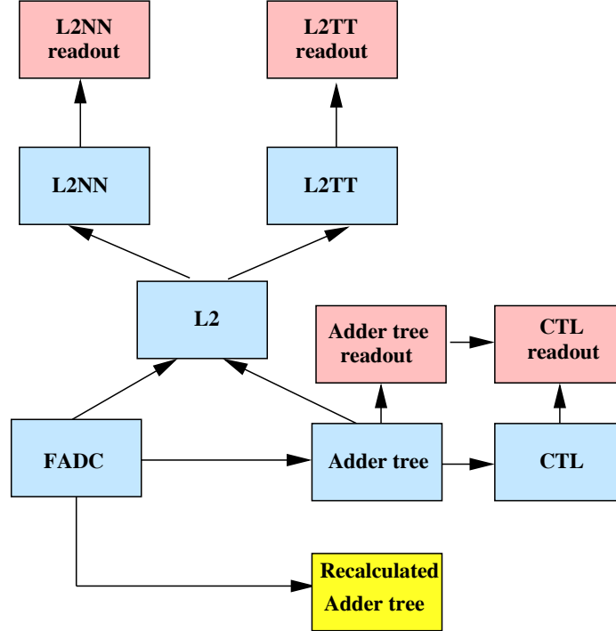
Figure A.1: A schematic view of the data stream from the LAr trigger.
