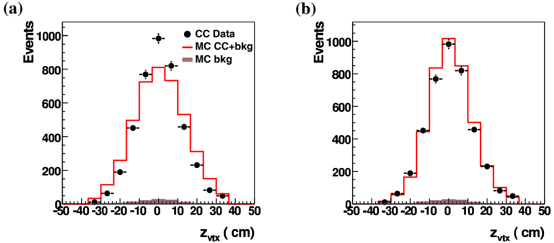
Figure 5.2: The vertex distribution for data and MC before (a) and after reweighting of MC (b). The reweighting factors applied to the MC have been done for the four different data periods.
