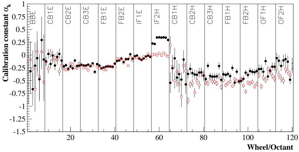
Figure 5.2: Calibration constants for the LAr calorimeter for data of the Shifted vertex period (closed points) and DJANGO MC (open points). Each wheel is labelled according to its position with respect to the nominal interaction point (central (CB), forward (IF,OF), Backward (B) see also Fig. 2.9). The lines indicate the octants of the corresponding wheels of the LAr calorimeter.
