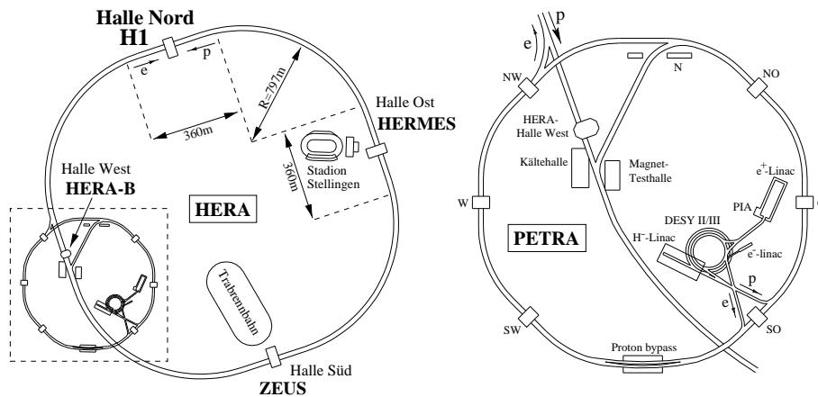
Figure 2.1: Schematic view of HERA (left) and the preaccelerator system (b)
