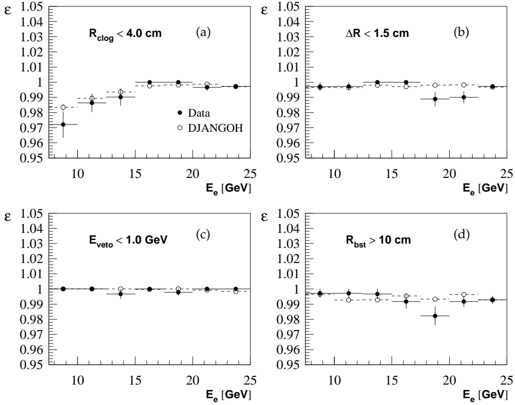
Figure 3.7: Efficiency of the electron identification cuts as function of the energy of the scattered electron E_e . (a) R_{clog} < 4 cm (b) \Delta R < 1.5 cm (c) E_{veto} < 1 GeV and (d) R_{BST} > 10 cm cut. The efficiency is derived using tagged-ISR events. Close points are Data and open circles are the signal DJANGO MC simulation.
