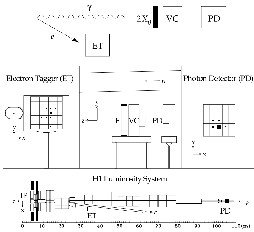
Figure 2.10: Luminosity system [39, 58].
