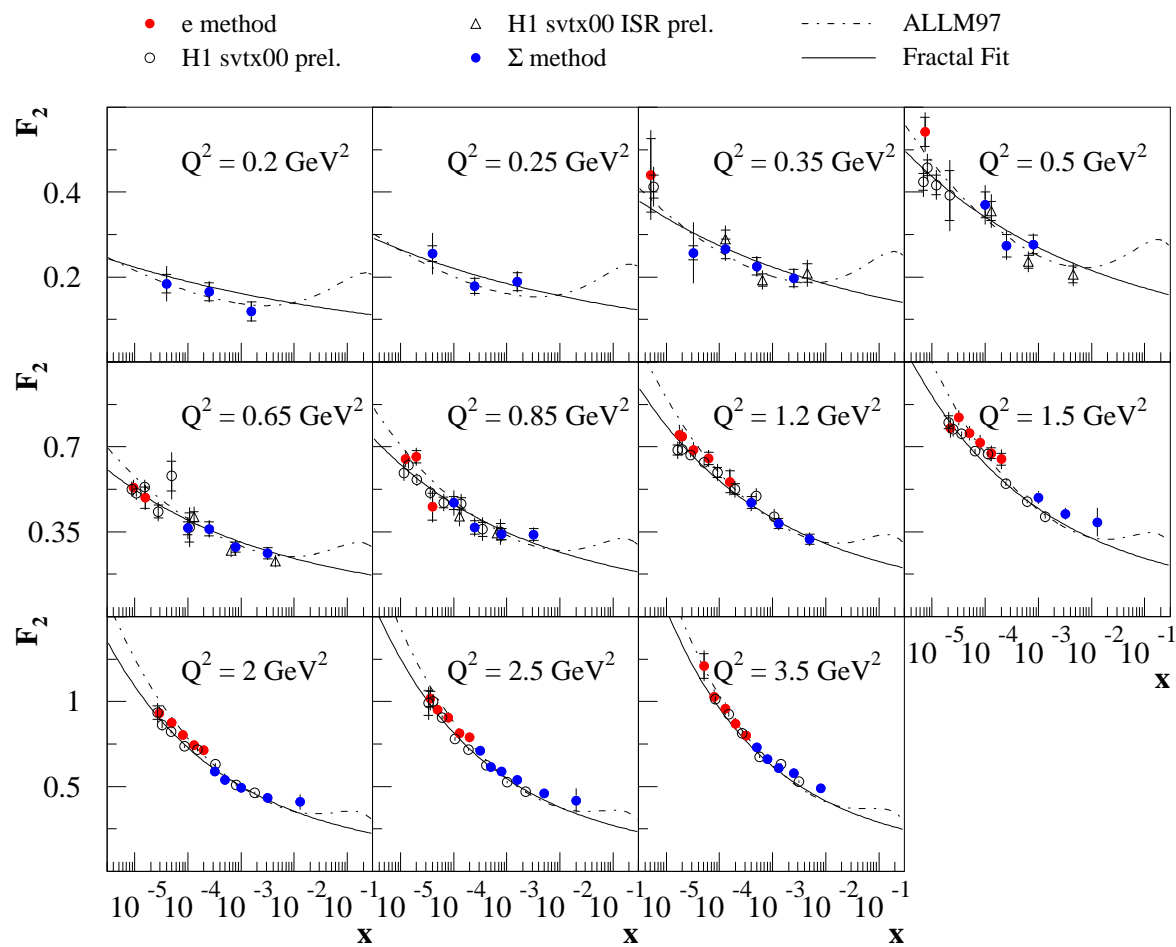
Figure 6.21: Comparison between the measurement of the proton structure function F_2 of the present analysis and the preliminary performed in [105] (open points). The dashed line correspond to the ALLM97 fit, while the full line is the expectation from the Fractal fit.
