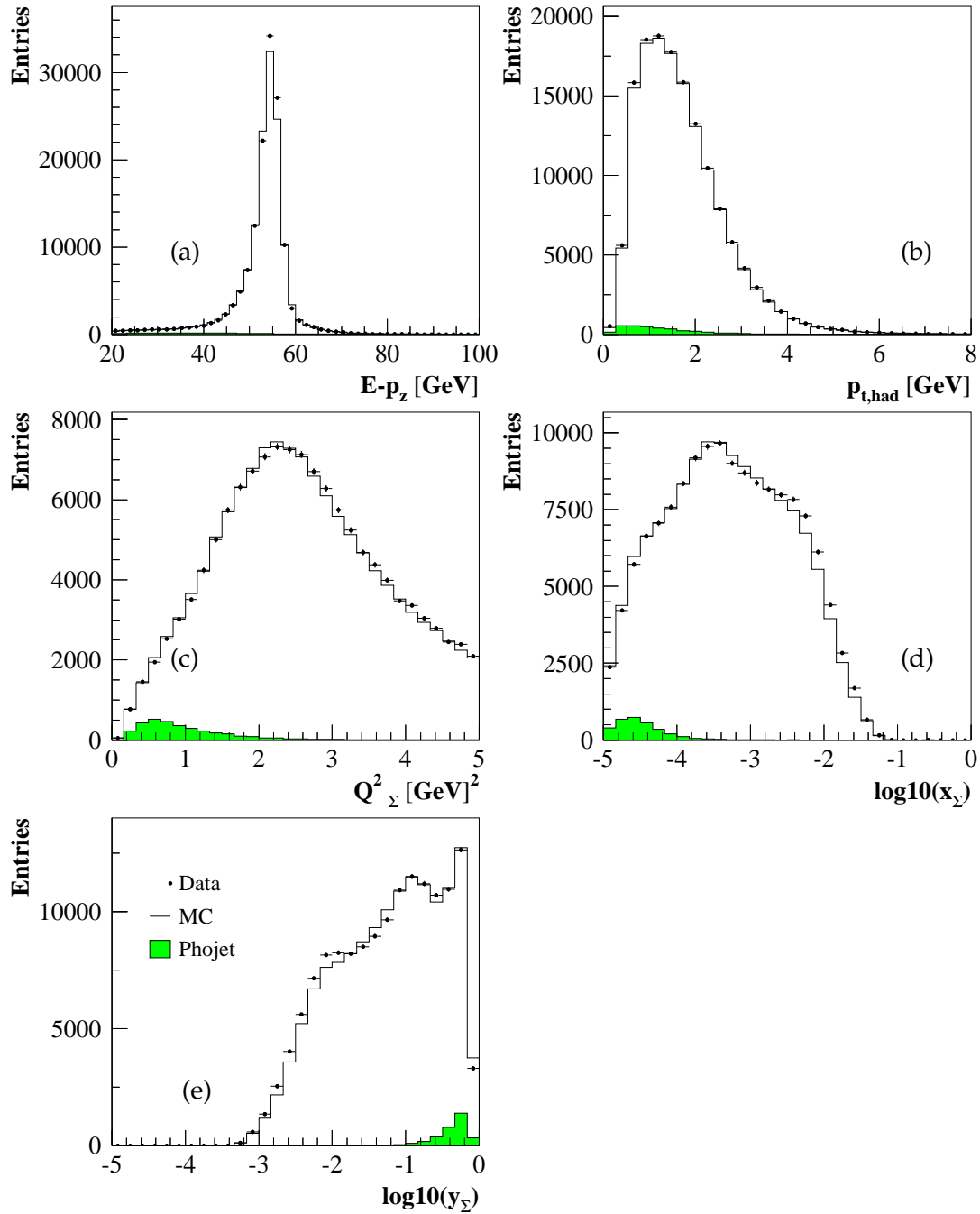
Figure 6.12: Control distributions of (a) E - p_z (b) the transvers momentum of the hadrons p_{t,had} . The kinematical variables (c) Q^2 (d) x_{\Sigma} and (e) y_{\Sigma} reconstructed with the \Sigma method. The MC simulation is normalized to the luminosity of the data +5% (see text)
