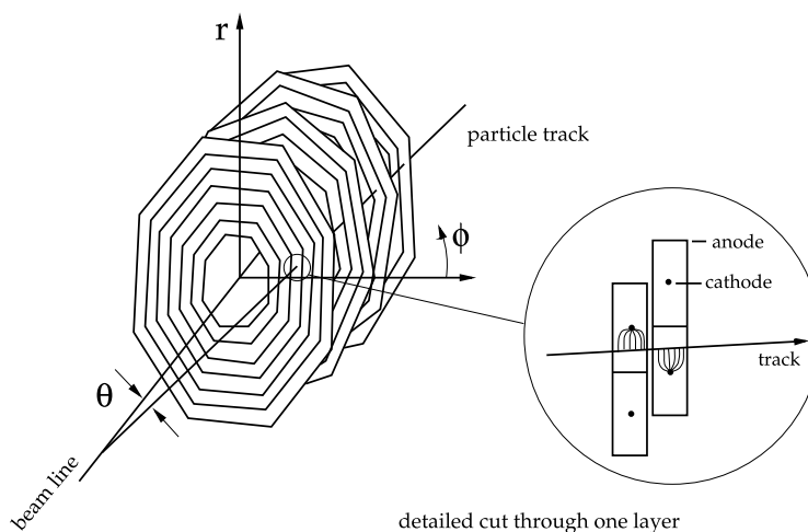
Figure 2.5: Schematic drawing of the Backward Drift Chamber [52].
