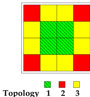
Figure 4.5: Schematic view of one module of the SpaCal calorimeter. Cells in the middle, corner and border define the topology 1,2 and 3, respectively.
