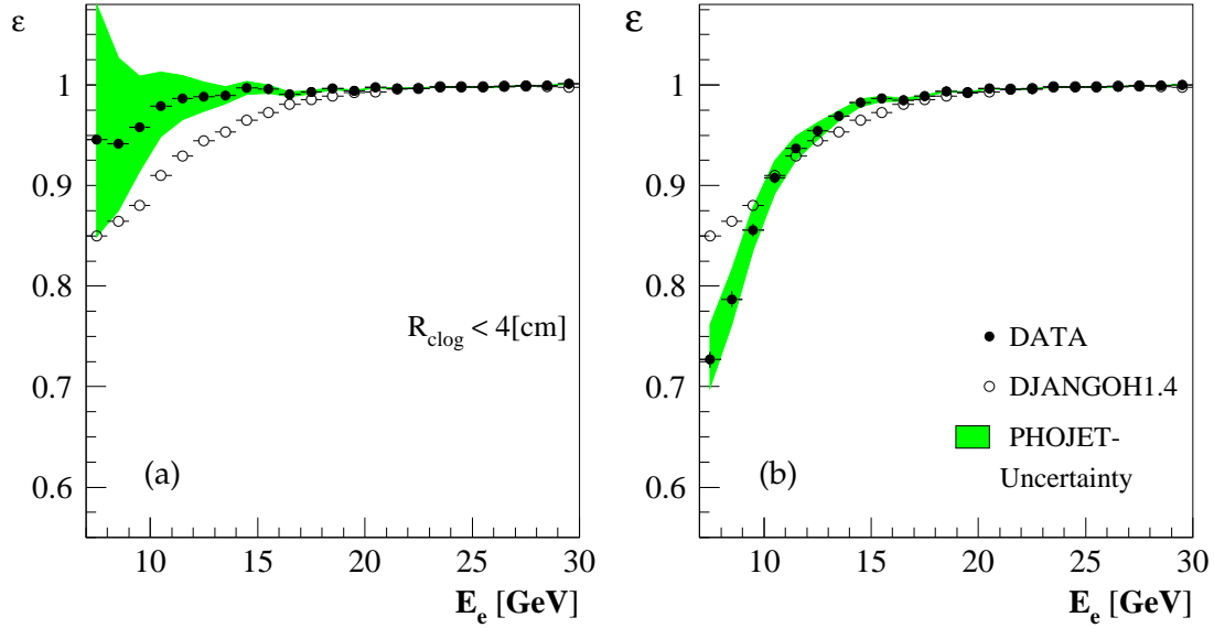
Figure 6.2: Efficiency of the R_{clog} < 4 cm cut as function of the energy of the scattered electron E_e . The open points shows the efficiency of the signal MC DJANGO1.4, while full points is data where the \gamma p is subtracted using the MC PHOJET. (a) The \gamma p background is subtracted from the data using the same normalization factor for R_{clog} < 4 cm and R_{clog} > 4 cm. (b) Same as Fig. (a), but using different normalization factors for accepted and rejected events (see text). Thus, for Fig. (b) the \gamma p background is subtracted considering the relative contribution of \gamma p to the data with R_{clog} < 4 cm and R_{clog} > 4 cm.
