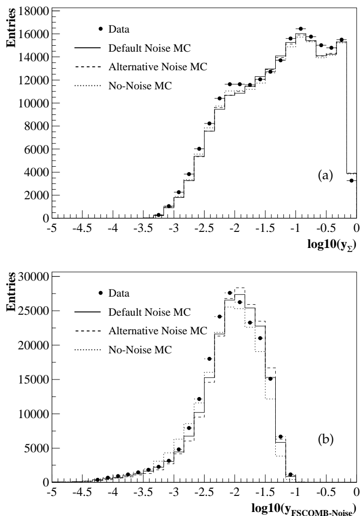
Figure 5.11: (a) Comparison between data and the different MC simulations of the y_{\Sigma} distributions of the DIS sample. (b) Comparison between data and MC for the mean value in y of the noise identified by the FSCOMB algorithm.
