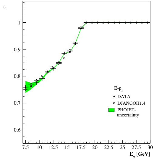
Figure 6.7: Efficiency of the (E - p_z)_{tot} > 35 GeV cut as function of the energy of the scattered electron E_e . Open points is the efficiency of DJANGO1.4 MC while closed points are data where the \gamma p background is subtracted using PHOJET.
