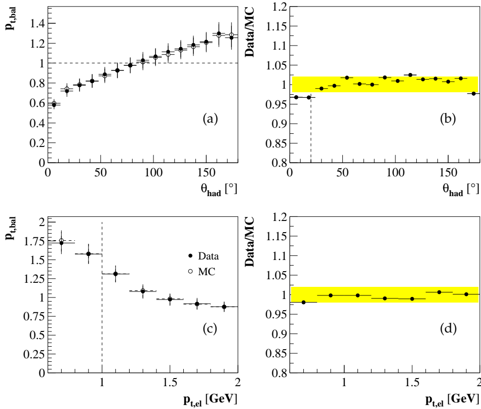
Figure 5.5: Comparison between data and MC for the p_{t,bal} distribution as function of (a) the hadronic angle \theta_{had} , (c) the transverse momentum of the electron p_{t,el} . The ratio of data over MC of Fig (a) and (c) are shown in Fig. (b) and (d). The ratio of data and MC has a drawn band corresponding to a deviation of 2%.
