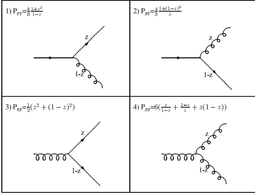
Figure 1.4: Splitting functions
