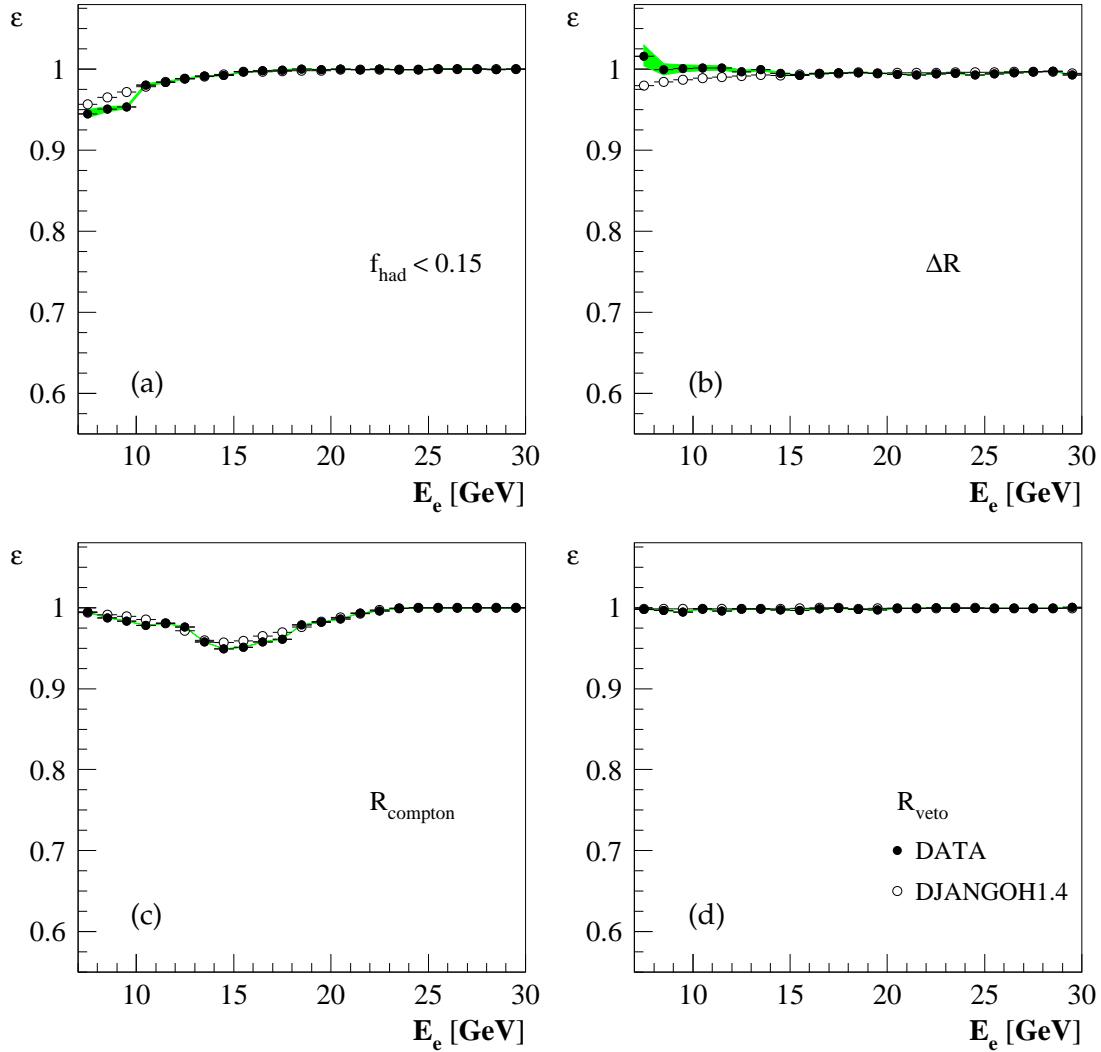
Figure 6.3: Efficiency of the selection cuts as function of the energy of the scattered electron E_e (a) the f_{had} < 0.15 cut (b) the SpaCal-BST matching \Delta R < 1.5 cm (c) the Compton rejection R_{compton} cut and (d) the R_{veto} cut. The open points shows the efficiency of the signal MC DJANGO1.4, while full points is data where the \gamma p is subtracted using the MC PHOJET.
