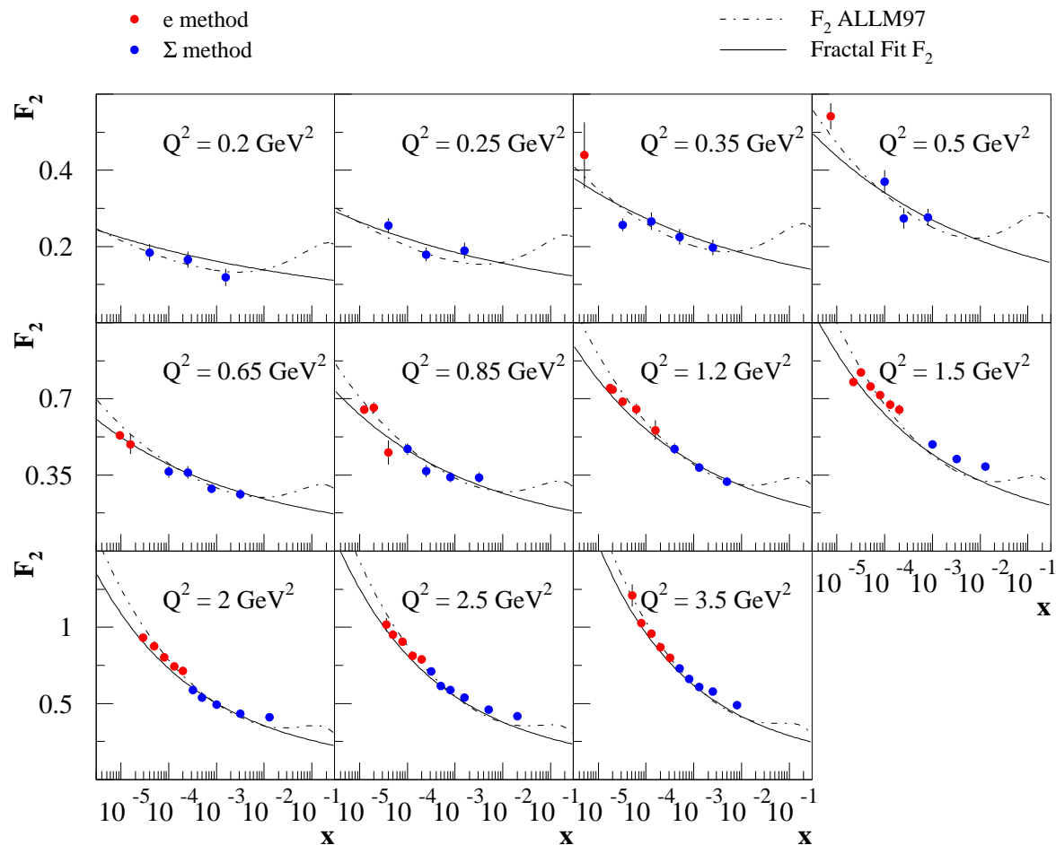
Figure 6.18: The proton structure function F_2 as function of x for different Q^2 values. The dashed line correspond to the ALLM97 fit [33], while the full line is the expectation from the Fractal fit [36]
