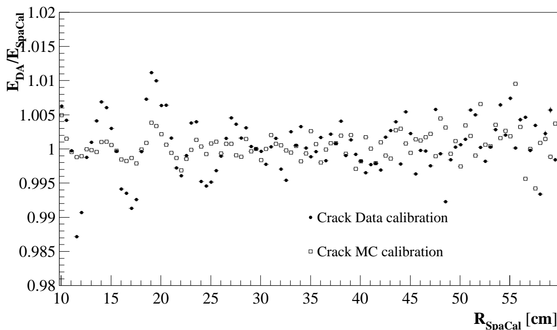
Figure 4.7: E_{DA}/E_{SpaCal} distribution using the gains, inbox and crack calibration factors as function of R_{SpaCal} .
