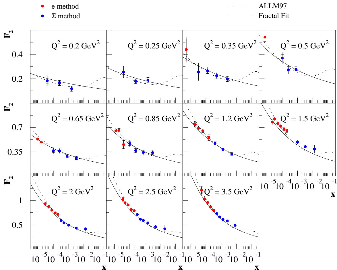
Figure 6.20: The proton structure function F_2 as function of x for different Q^2 values. The inner error bars correspond to the statistical uncertainty while the outer error bars show the total error obtaining by adding statistical and systematical uncertainties in quadrature. The dashed line correspond to the ALLM97 fit, while the full line is the expectation from the Fractal fit.
