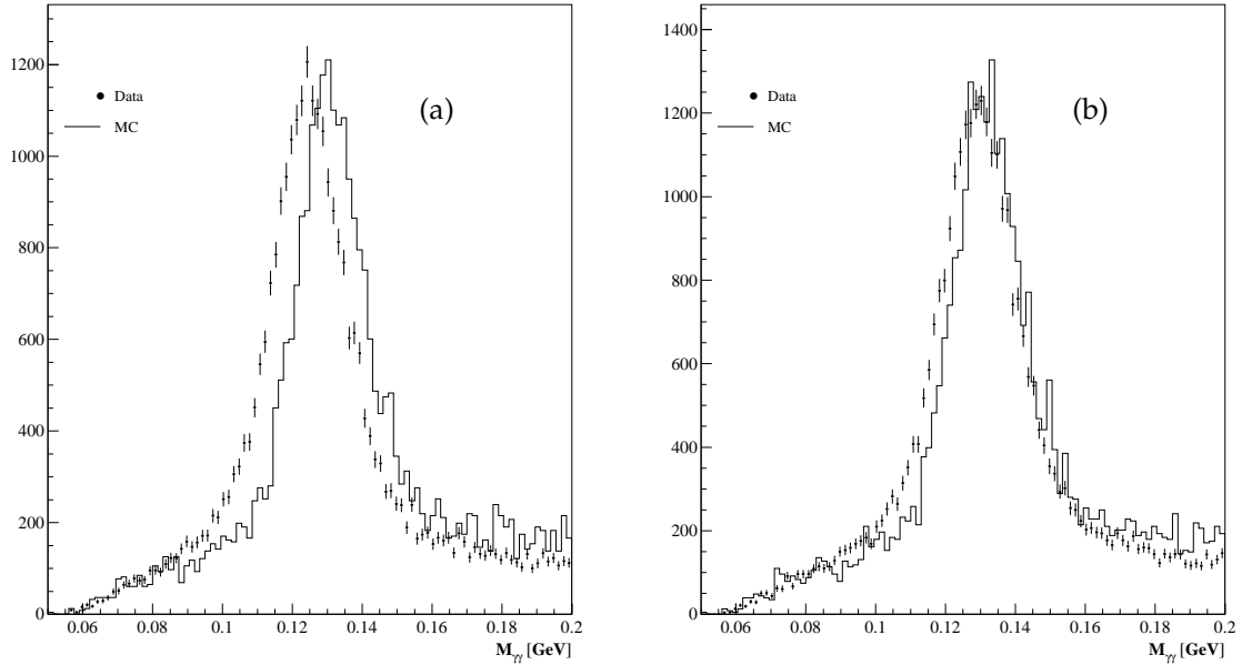
Figure 4.12: Invariant mass of \pi^0 invariant mass for energy clusters measured by SpaCal before (a) and (b) after applying the DA calibration.
