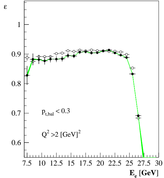
Figure 6.6: Efficiency of the p_{t,bal} < 0.3 cut using only events with Q_{\Sigma}^2 > 2 \text{ GeV}^2 . Open points show the efficiency of the signal MC DJANGO, while full points is data where the \gamma p is subtracted using PHOJET.
