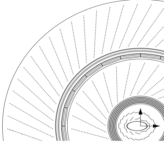
Figure 4.2: Transverse section of the Central Tracking Detector.
