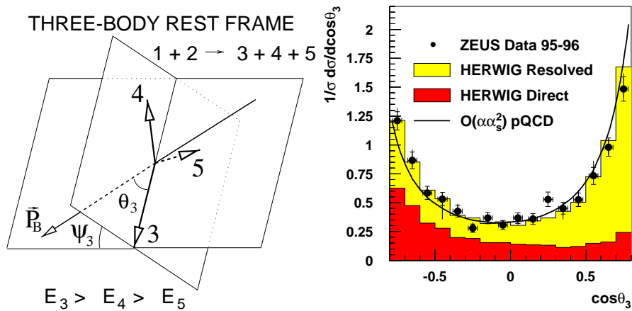
Figure 3. The definition and distribution of \cos(\theta_3) for three jet events in photoproduction measured by ZEUS. In addition to the data, the breakdown of the HERWIG Monte Carlo into direct and resolved component and the theory prediction is shown.
