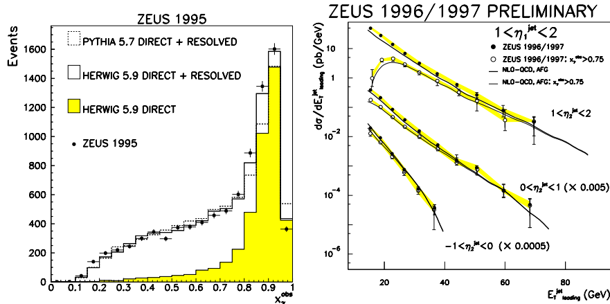
Figure 4. x_\gamma^{obs} spectrum and single differential cross section for dijet events in photoproduction measured at ZEUS compared to Monte Carlo and NLO pQCD predictions. The leading (second) jet is required to have a transverse energy greater than 14(11) GeV.
