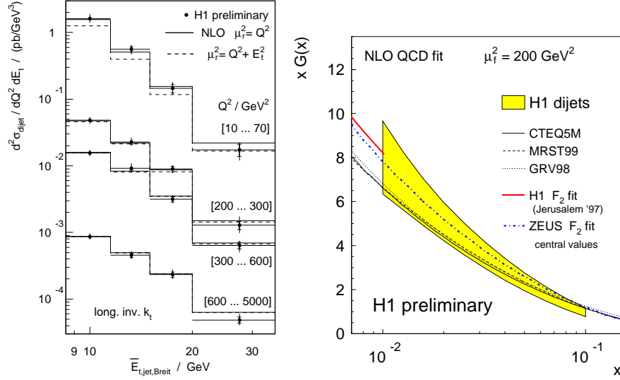
Figure 2. H1 double differential cross sections for dijet production in DIS. The data are compared to NLO predictions. The gluon density, extracted from the dijet distributions, is also shown.
