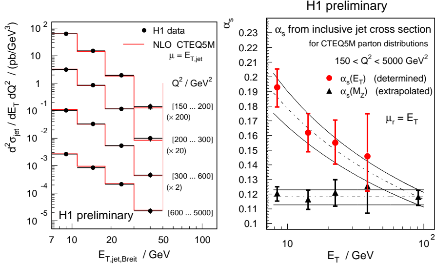
Figure 1. H1 double differential cross sections for inclusive jet production in DIS. The data are compared to NLO predictions. The strong coupling strength \alpha_s , extracted from the inclusive jet distributions, is also shown.
