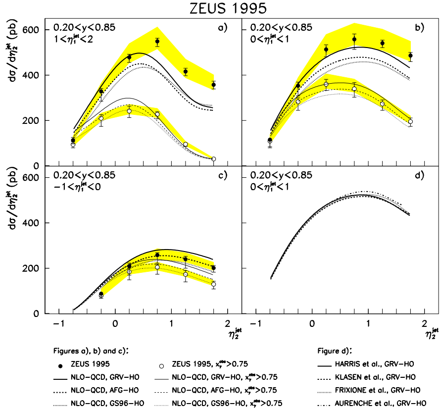
Figure 5. a)-c) Dijet cross section as function of jet rapidity for different x_\gamma^{\text{obs}} ranges compared to NLO pQCD predictions using various photon structure functions. The thick band shows the systematic uncertainty; d) Comparison of different NLO pQCD calculations for one choice of photon structure function.
