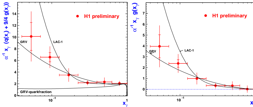
Figure 6. Effective photon structure function (left) and gluon density (right) in the photon as extracted from H1 dijet data for photoproduction. For comparison the LAC-1 and the GRV parameterizations are shown.
