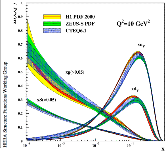
Parton densities
