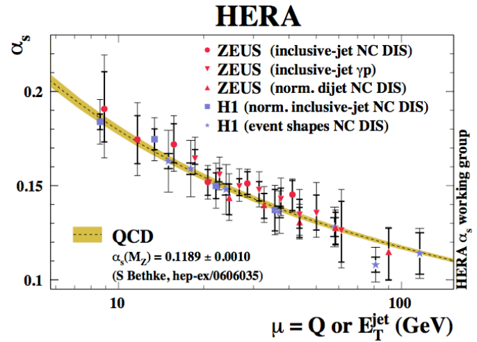
Strong coupling
