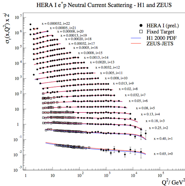
Structure functions
