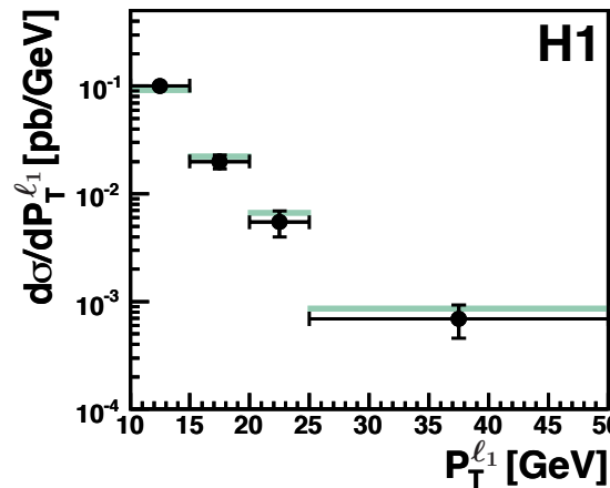
Multi-Leptons at HERA (463 pb -1 )
