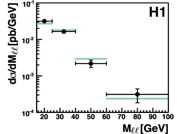
Multi-Leptons at HERA (463 pb -1 )
