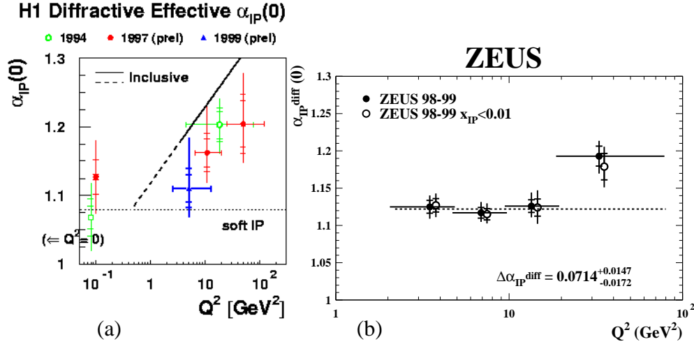
FIGURE 3. Q^2 dependence of the Pomeron intercept \alpha_{\mathbb{P}}(0) , measured by H1 (a) and by ZEUS (b).
