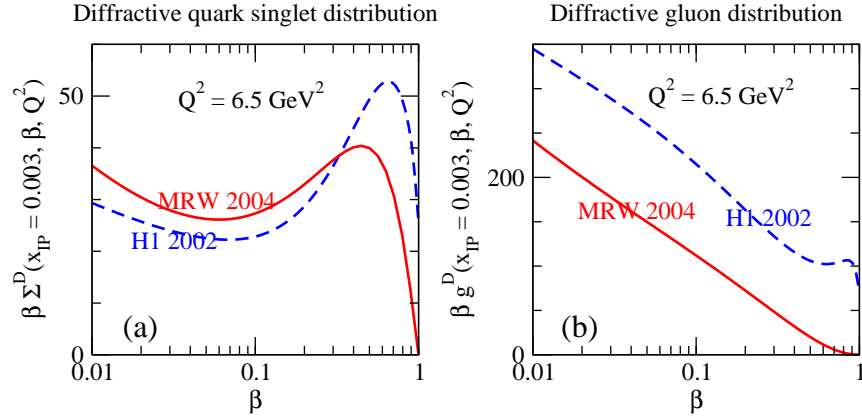
FIGURE 6. The diffractive parton densities resulting from a combined QCD fit by A. Martin et al. [13] to the ZEUS proton tagged, ZEUS M_X and H1 LRG data. The dashed lines are the densities obtained in the H1 fit 2002 [5].
