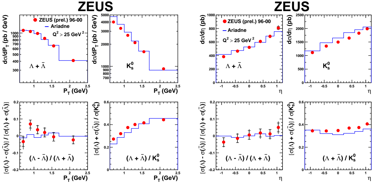
FIGURE 2. \Lambda and K_S^0 cross sections, \frac{\Lambda - \bar{\Lambda}}{\Lambda + \bar{\Lambda}} ratio and \frac{\Lambda + \bar{\Lambda}}{K_S^0} ratio as a function of P_T and \eta
