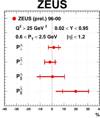
FIGURE 1. Transverse and longitudinal \Lambda and \bar{\Lambda} polarization.
