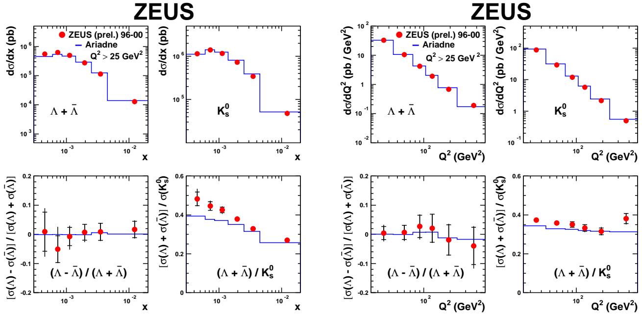
FIGURE 3. \Lambda and K_s^0 cross sections, \frac{\Lambda - \bar{\Lambda}}{\Lambda + \bar{\Lambda}} ratio and \frac{\Lambda + \bar{\Lambda}}{K_s^0} ratio as a function of x and Q^2
