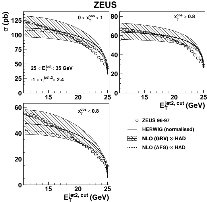
Fig. 8. Dependence of the two-jet cross section on E_T^{\text{jet2;cut}} from ZEUS [16].
