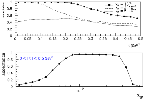
Figure 4. VFPS acceptances, as a function of t (top) and of x_{IP} (bottom).
