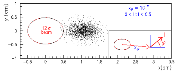
Figure 3. Spread of the impact point of diffractively scattered protons in the (x, y) plane for x_{IP} = 0.01 and 0 \leq |t| \leq 0.5 \text{ GeV}^2 , with the 12 \sigma beam envelope. Insert: Illustration of the relation between the impact point of the scattered proton in the transverse (x, y) plane and the variables x_{IP} , |t| and \phi .
