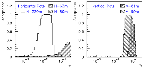
Figure 5. Acceptance as a function of x_{IP} for the VFPS and the present H1 spectrometer (horizontal and vertical stations, respectively).
