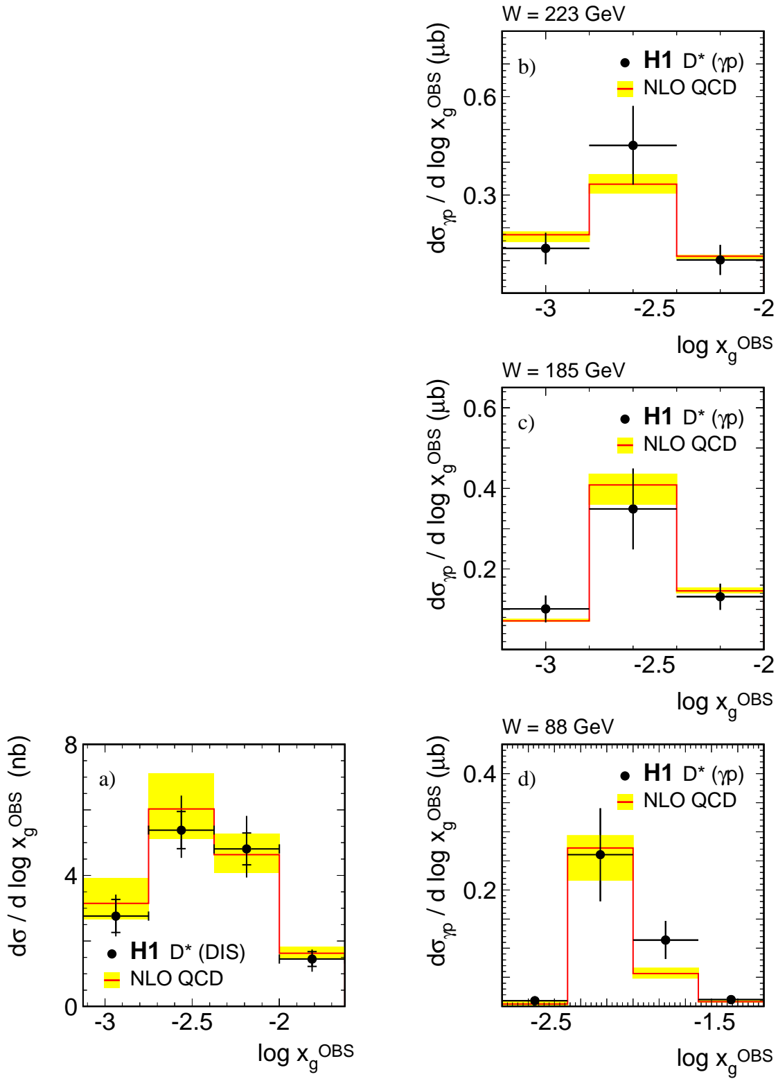
Figure 5: (a) Differential DIS cross section as a function of x_g^{OBS} in the kinematic range of experimental acceptance (see Tab. 1). Figures (b-d) show the corresponding photoproduction cross sections, separately for W_{\gamma p} = 223, 185 and 88 GeV, respectively. The meaning of the data points, histograms and their errors is the same as in Fig. 2 (for DIS) and Fig. 3 (for \gamma p ).
