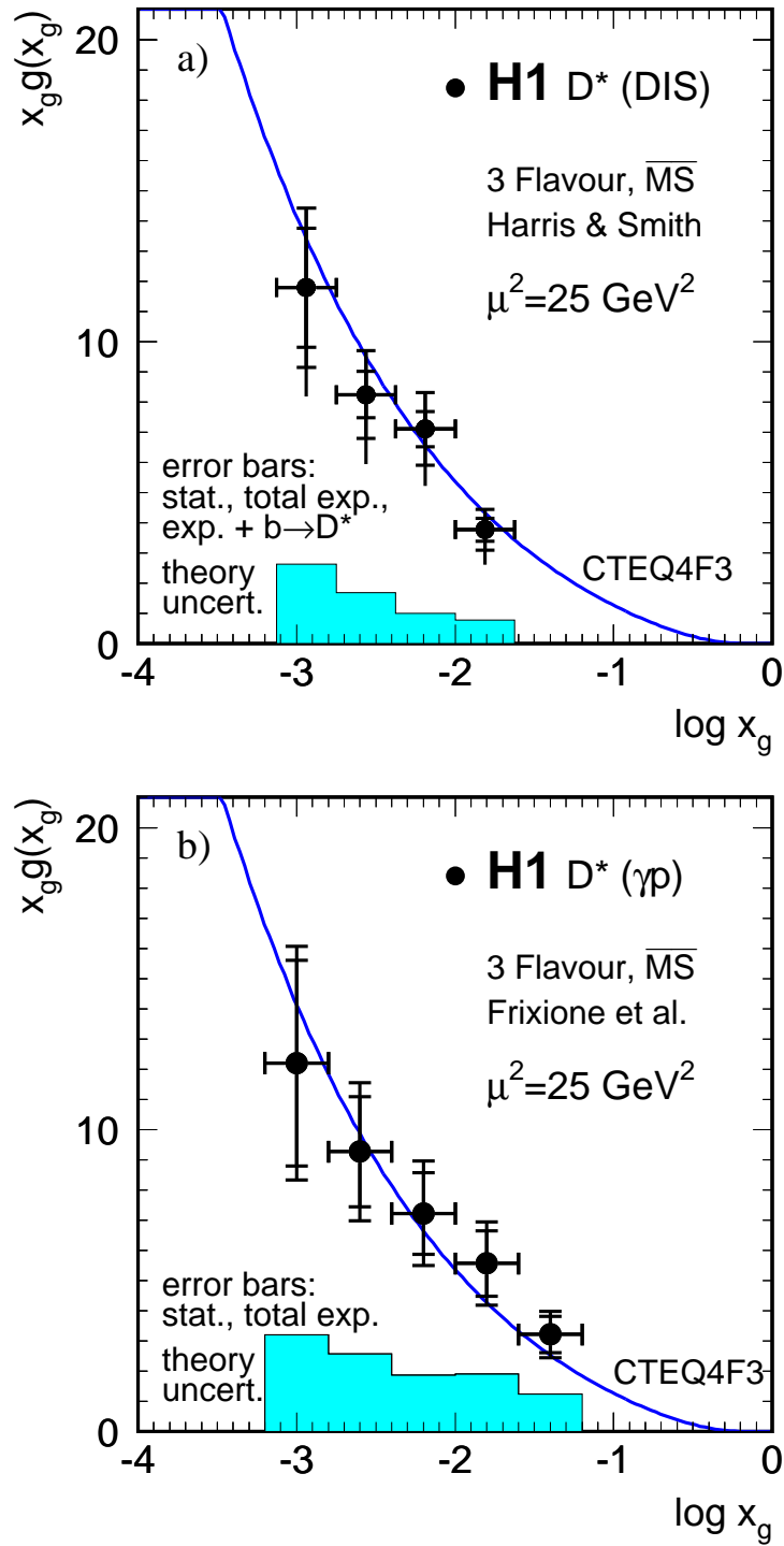
Figure 8: Gluon density, determined from DIS (a) and from from photoproduction data (b), compared to the CTEQ4F3 parameterization at \mu^2 = 25 \text{ GeV}^2 (full line). The error bars represent the statistical (inner) and total experimental (outer) error; in addition the effect of a subtraction of b\bar{b} background (if 5 times higher than predicted in a LO Monte Carlo program) is displayed in (a), in (b) the b\bar{b} contribution is negligible. The theoretical systematic error is shown as shaded band along the abscissa and is dominated in DIS (a) by the uncertainty associated with the charm quark mass, in photoproduction (b) it is dominated by the uncertainty associated with the renormalization and factorization scale.
