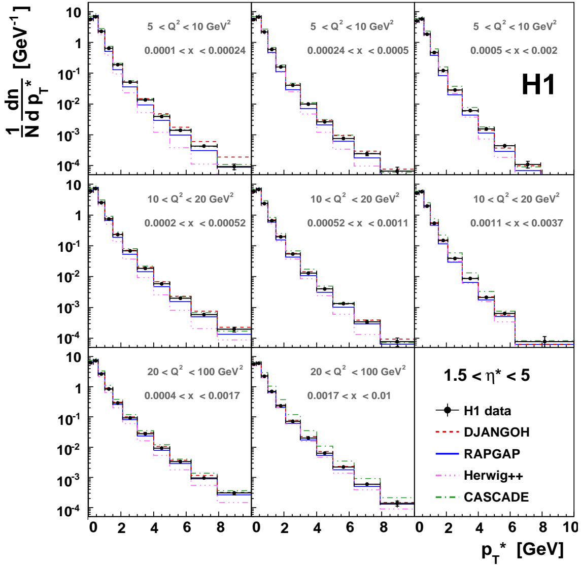
Figure 10: Charged particle density as a function of p_T^* in the range 1.5 < \eta^* < 5 for eight intervals of Q^2 and x compared to DJANGO, RAPGAP, Herwig++ and CASCADE Monte Carlo predictions.
