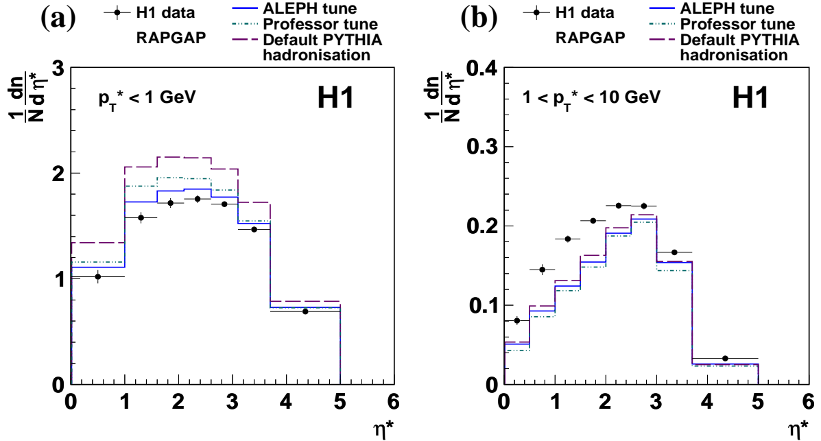
Figure 4: Charged particle density as a function of \eta^* for (a) p_T^* < 1 GeV for (b) 1 < p_T^* < 10 GeV compared to RAPGAP predictions for three different sets of fragmentation parameters. The predictions are obtained using CTEQ6L(LO) PDF.
