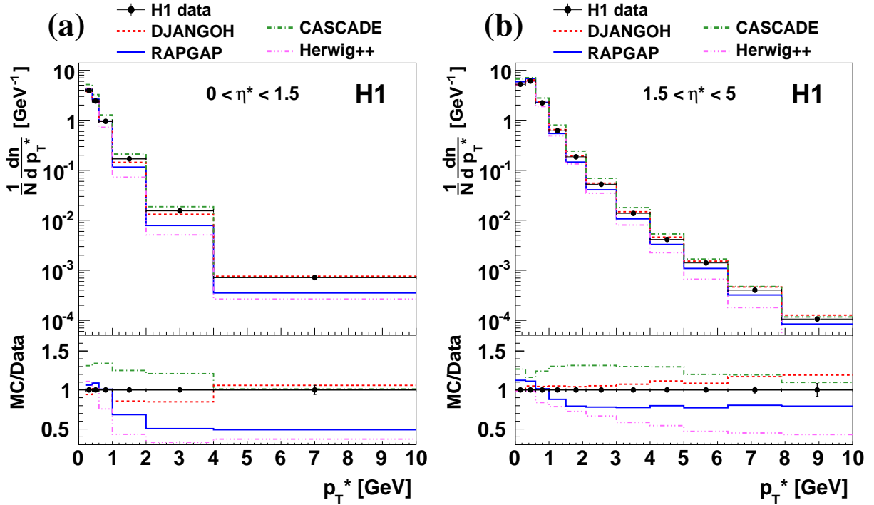
Figure 8: Charged particle density as a function of p_T^* in the ranges (a) 0 < \eta^* < 1.5 and (b) 1.5 < \eta^* < 5 compared to DJANGO, RAPGAP, Herwig++ and CASCADE Monte Carlo predictions. The ratios of MC predictions to the measurements are shown on the bottom of the figure.
