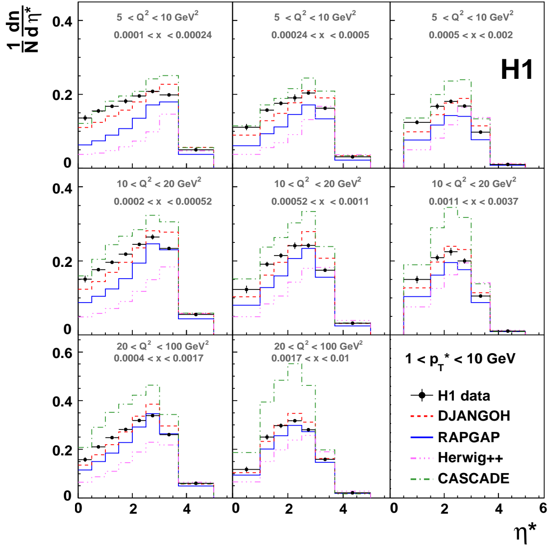
Figure 7: Charged particle density as a function of \eta^* for 1 < p_T^* < 10 GeV for eight intervals of Q^2 and x compared to DJANGO, RAPGAP, Herwig++ and CASCADE Monte Carlo predictions.
