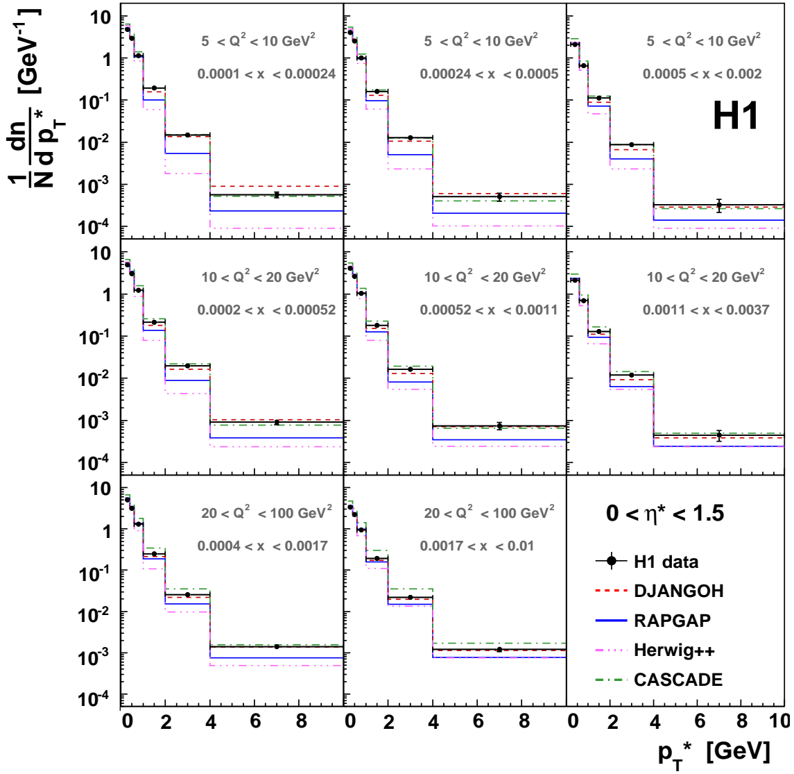
Figure 9: Charged particle density as a function of p_T^* in the range 0 < \eta^* < 1.5 for eight intervals of Q^2 and x compared to DJANGO, RAPGAP, Herwig++ and CASCADE Monte Carlo predictions.
