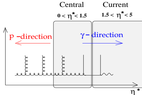
Figure 2: The two pseudorapidity regions analysed in this paper. The region 0 < \eta^* < 1.5 and 1.5 < \eta^* < 5 , are denoted as “central” and “current” regions, respectively.
