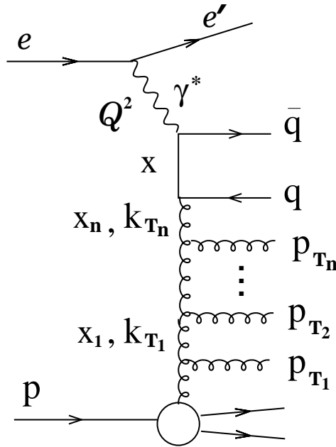
Figure 1: Generic diagram for deep-inelastic ep scattering at small x . The transverse momenta of the emitted gluons are labeled as p_{T,i} , while the proton longitudinal momentum fractions and the transverse momenta carried by the propagating gluons are denoted by x_i and k_{T,i} , respectively.
