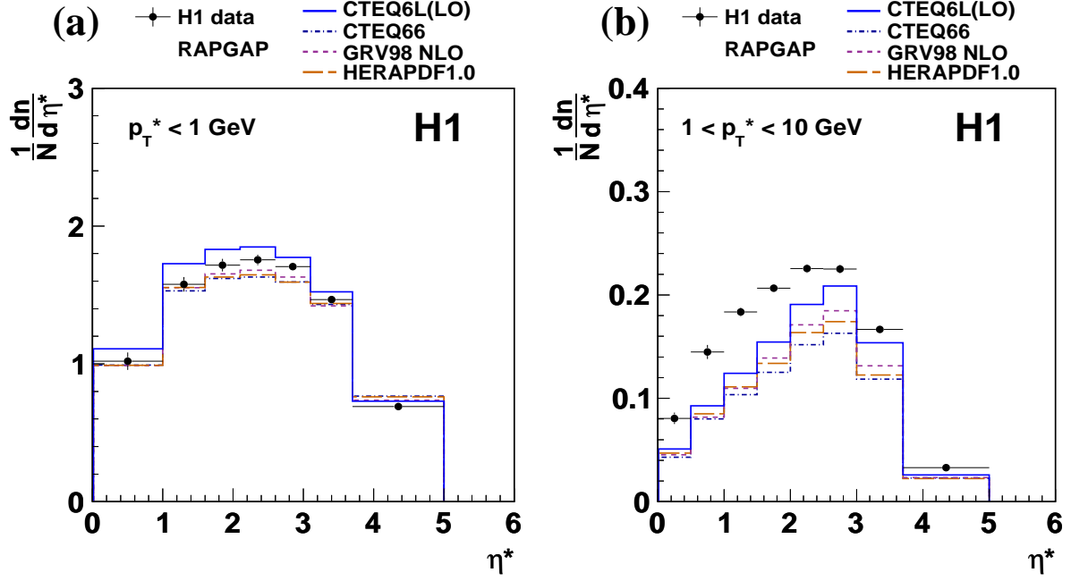
Figure 3: Charged particle density as a function of \eta^* for (a) p_T^* < 1 GeV and for (b) 1 < p_T^* < 10 GeV compared to RAPGAP predictions with different proton PDFs. The predictions are obtained using the ALEPH tune.
