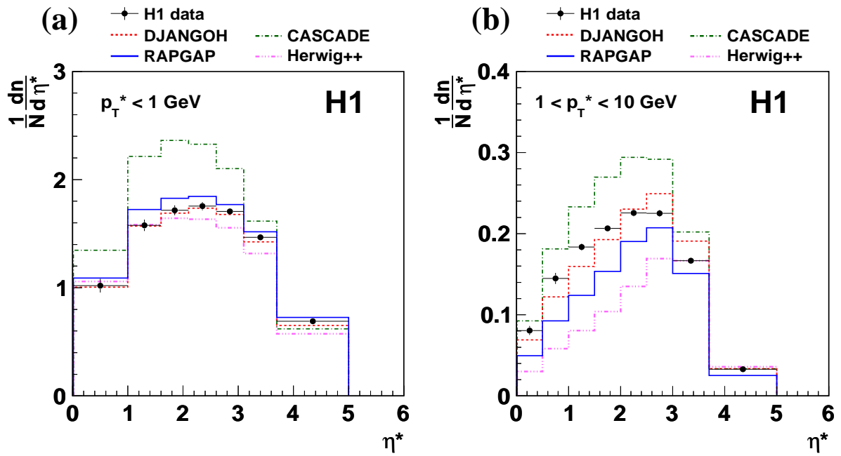
Figure 5: Charged particle density as a function of \eta^* for (a) p_T^* < 1 \text{ GeV} for (b) 1 < p_T^* < 10 \text{ GeV} compared to DJANGO, RAPGAP, Herwig++ and CASCADE Monte Carlo predictions.
