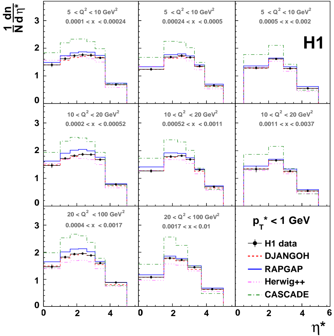
Figure 6: Charged particle density as a function of \eta^* for p_T^* < 1 GeV for eight intervals of Q^2 and x compared to DJANGO, RAPGAP, Herwig++ and CASCADE Monte Carlo predictions.
